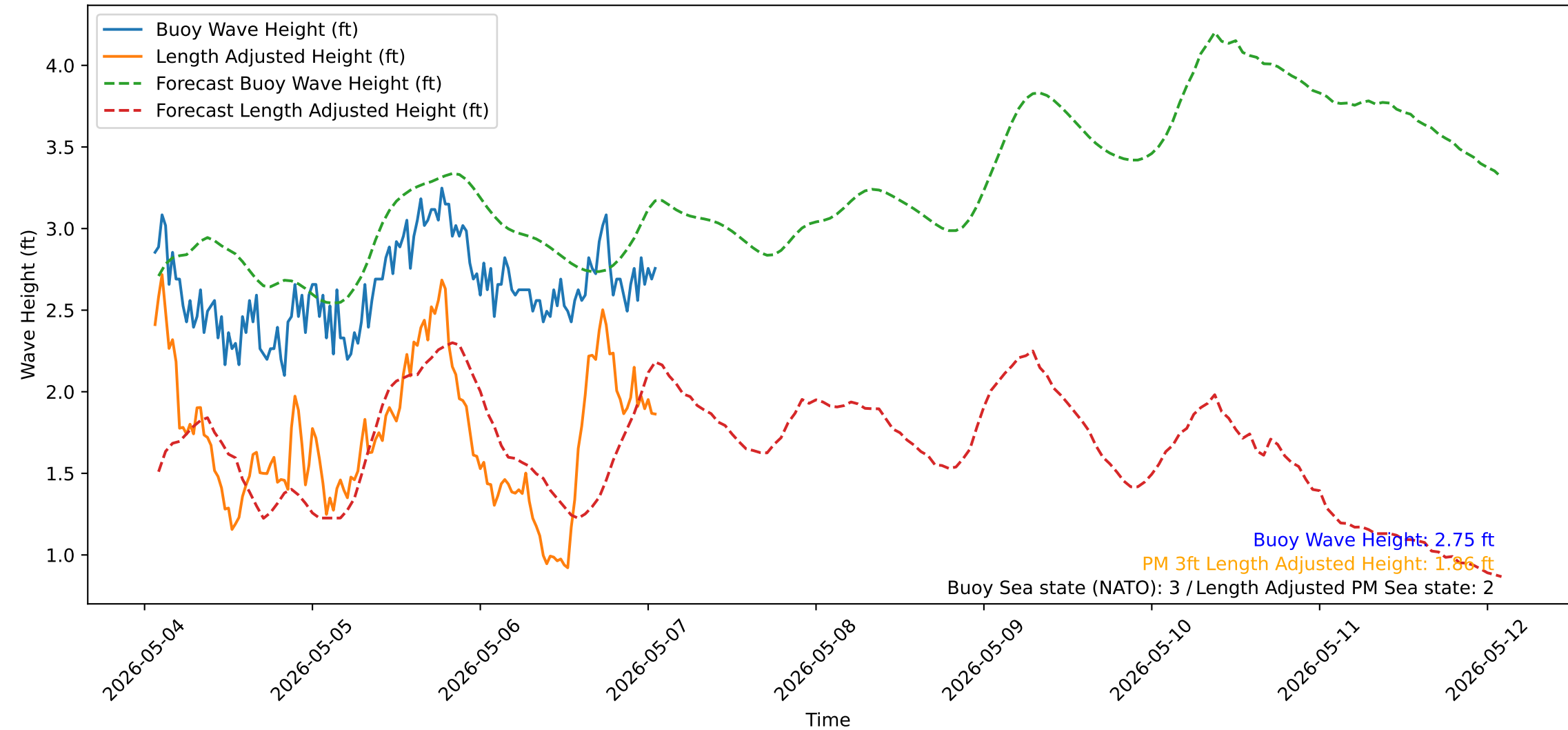
Wave Heights over Time for Oceanside Harbor at 2026-05-07 01:40:31
