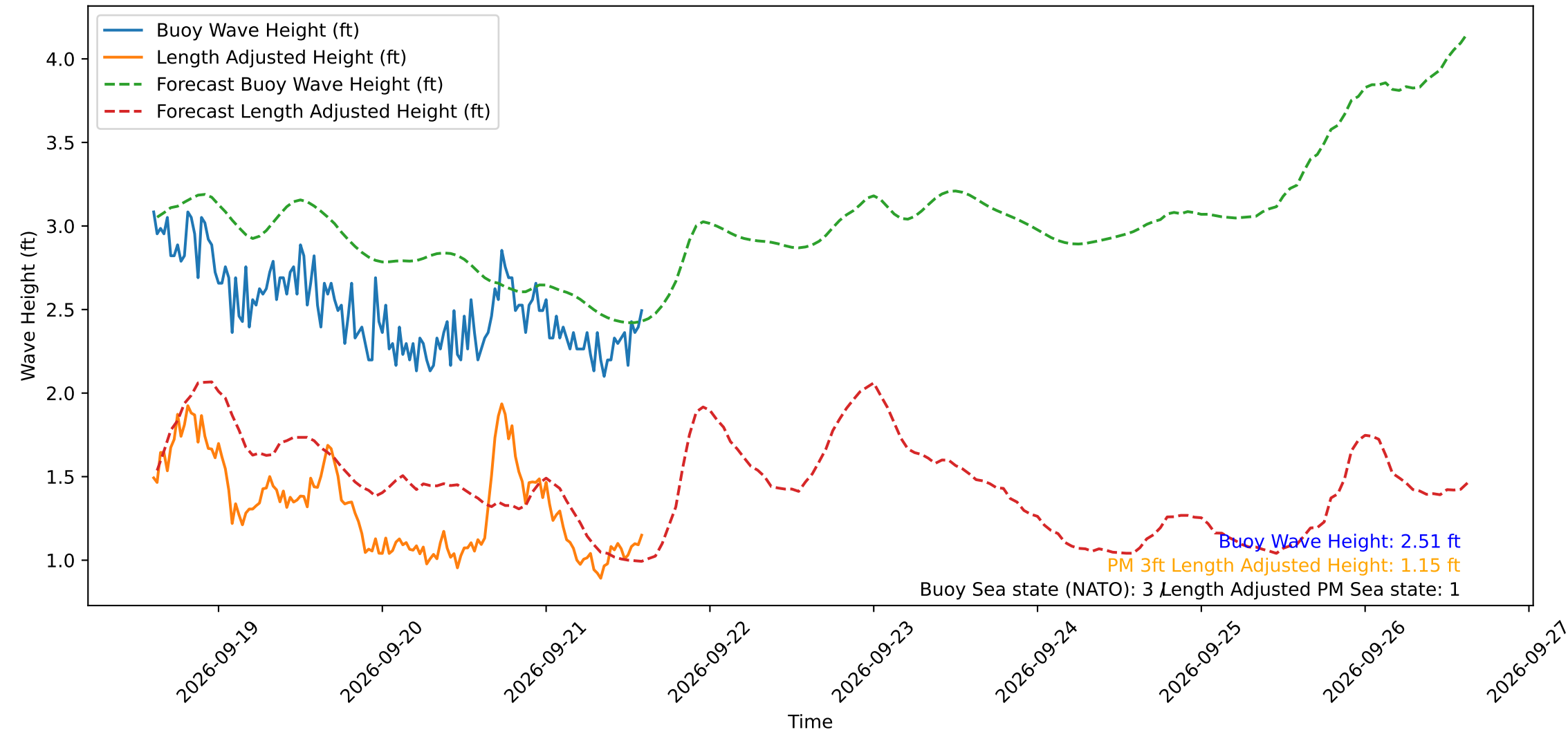
Wave Heights over Time for Oceanside Harbor at 2026-09-21 14:30:30
