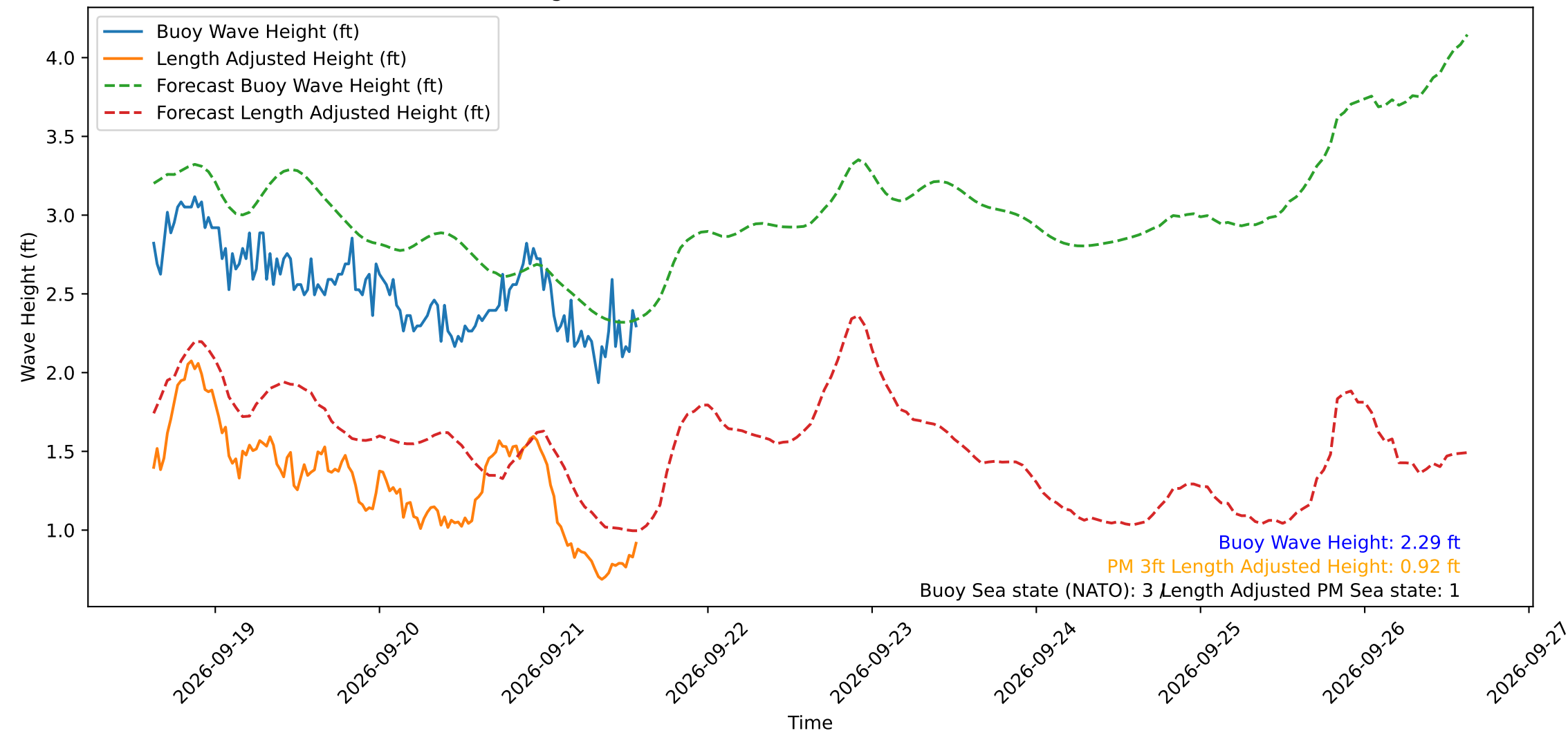
Wave Heights over Time for Green Beach at 2026-09-21 14:31:11
