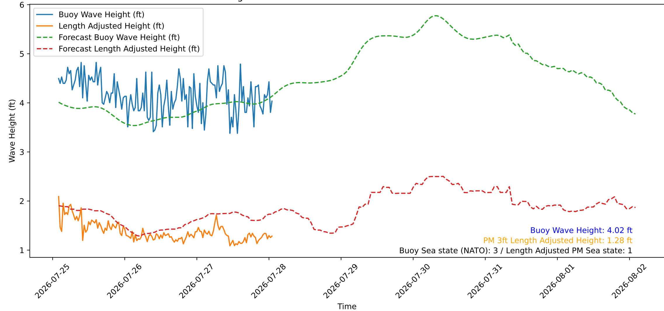
Wave Heights over Time for Green Beach at 2026-07-28 01:51:10
