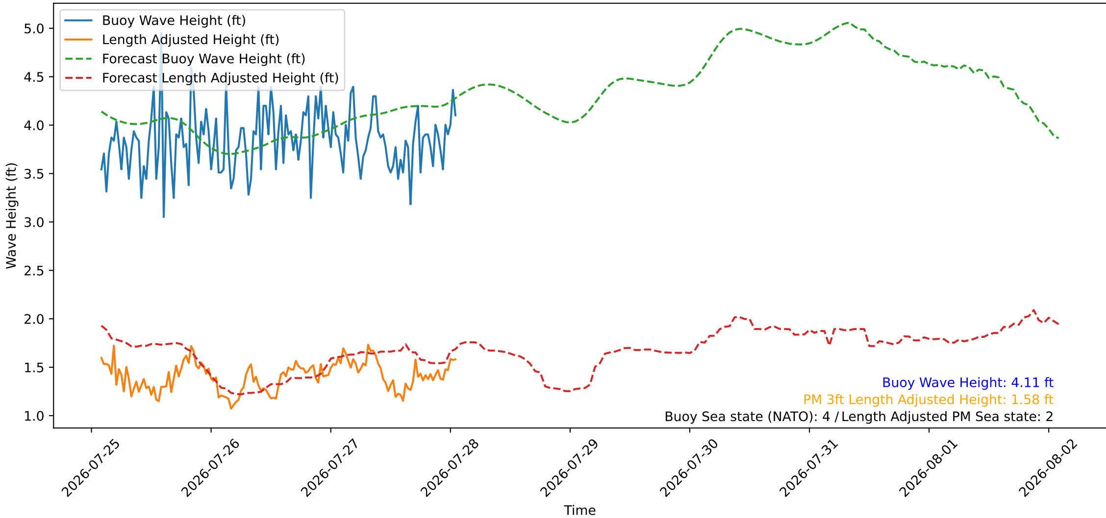
Wave Heights over Time for Oceanside Harbor at 2026-07-28 01:50:27
