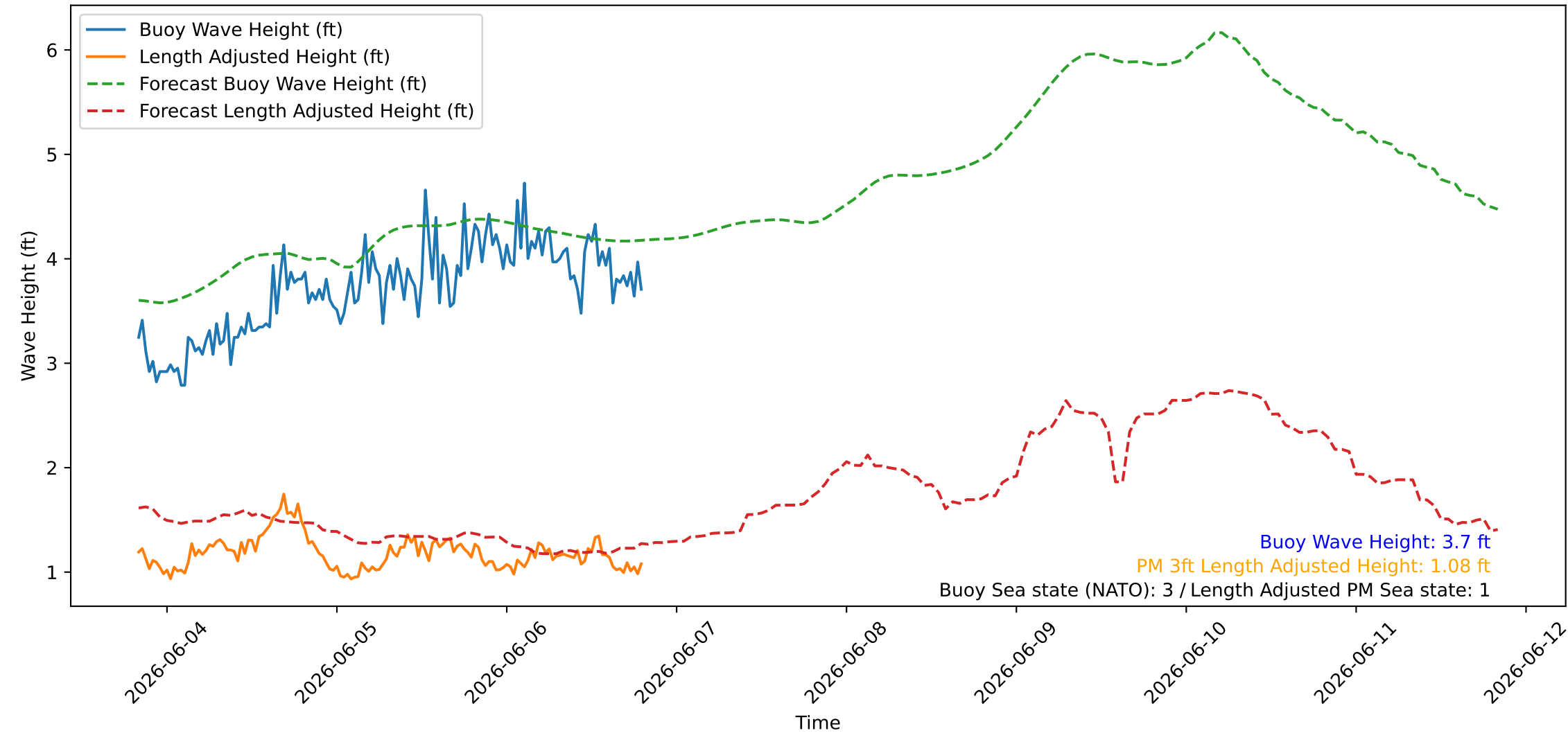
Wave Heights over Time for Green Beach at 2026-06-06 20:01:07
