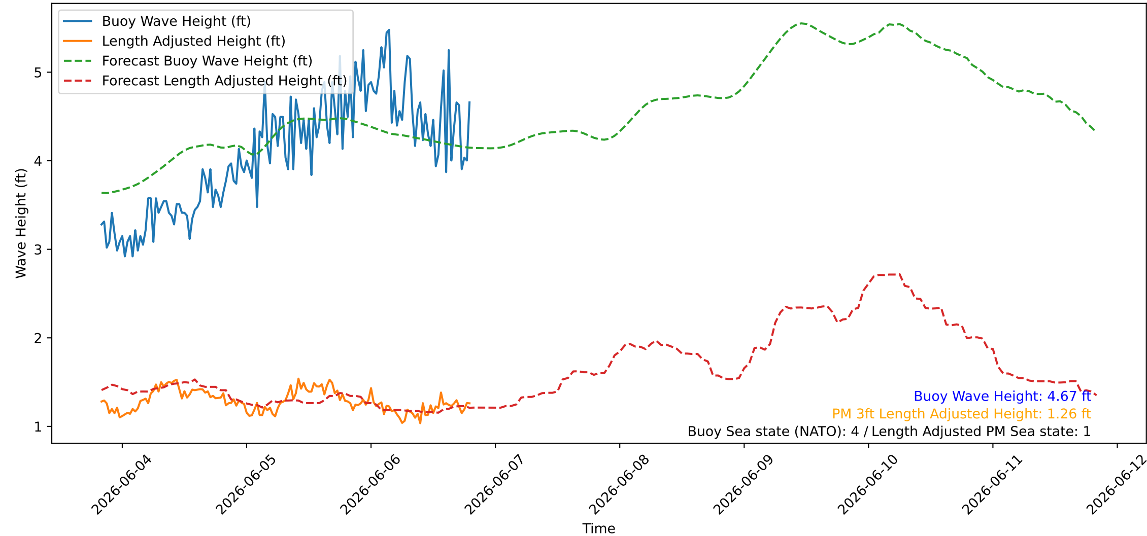
Wave Heights over Time for Oceanside Harbor at 2026-06-06 20:00:26
