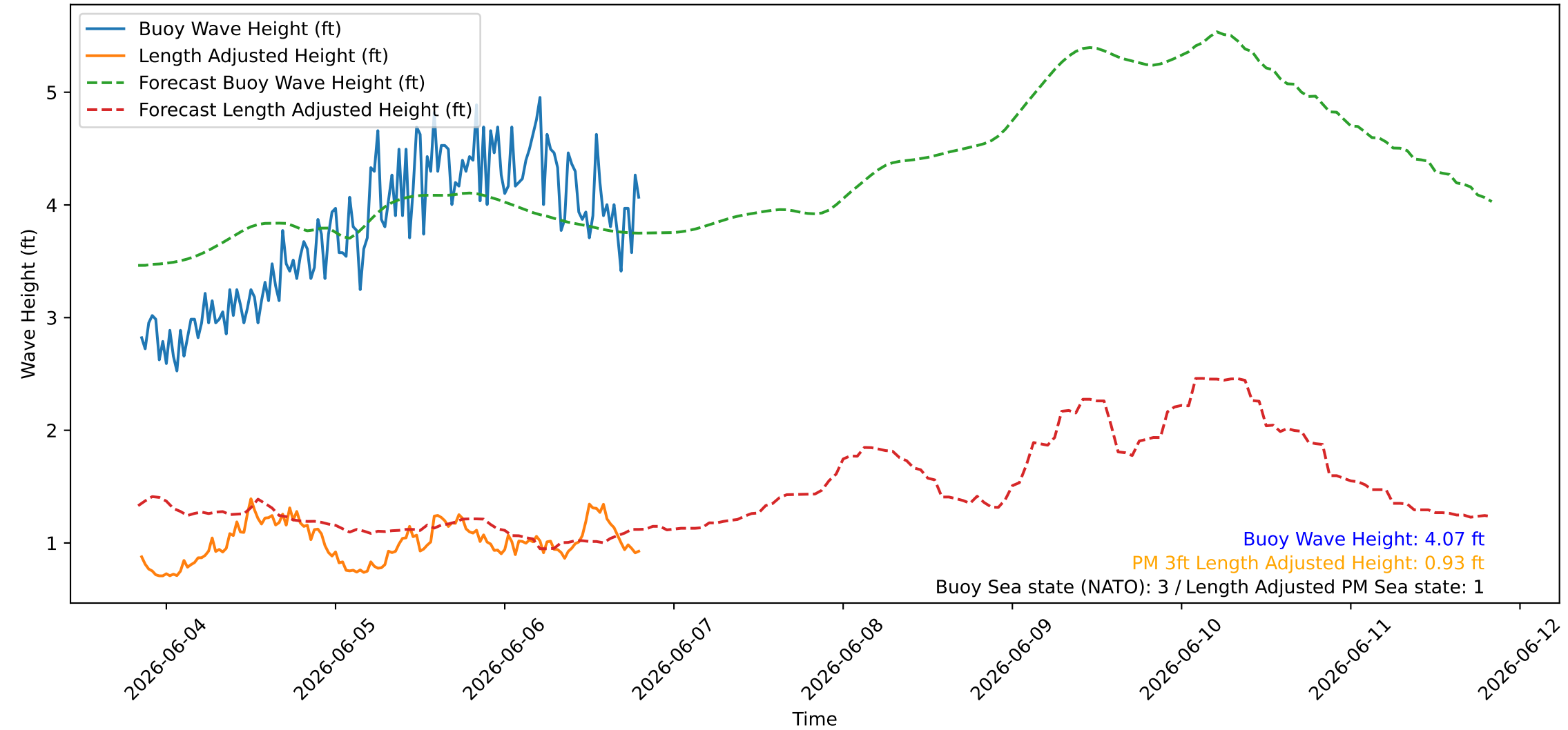
Wave Heights over Time for Red Beach at 2026-06-06 20:00:45
