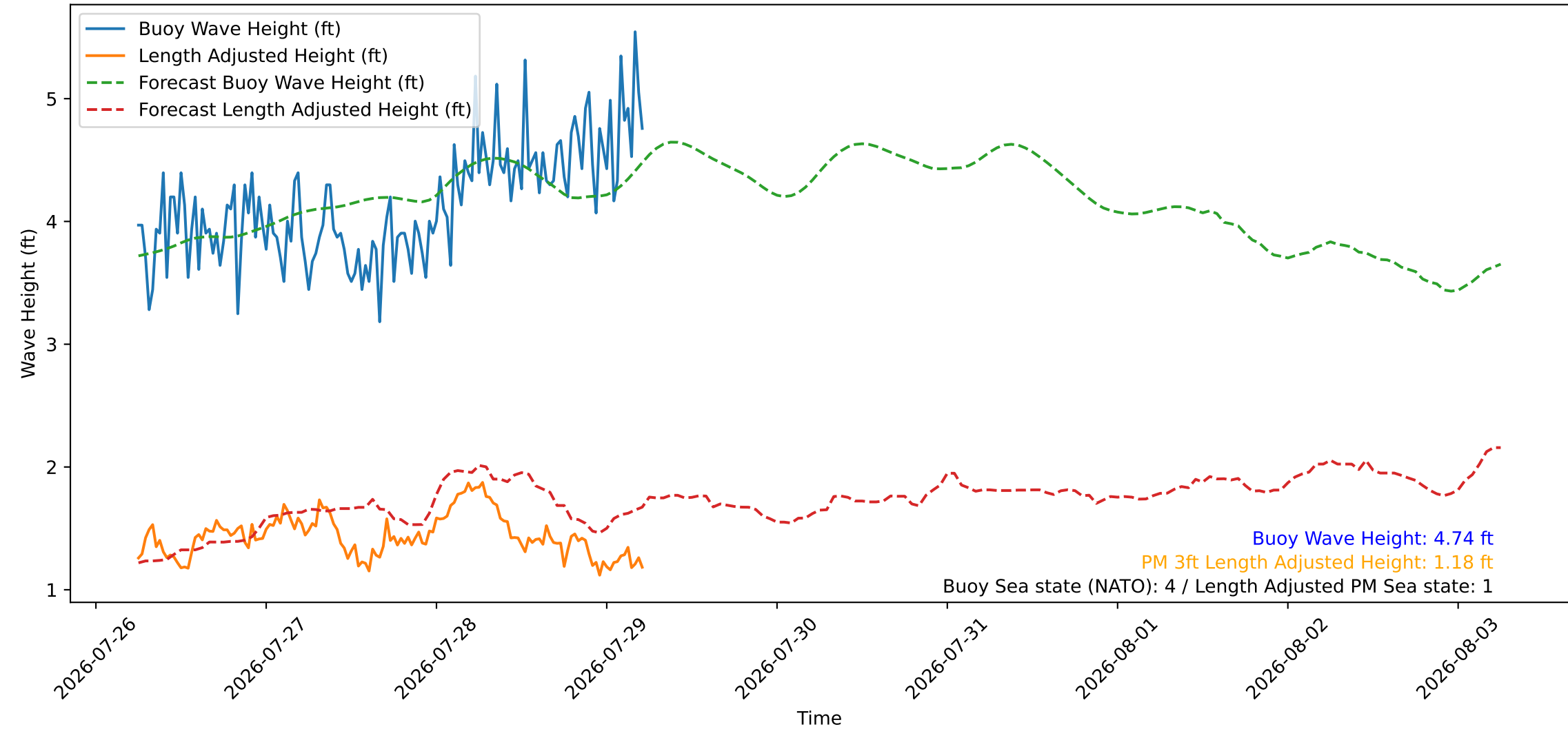
Wave Heights over Time for Oceanside Harbor at 2026-07-29 05:50:26
