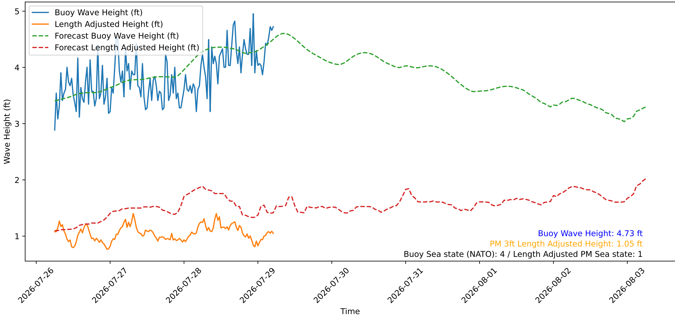
Wave Heights over Time for Red Beach at 2026-07-29 05:50:47
