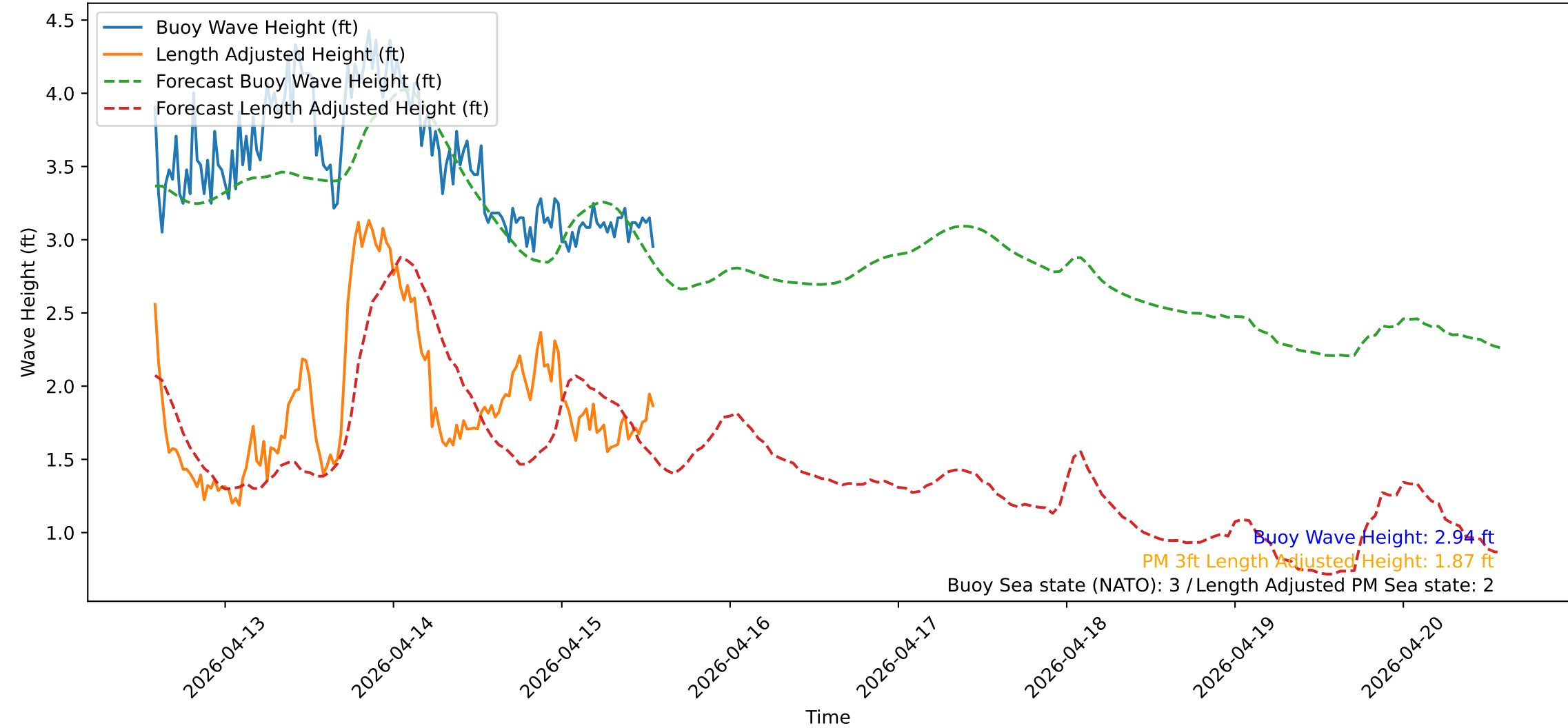
Wave Heights over Time for Red Beach at 2026-04-15 13:40:51
