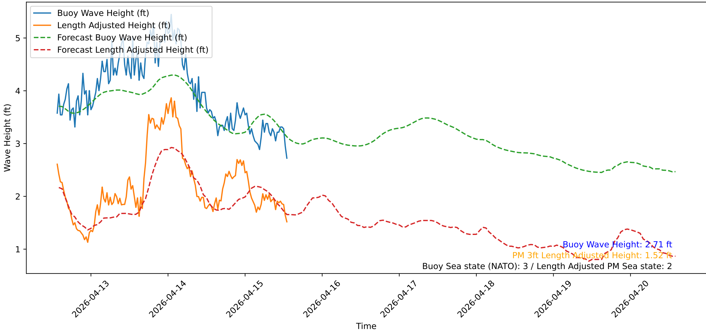
Wave Heights over Time for Oceanside Harbor at 2026-04-15 13:40:31
