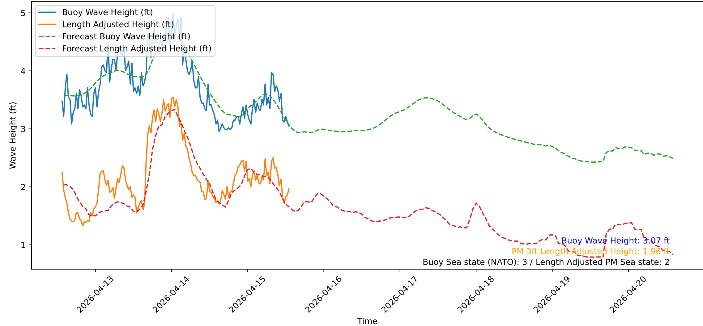
Wave Heights over Time for Green Beach at 2026-04-15 13:41:13
