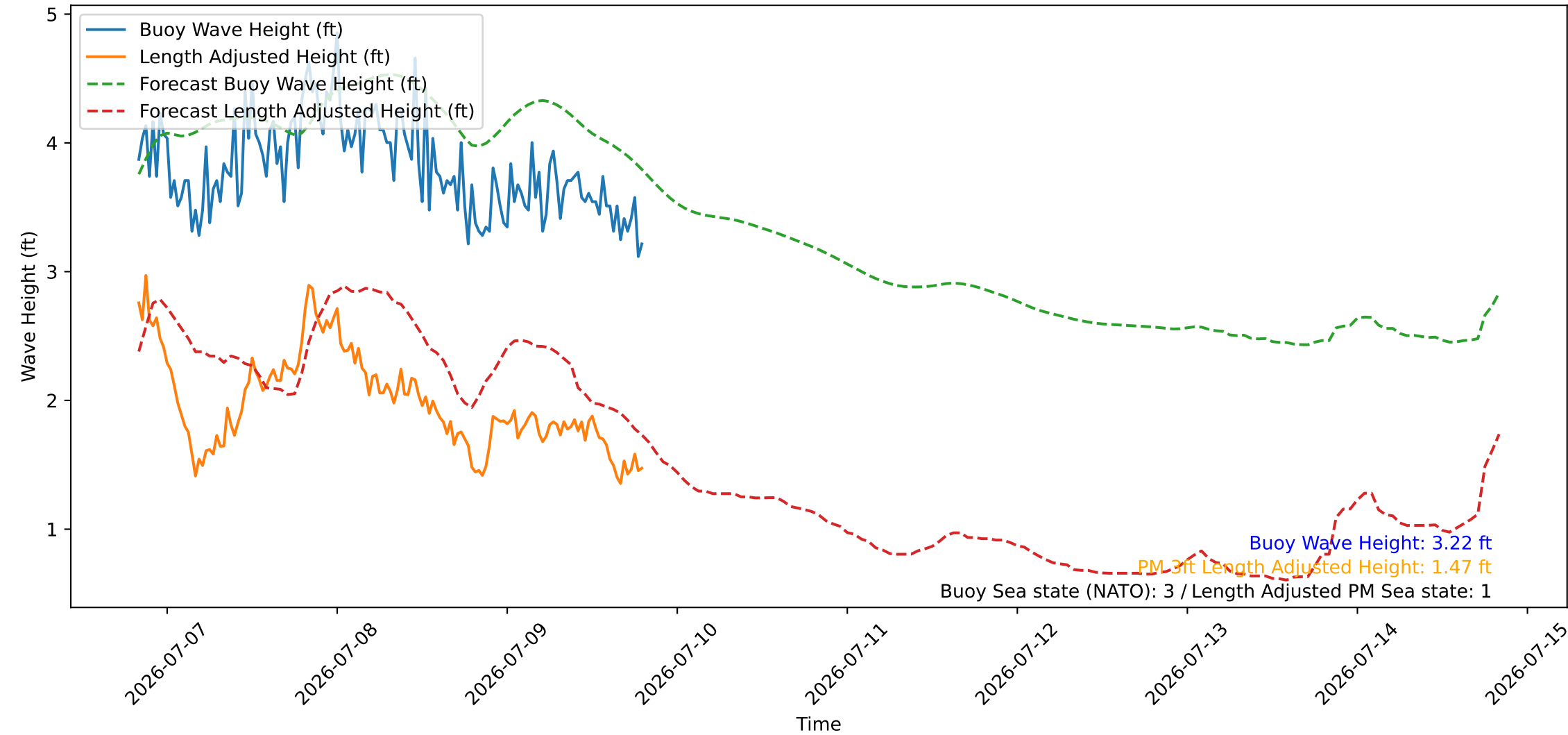
Wave Heights over Time for Red Beach at 2026-07-09 19:50:47
