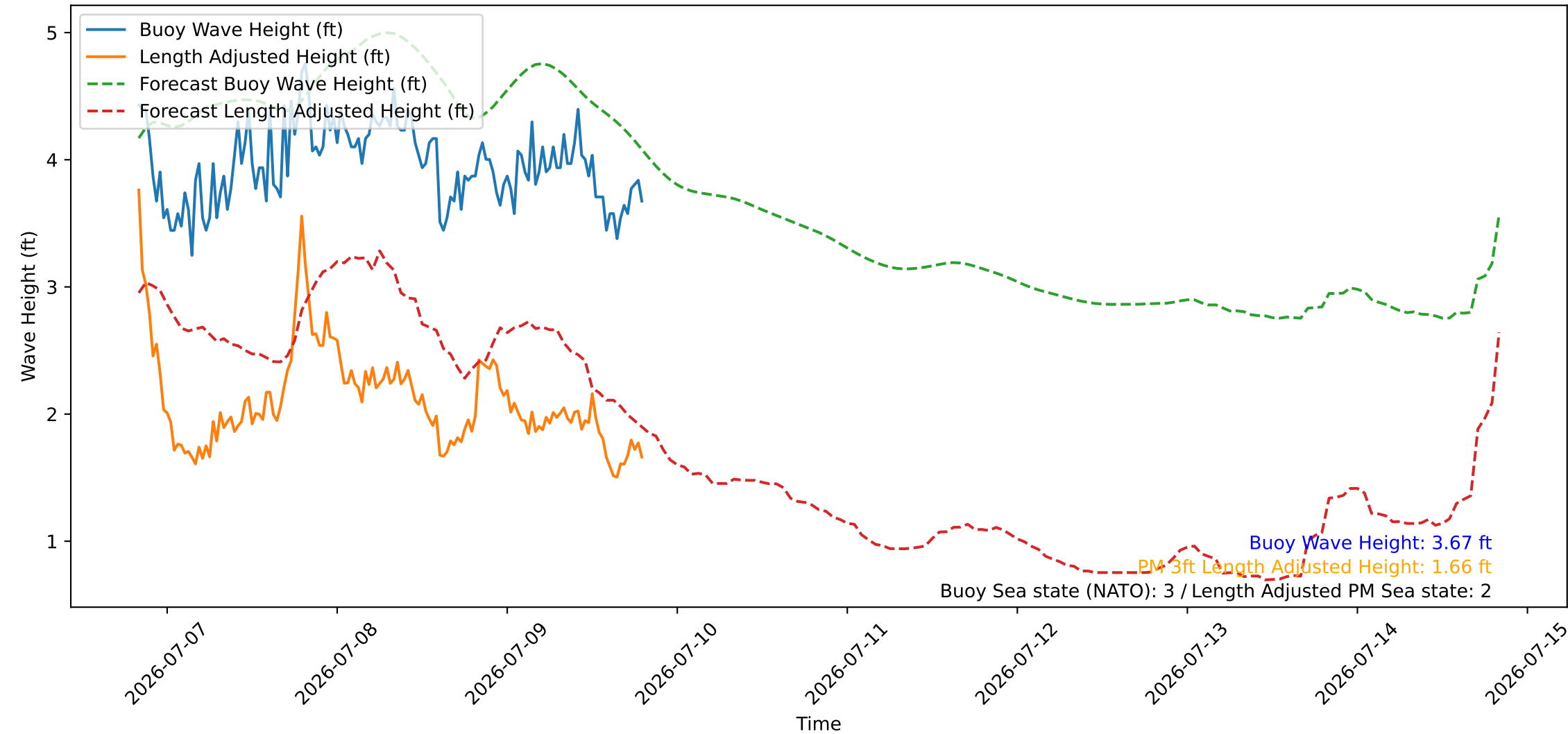
Wave Heights over Time for Green Beach at 2026-07-09 19:51:10
