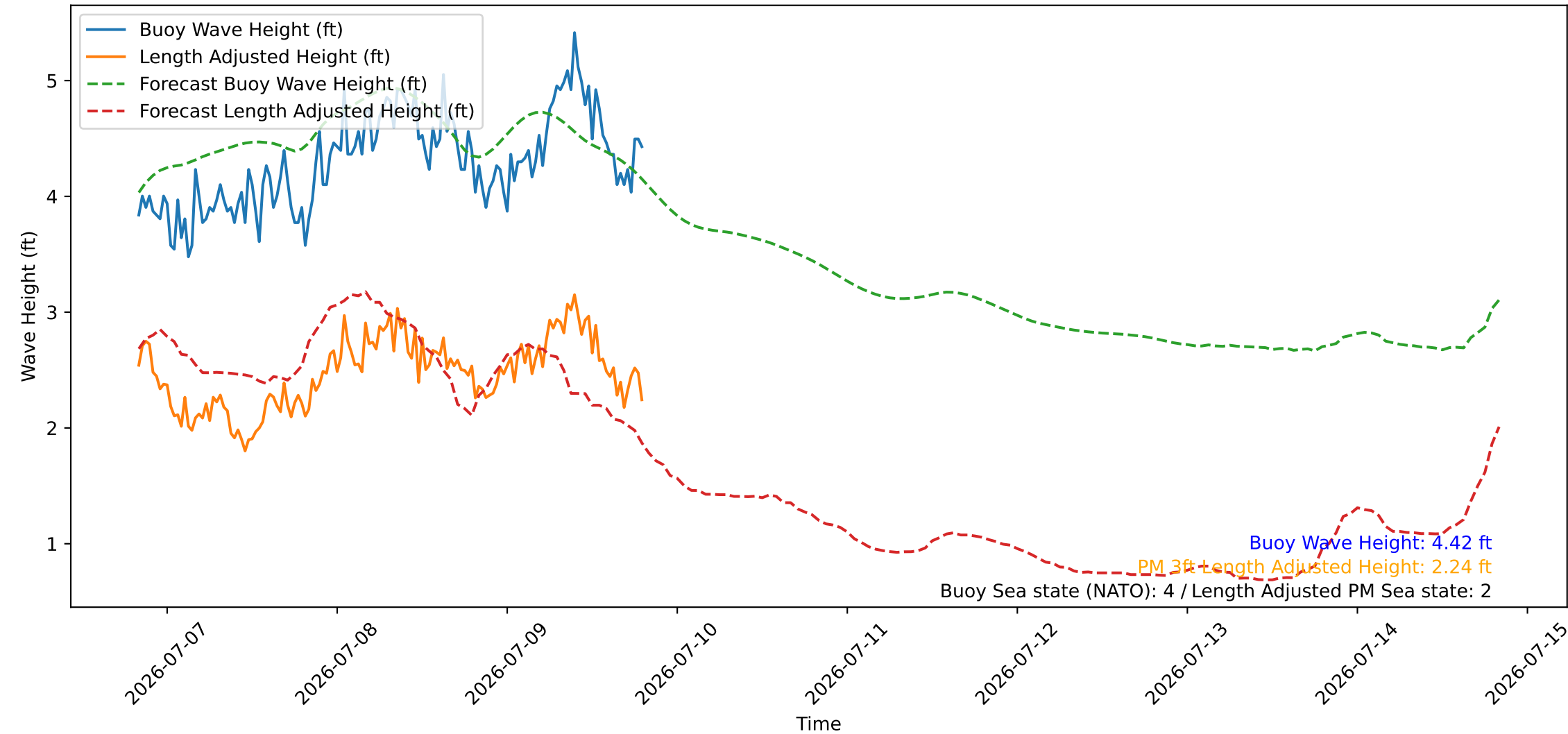
Wave Heights over Time for Oceanside Harbor at 2026-07-09 19:50:27
