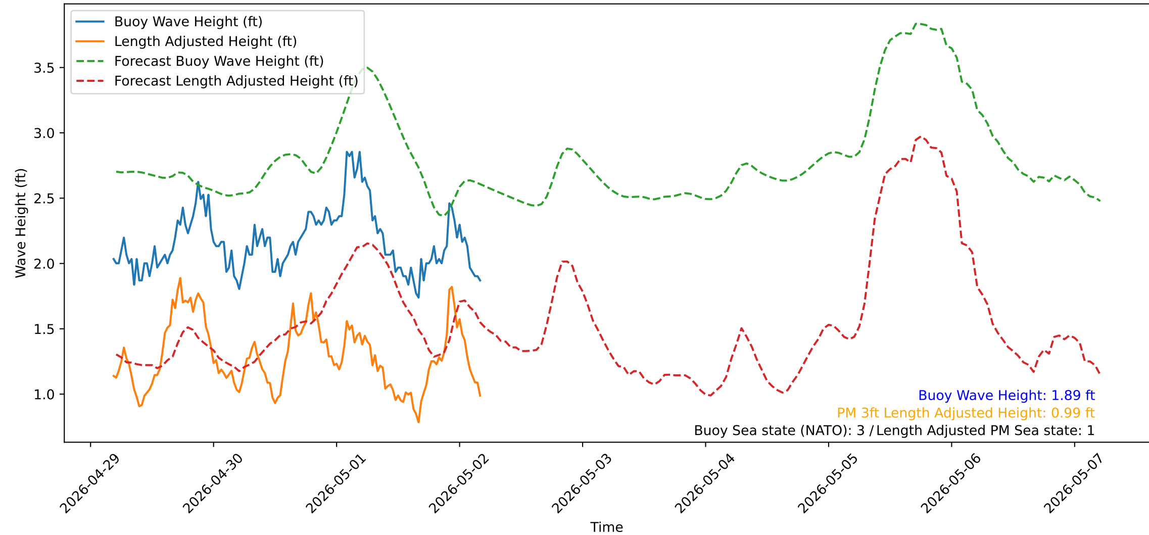
Wave Heights over Time for Green Beach at 2026-05-02 04:41:13
