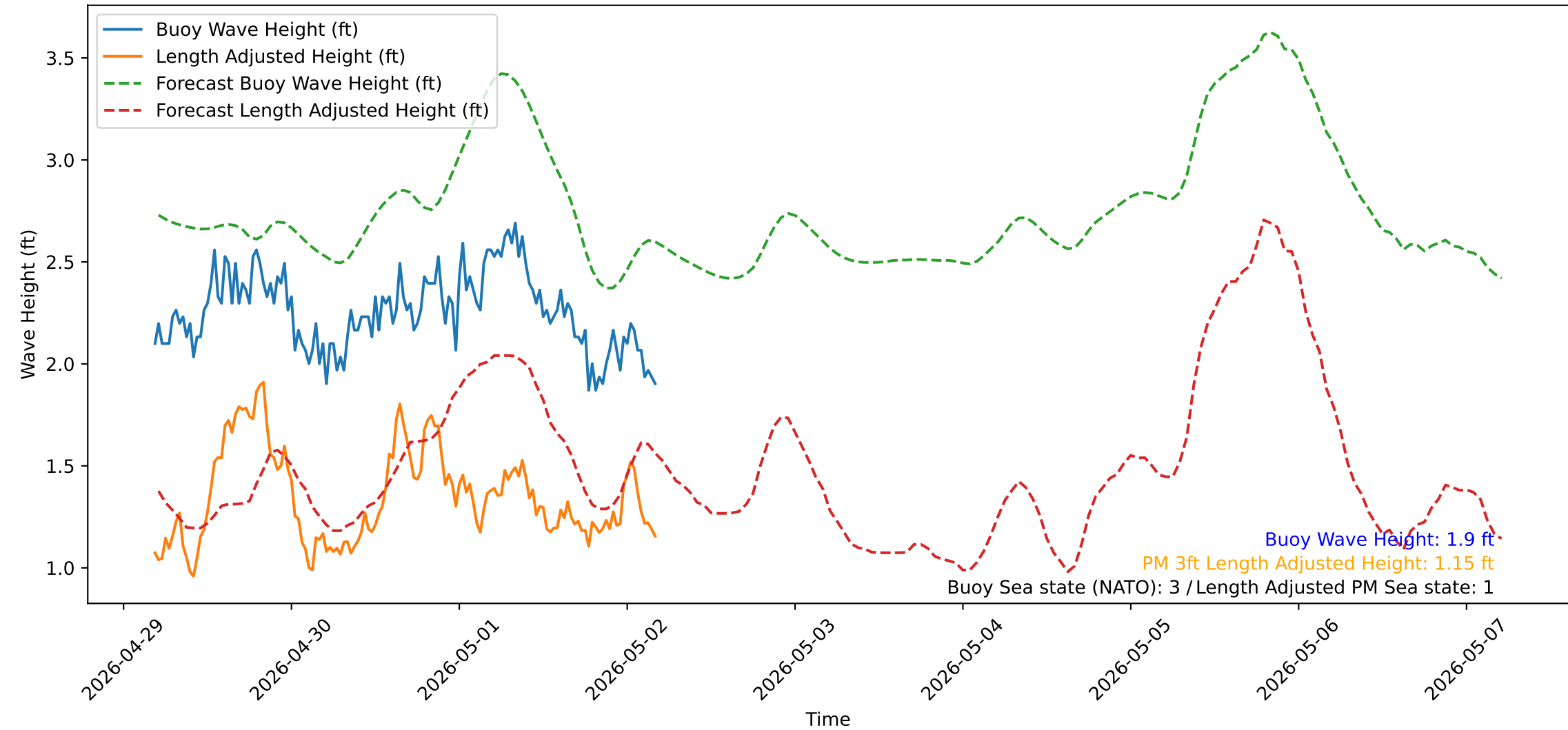
Wave Heights over Time for Oceanside Harbor at 2026-05-02 04:40:31
