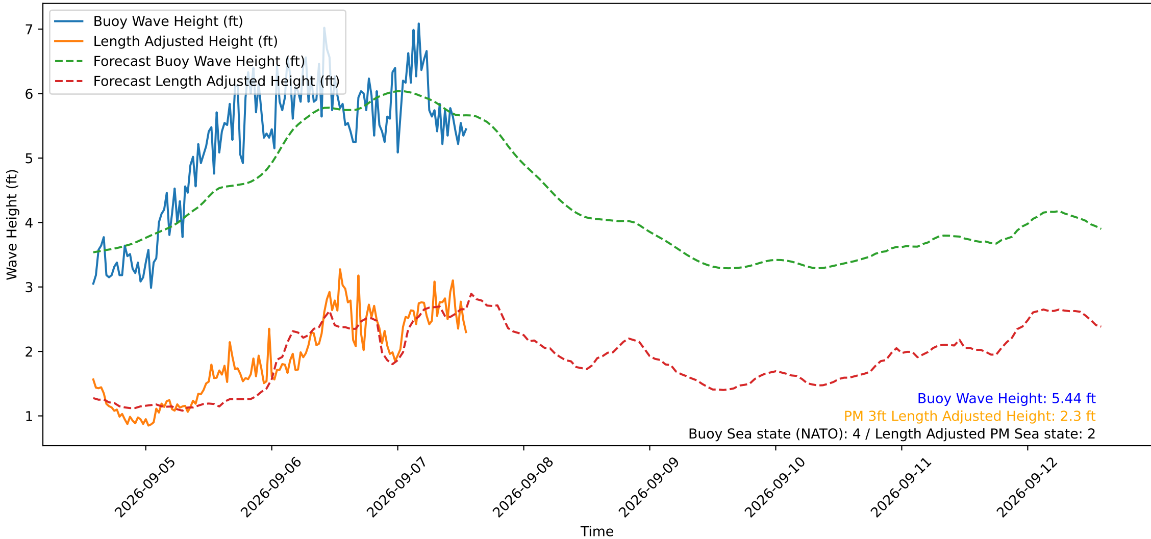
Wave Heights over Time for Oceanside Harbor at 2026-09-07 14:00:30
