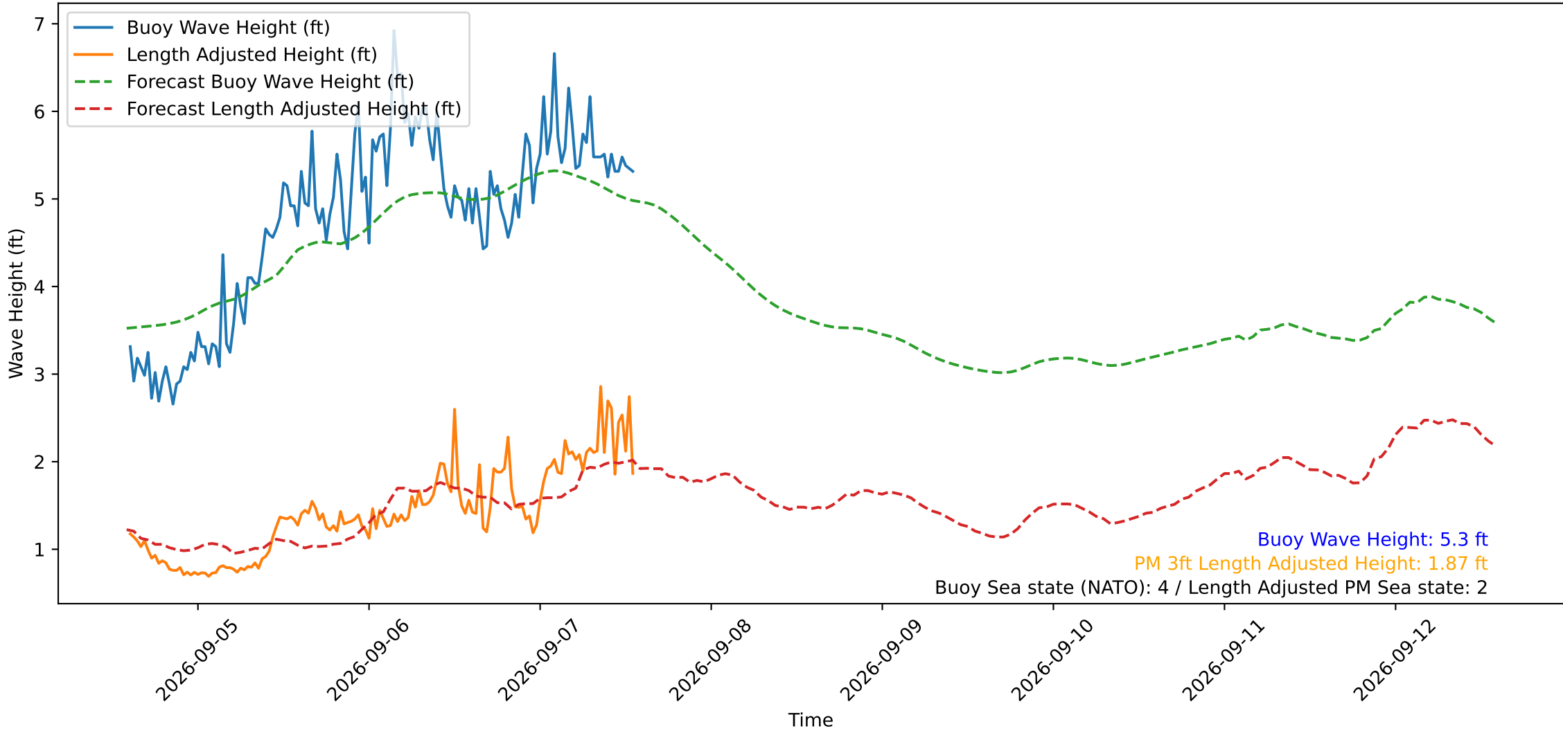
Wave Heights over Time for Red Beach at 2026-09-07 14:00:49
