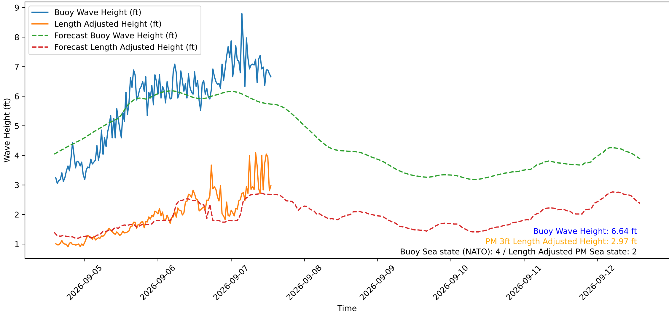
Wave Heights over Time for Green Beach at 2026-09-07 14:01:12
