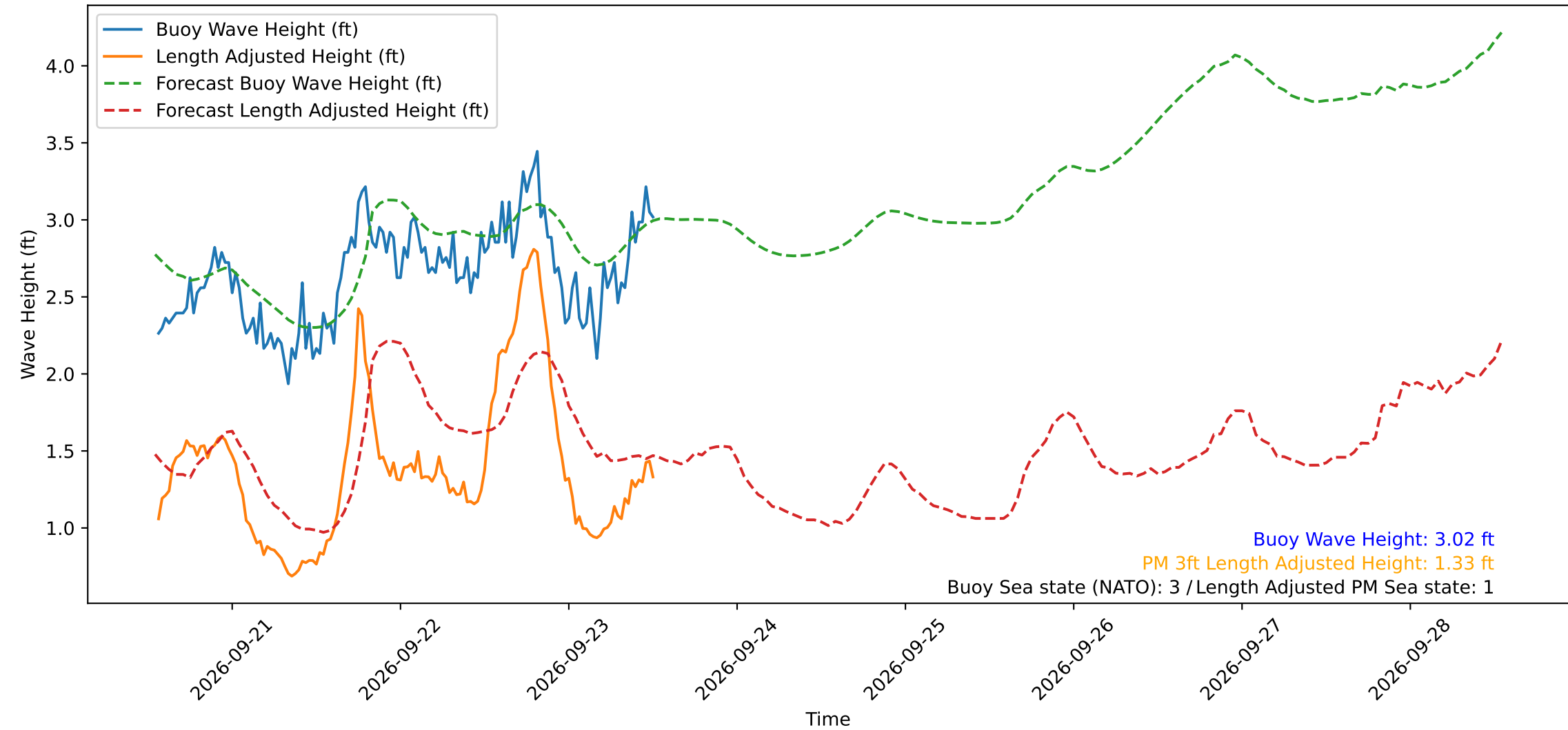
Wave Heights over Time for Green Beach at 2026-09-23 13:01:12
