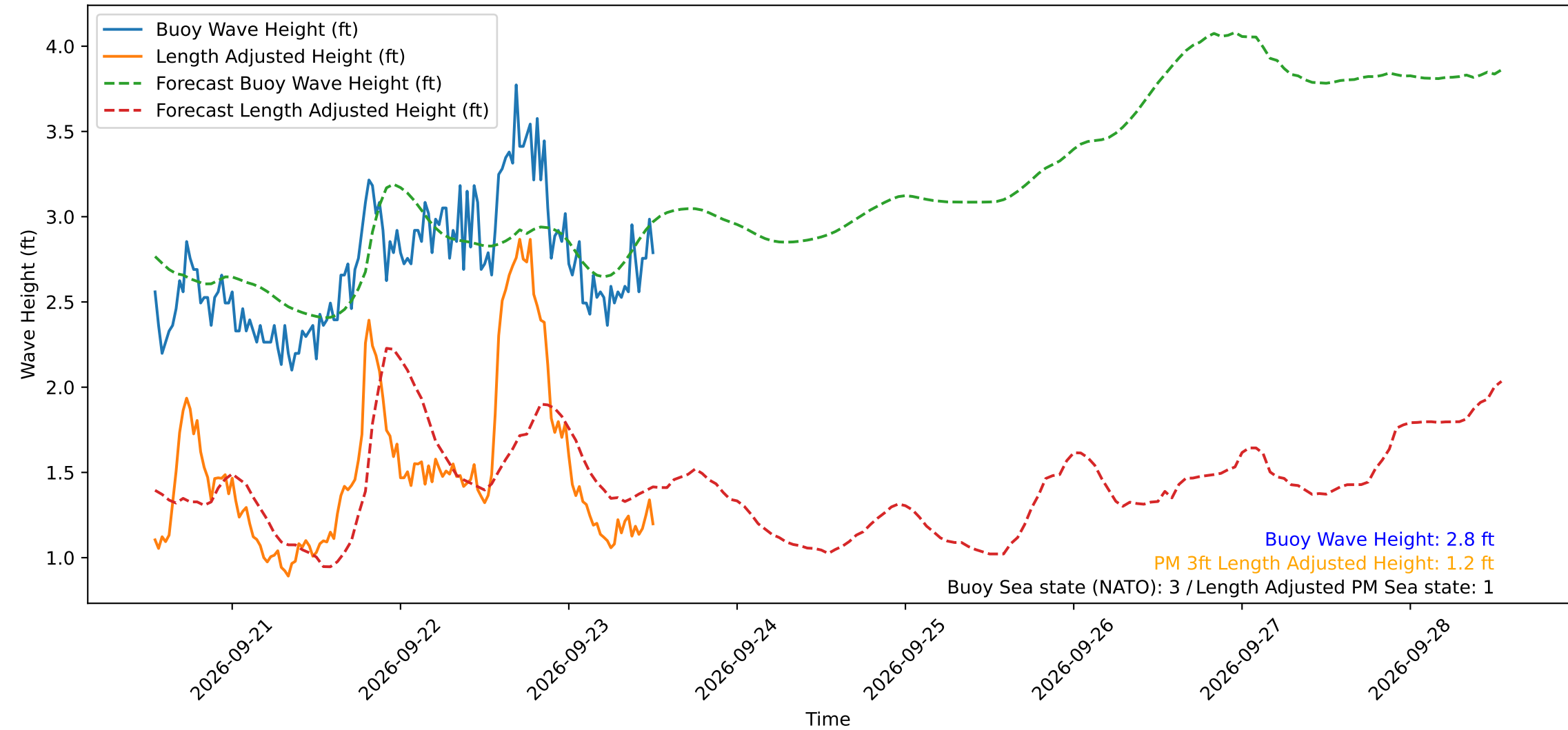
Wave Heights over Time for Oceanside Harbor at 2026-09-23 13:00:30
