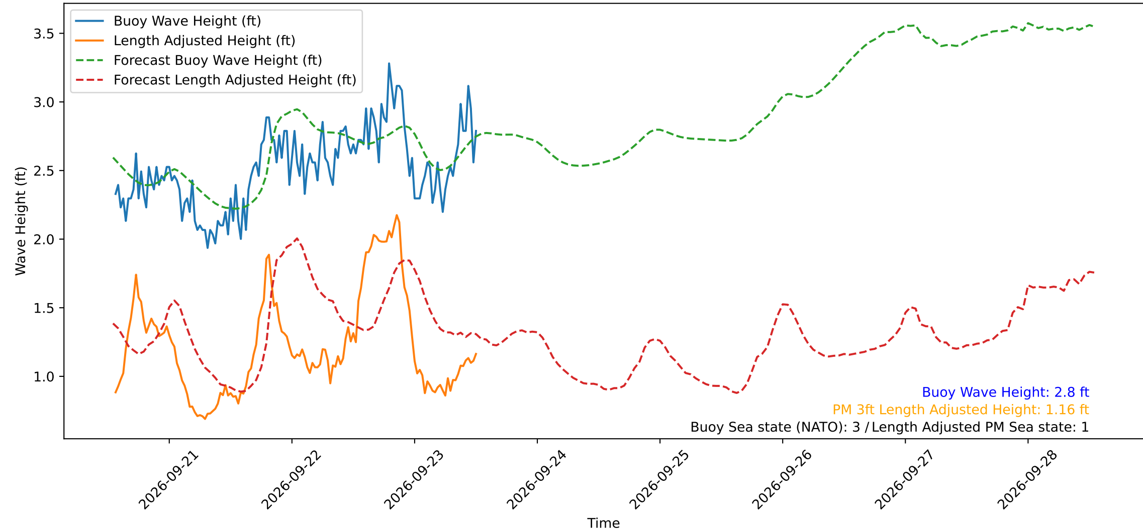
Wave Heights over Time for Red Beach at 2026-09-23 13:00:50
