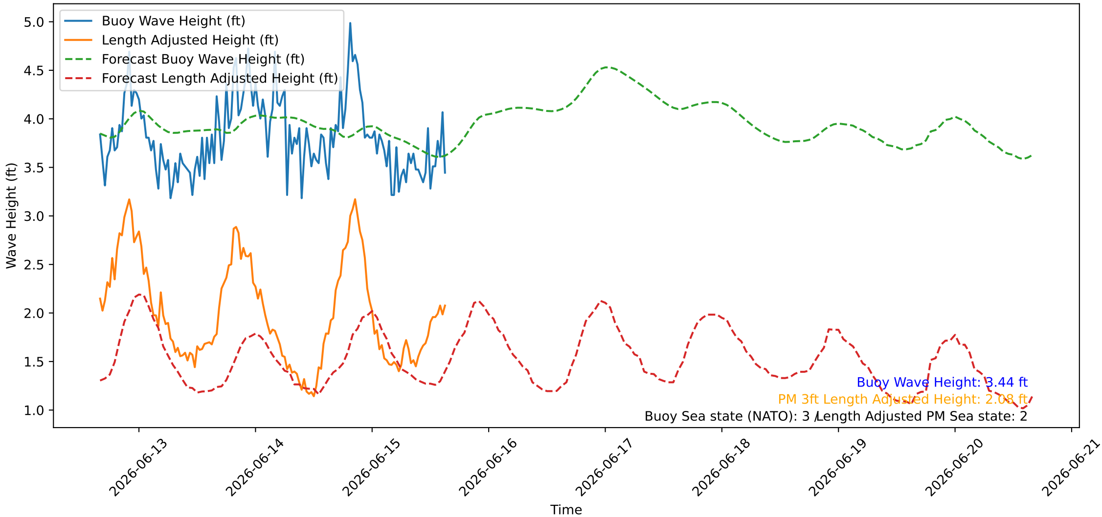
Wave Heights over Time for Oceanside Harbor at 2026-06-15 15:50:26
