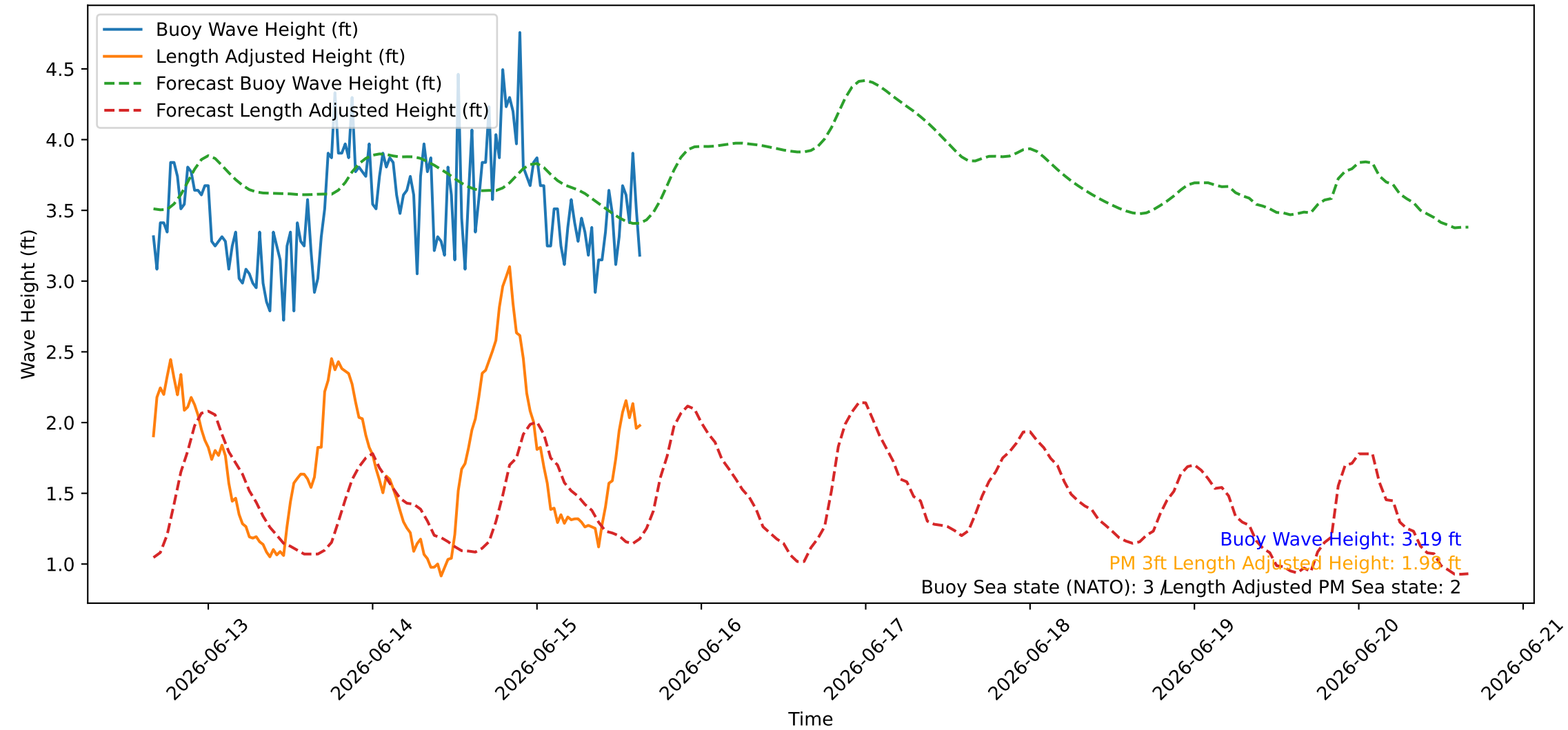
Wave Heights over Time for Red Beach at 2026-06-15 15:50:47
