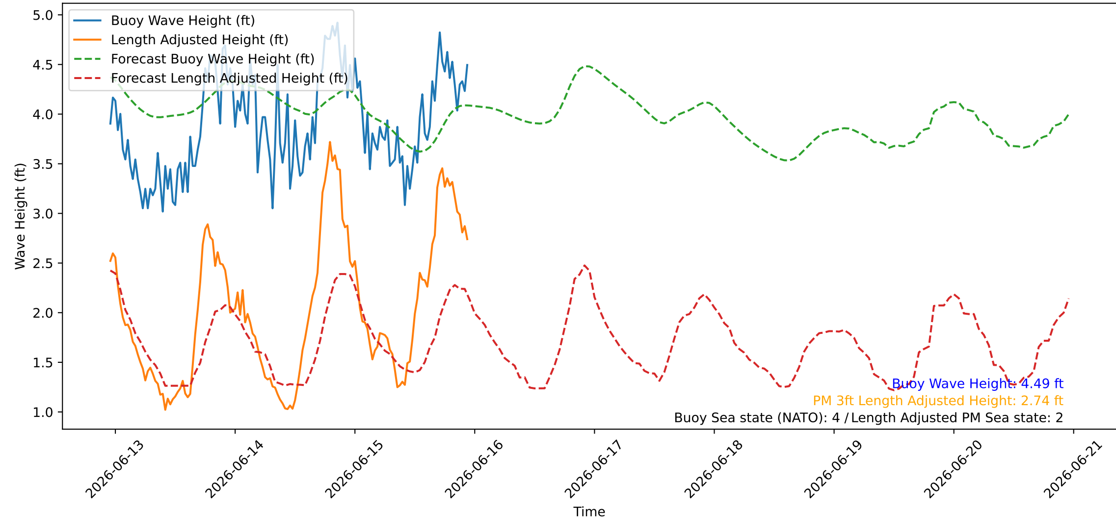
Wave Heights over Time for Green Beach at 2026-06-15 23:11:08
