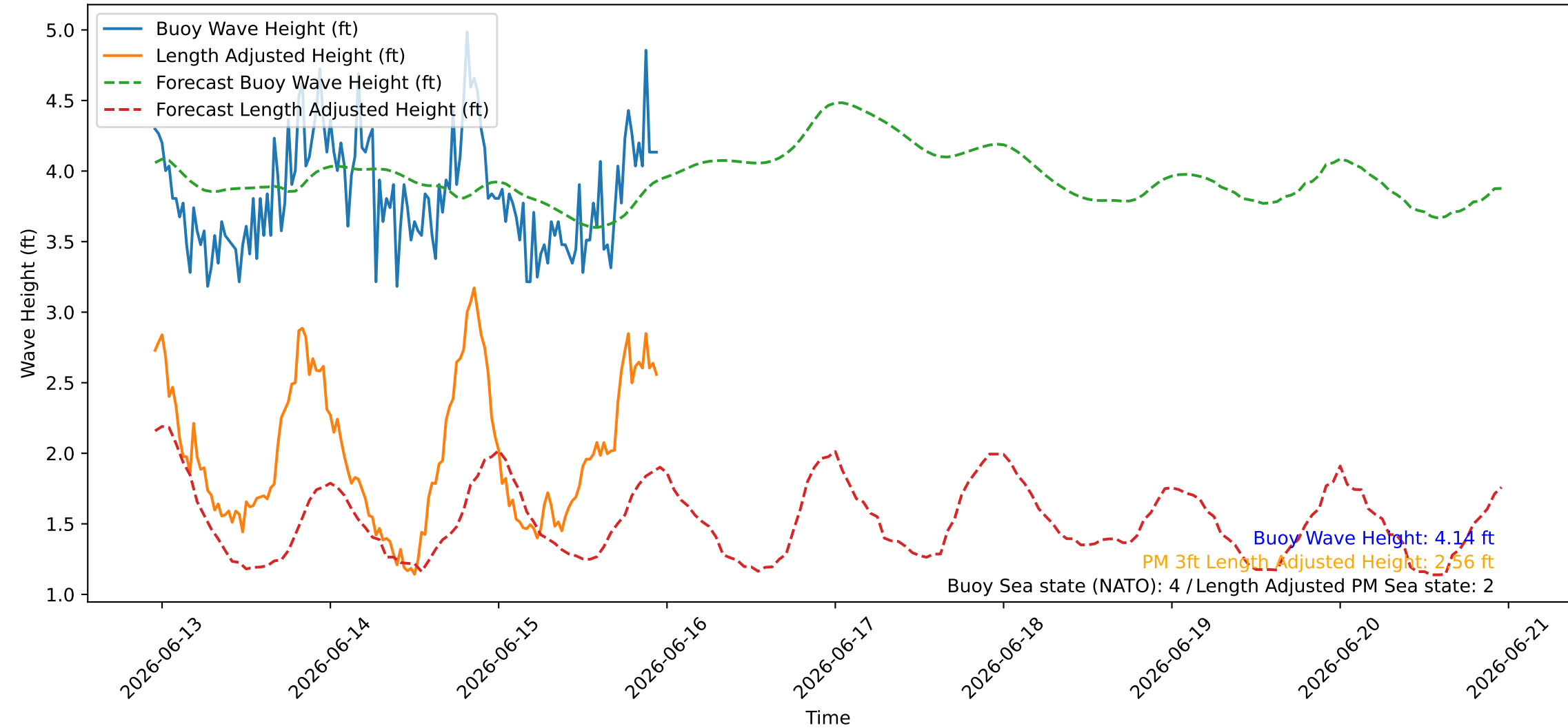
Wave Heights over Time for Oceanside Harbor at 2026-06-15 23:10:26
