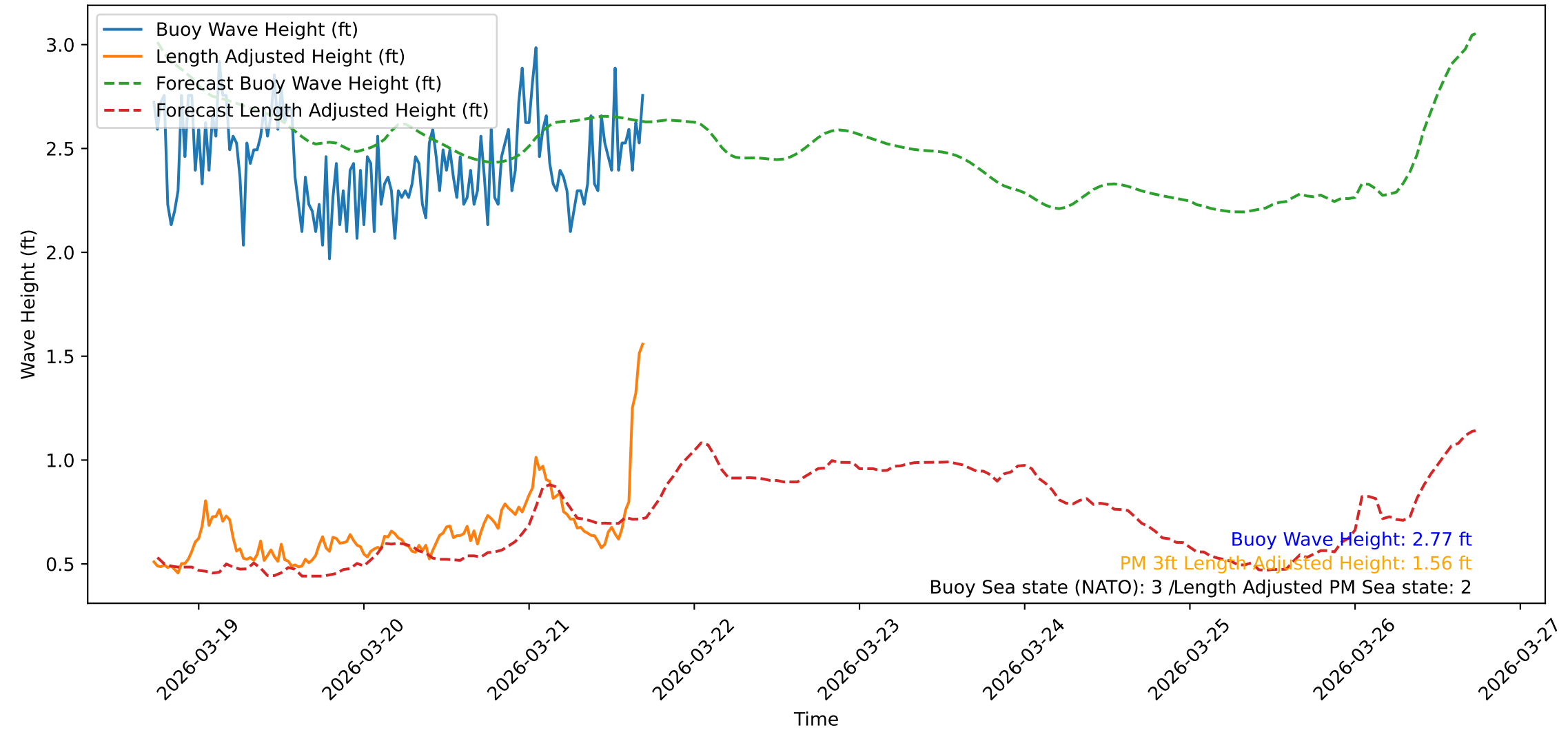
Wave Heights over Time for Oceanside Harbor at 2026-03-21 17:30:32
