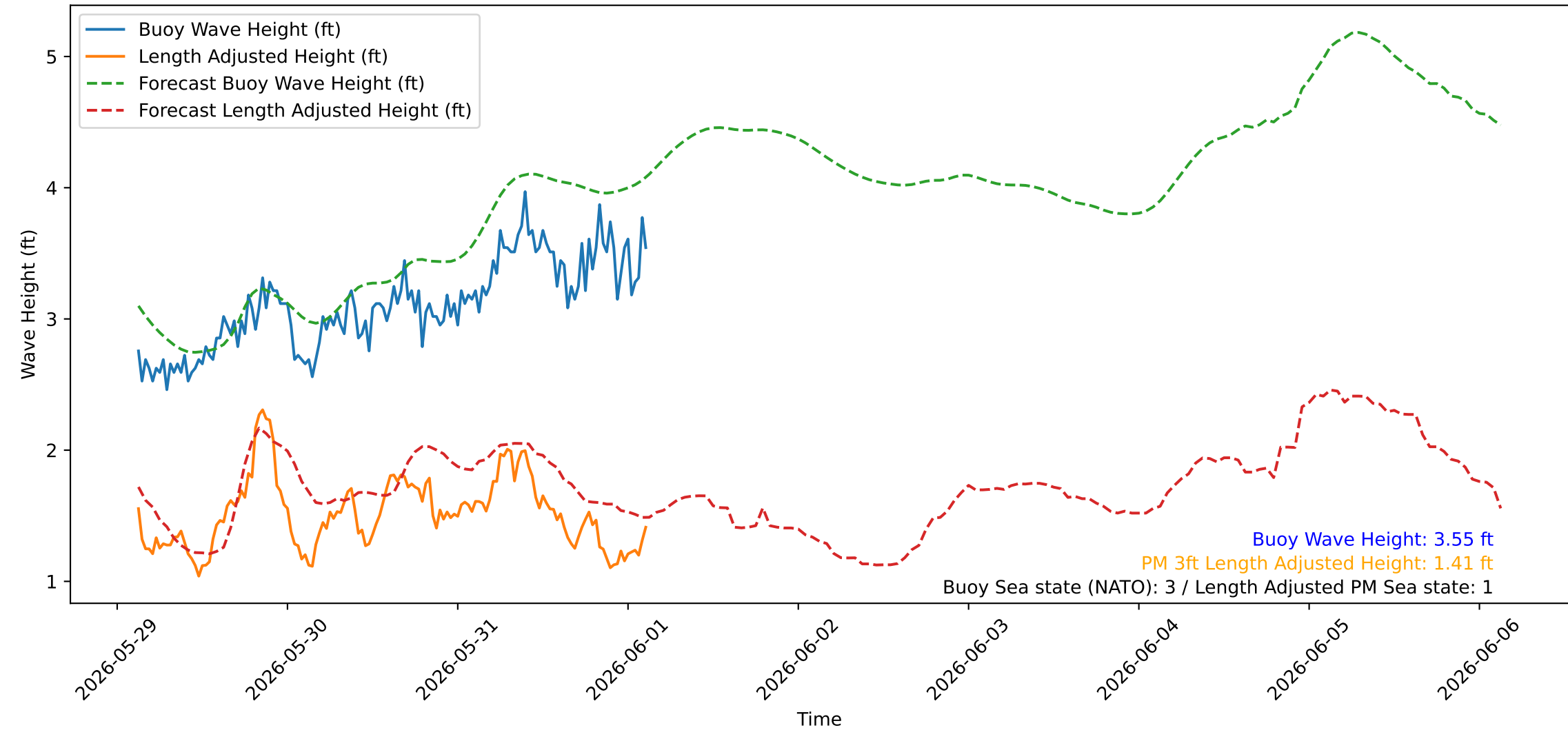
Wave Heights over Time for Green Beach at 2026-06-01 03:11:07
