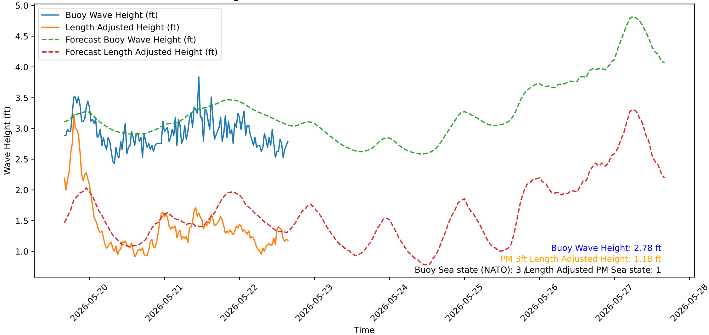
Wave Heights over Time for Oceanside Harbor at 2026-05-22 16:00:32
