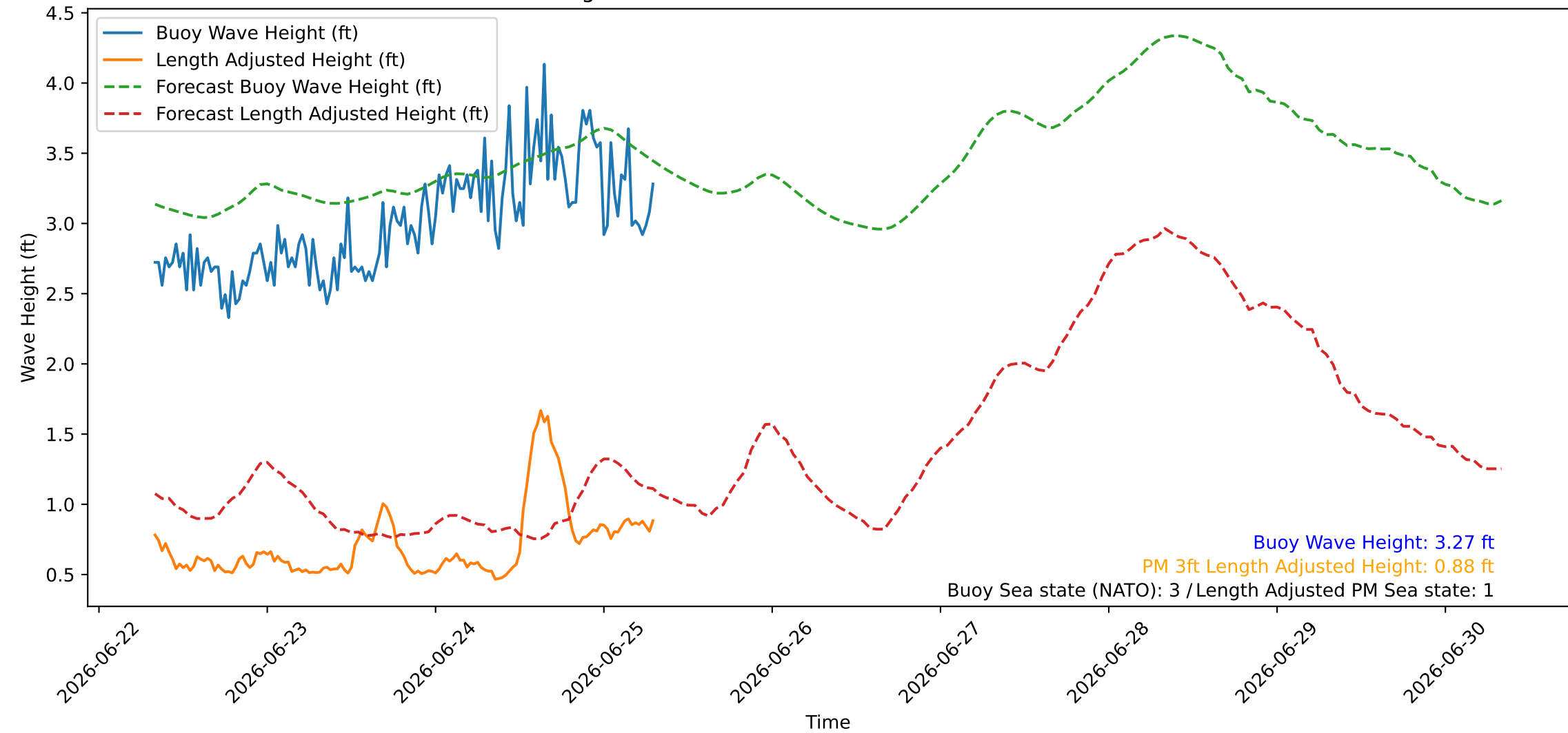
Wave Heights over Time for Red Beach at 2026-06-25 07:50:47
