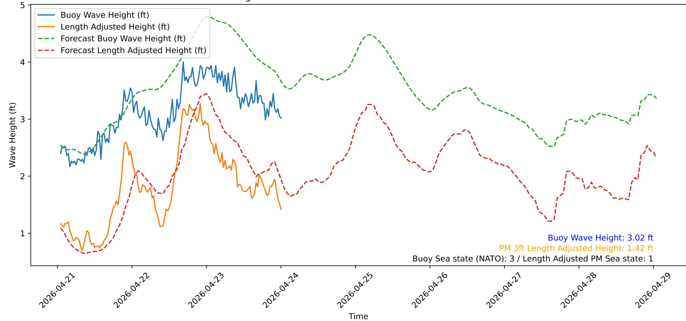
Wave Heights over Time for Green Beach at 2026-04-24 00:51:14
