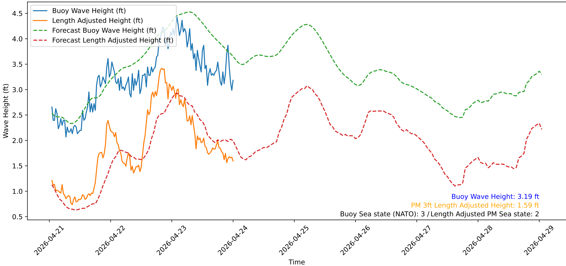
Wave Heights over Time for Oceanside Harbor at 2026-04-24 00:50:31
