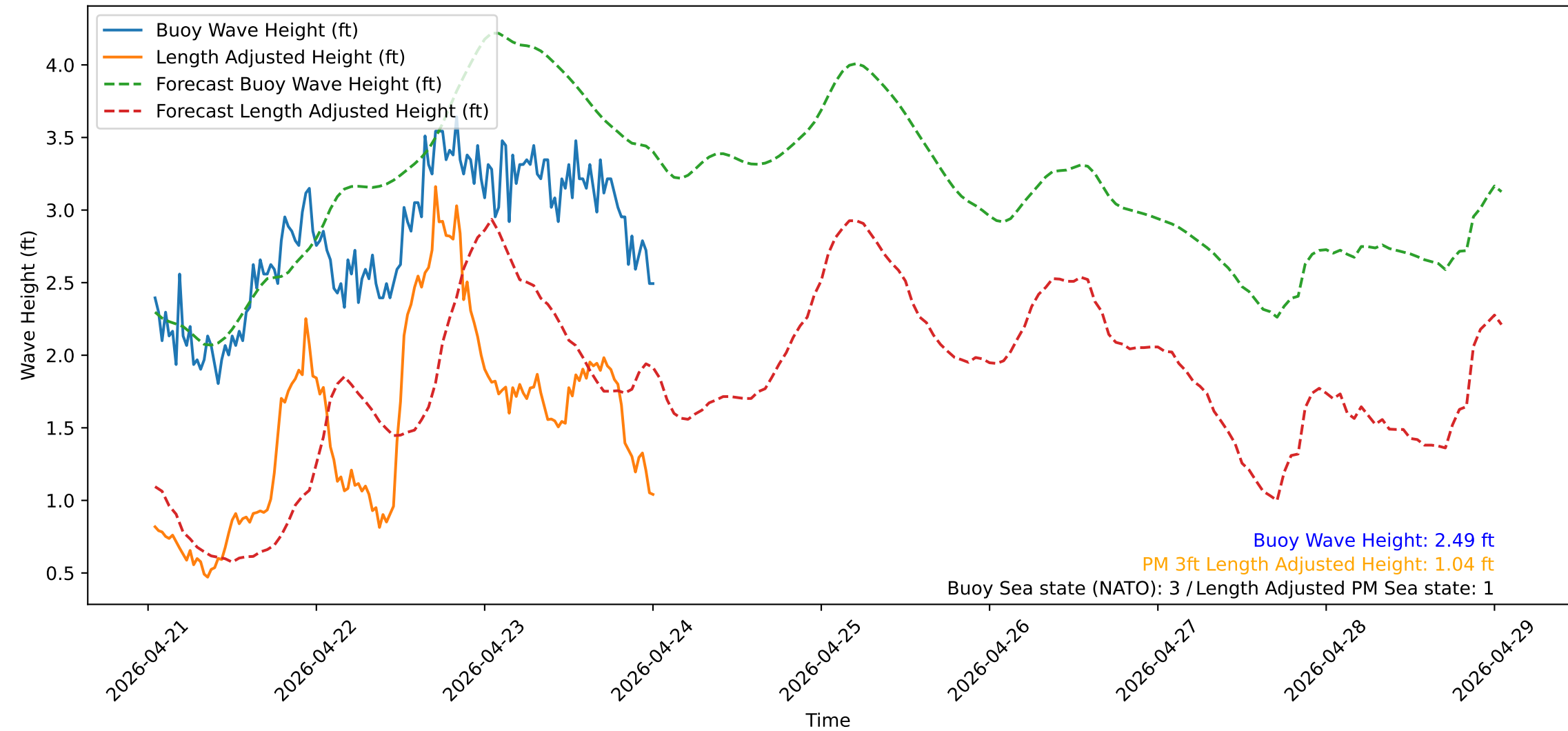
Wave Heights over Time for Red Beach at 2026-04-24 00:50:51
