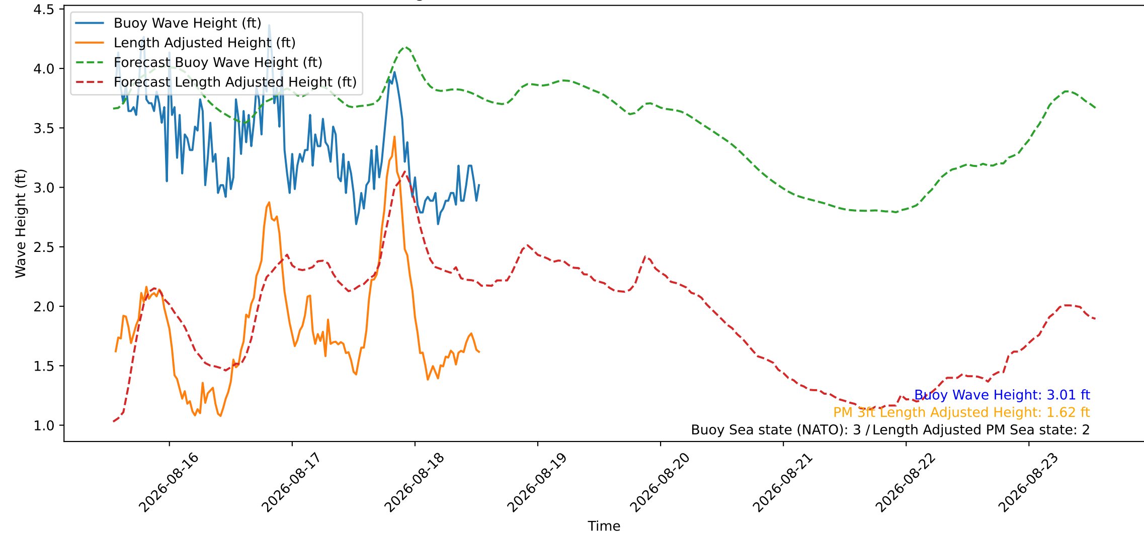
Wave Heights over Time for Green Beach at 2026-08-18 13:11:08
