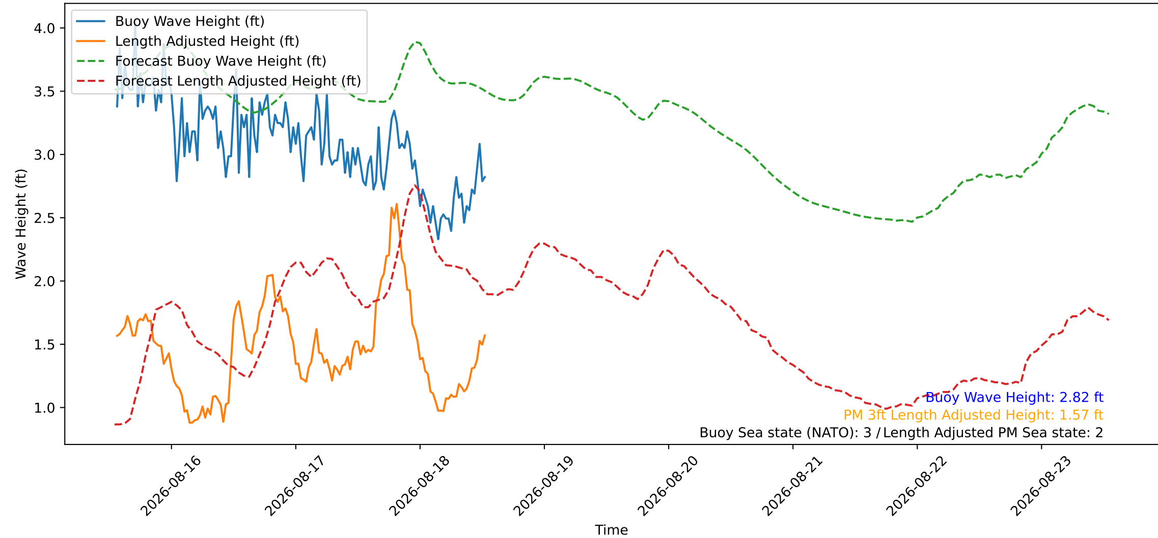
Wave Heights over Time for Red Beach at 2026-08-18 13:10:45
