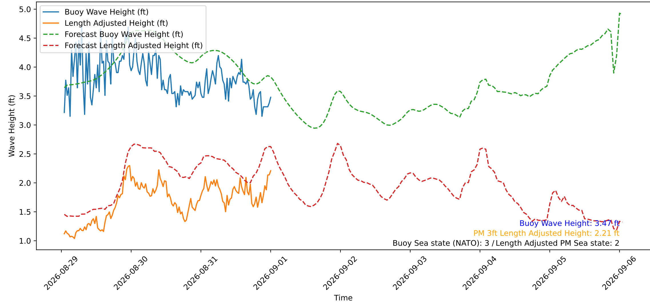
Wave Heights over Time for Red Beach at 2026-09-01 00:40:49
