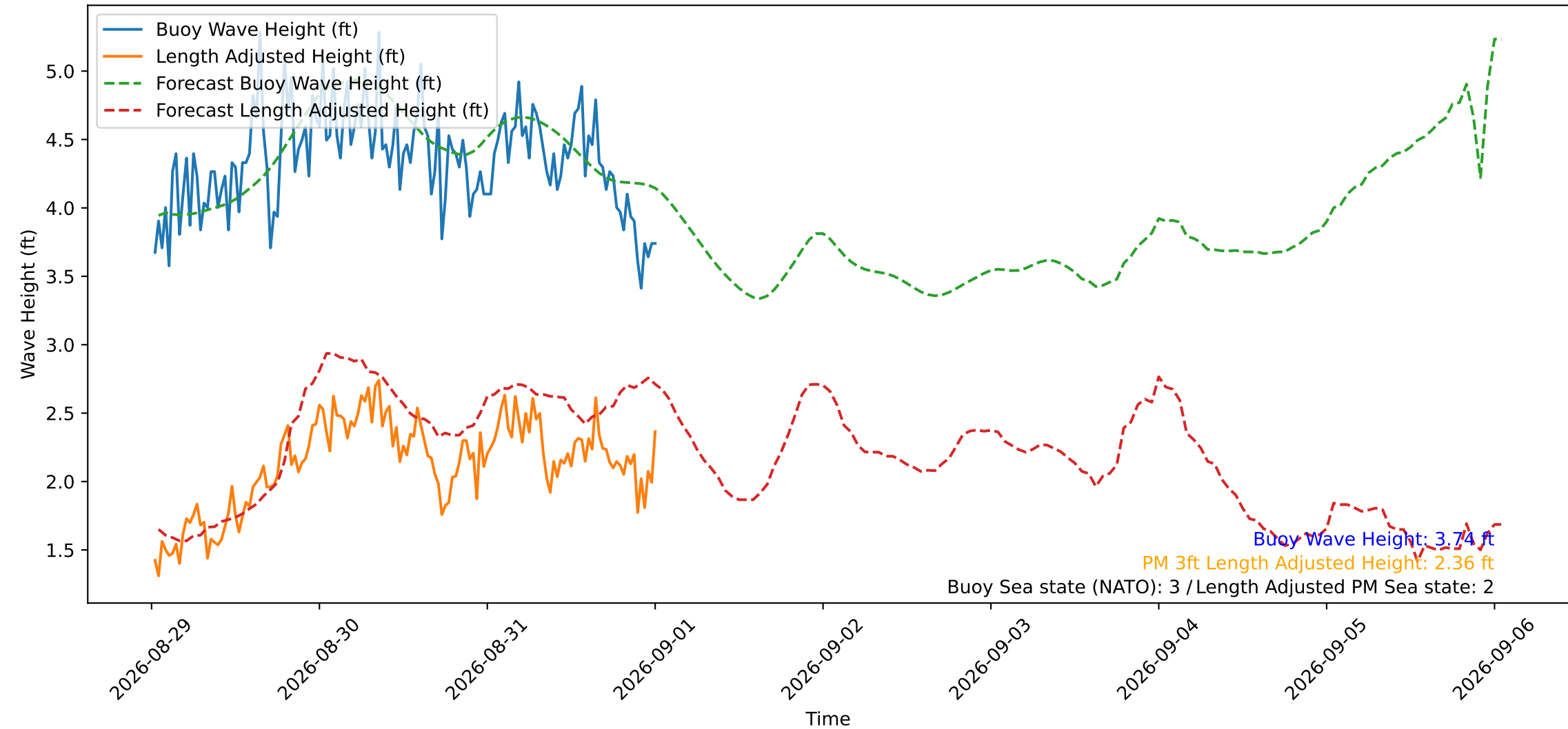
Wave Heights over Time for Oceanside Harbor at 2026-09-01 00:40:29
