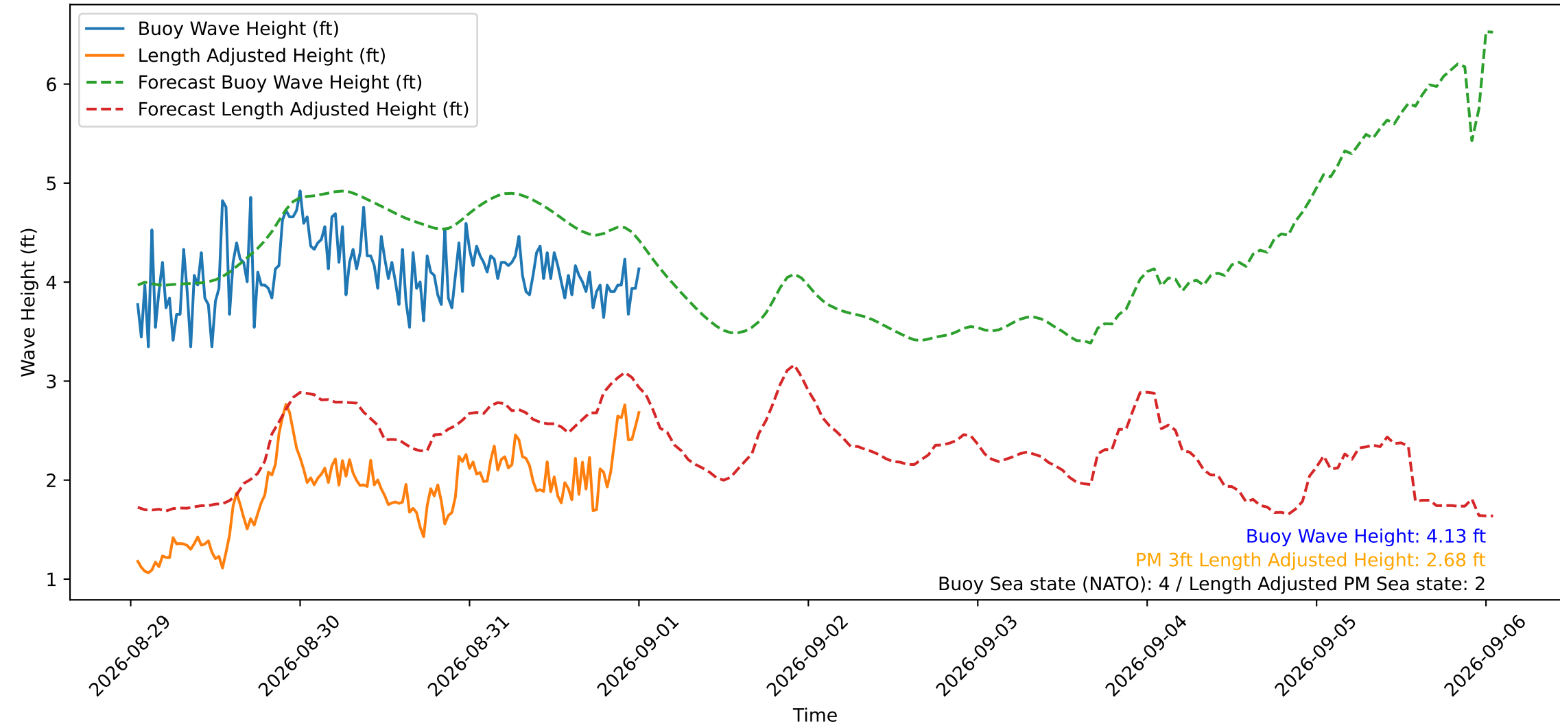
Wave Heights over Time for Green Beach at 2026-09-01 00:41:11
