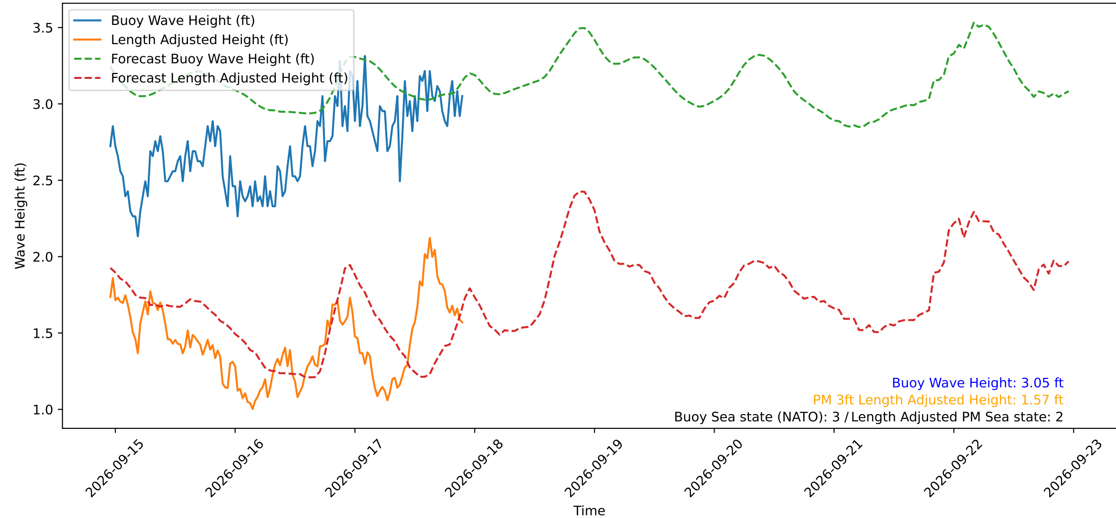
Wave Heights over Time for Green Beach at 2026-09-17 22:31:12
