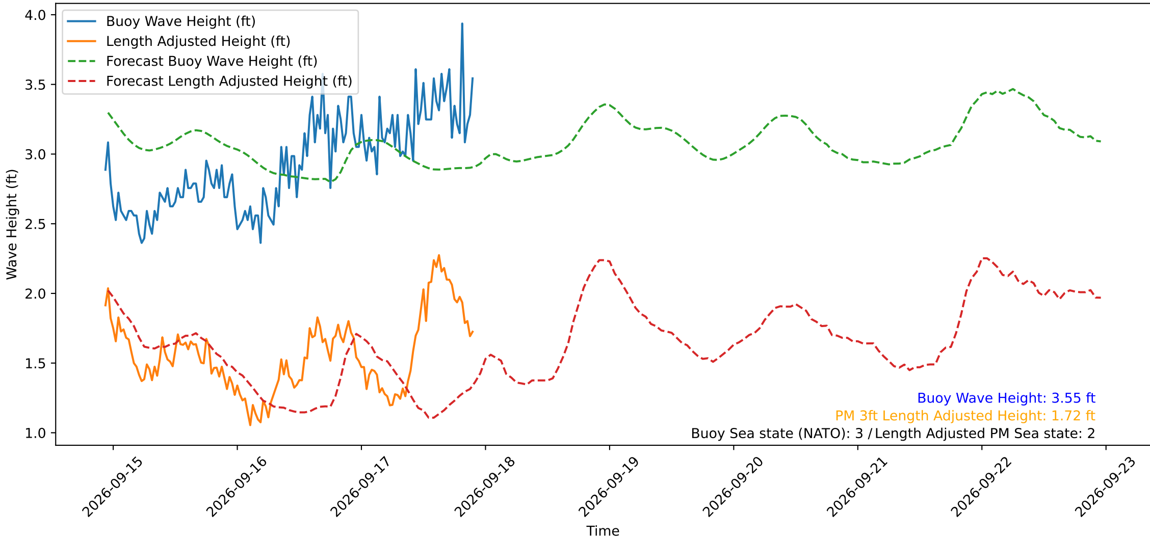
Wave Heights over Time for Oceanside Harbor at 2026-09-17 22:30:29
