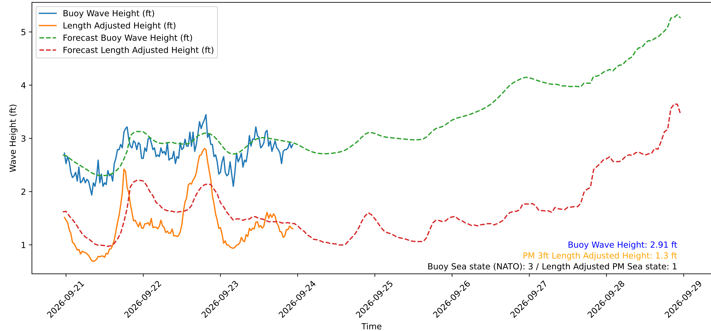
Wave Heights over Time for Green Beach at 2026-09-23 23:21:16
