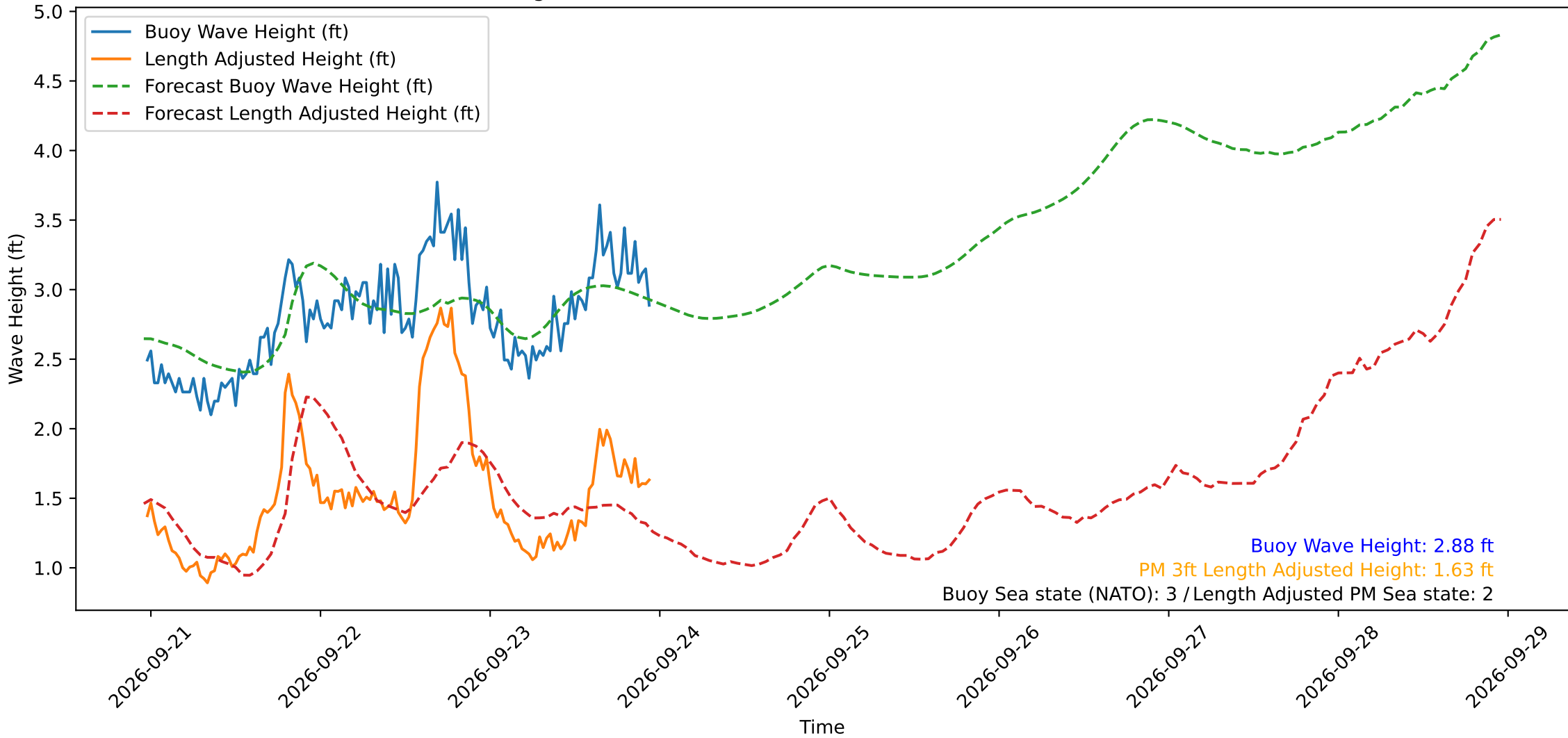
Wave Heights over Time for Oceanside Harbor at 2026-09-23 23:20:30
