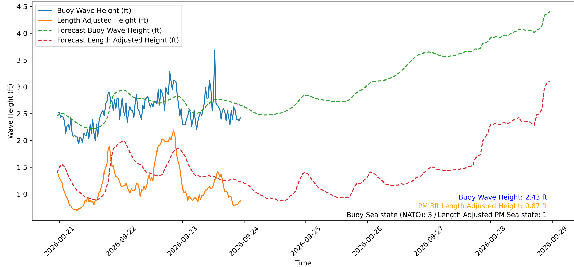
Wave Heights over Time for Red Beach at 2026-09-23 23:20:52
