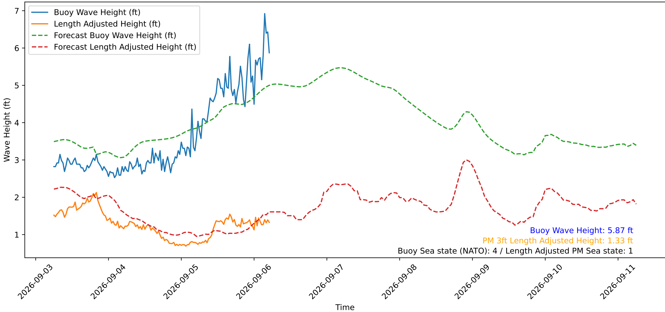
Wave Heights over Time for Red Beach at 2026-09-06 05:50:51
