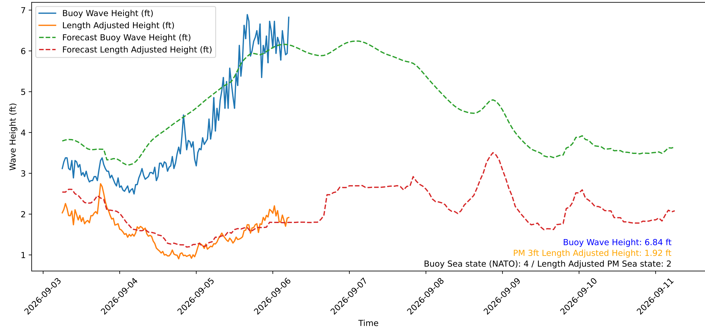
Wave Heights over Time for Green Beach at 2026-09-06 05:51:15
