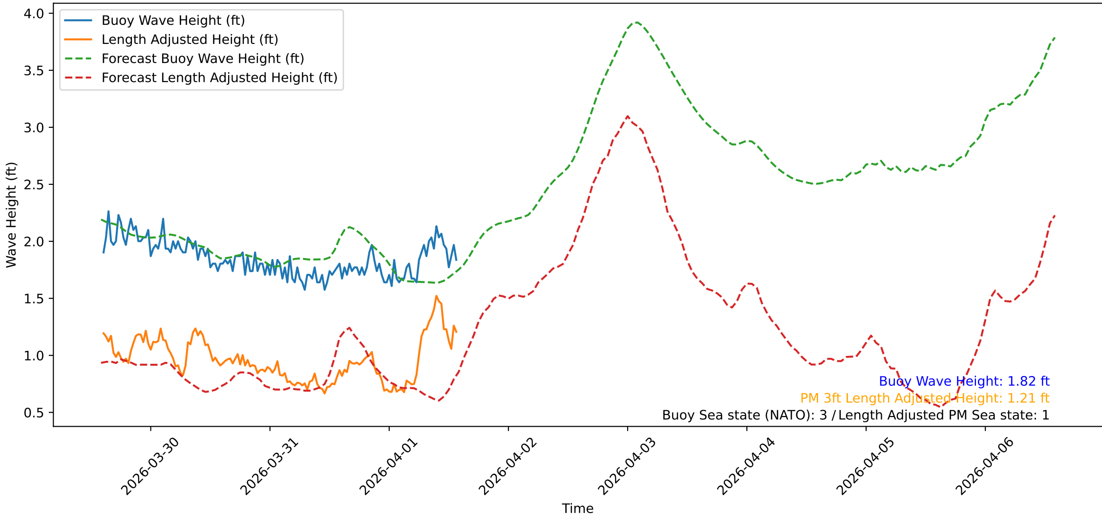
Wave Heights over Time for Oceanside Harbor at 2026-04-01 14:20:31
