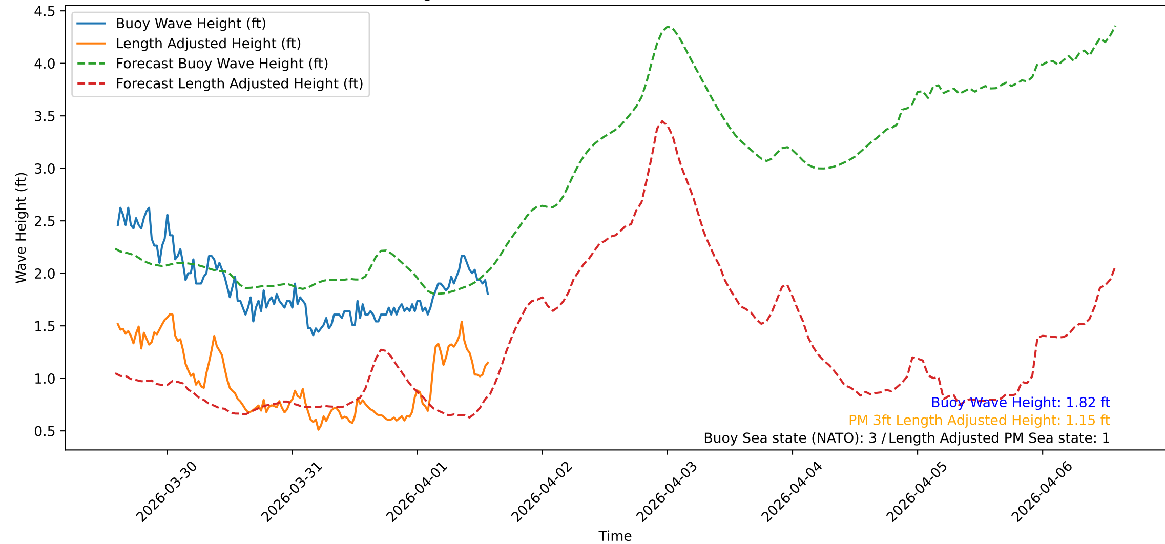
Wave Heights over Time for Green Beach at 2026-04-01 14:21:10
