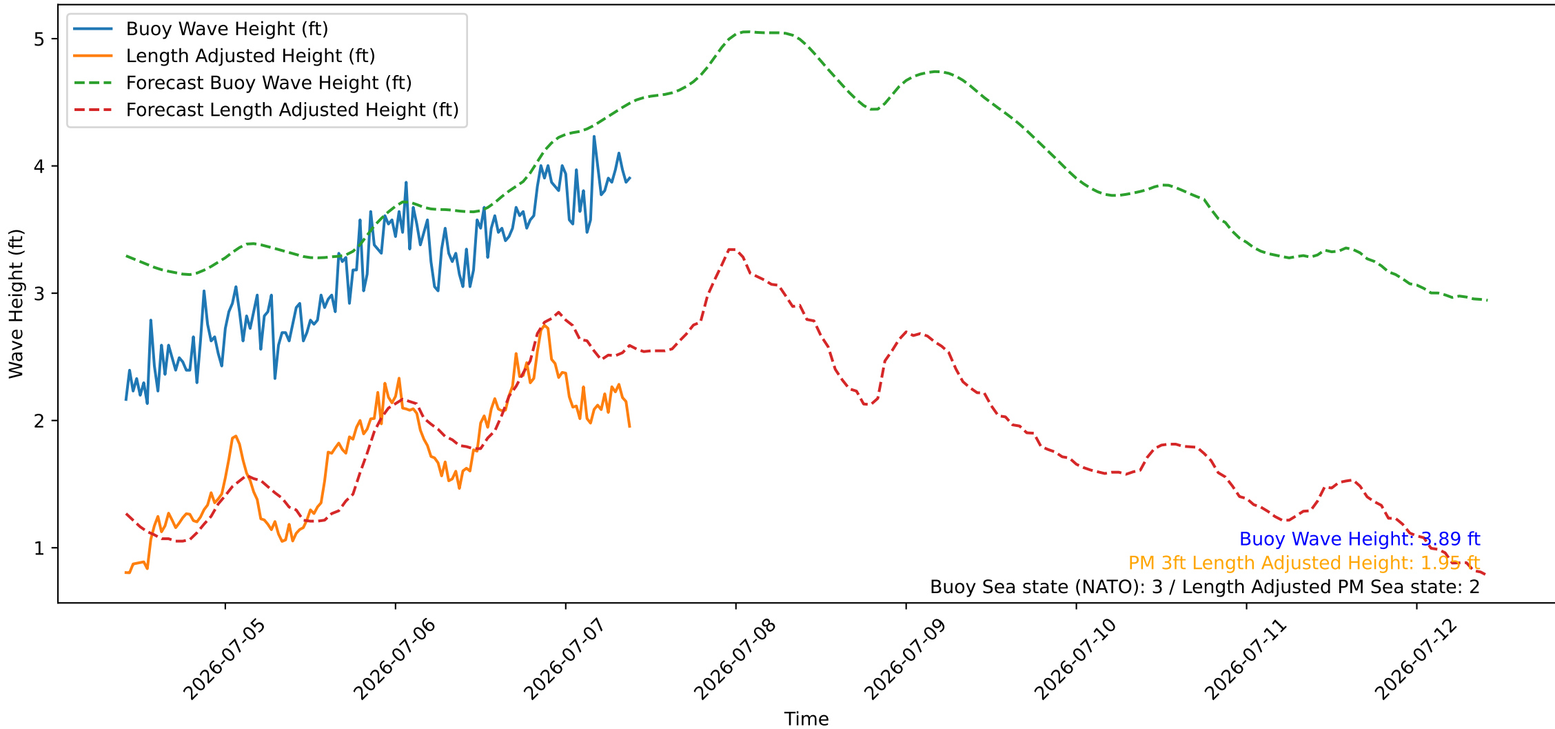
Wave Heights over Time for Oceanside Harbor at 2026-07-07 10:00:26
