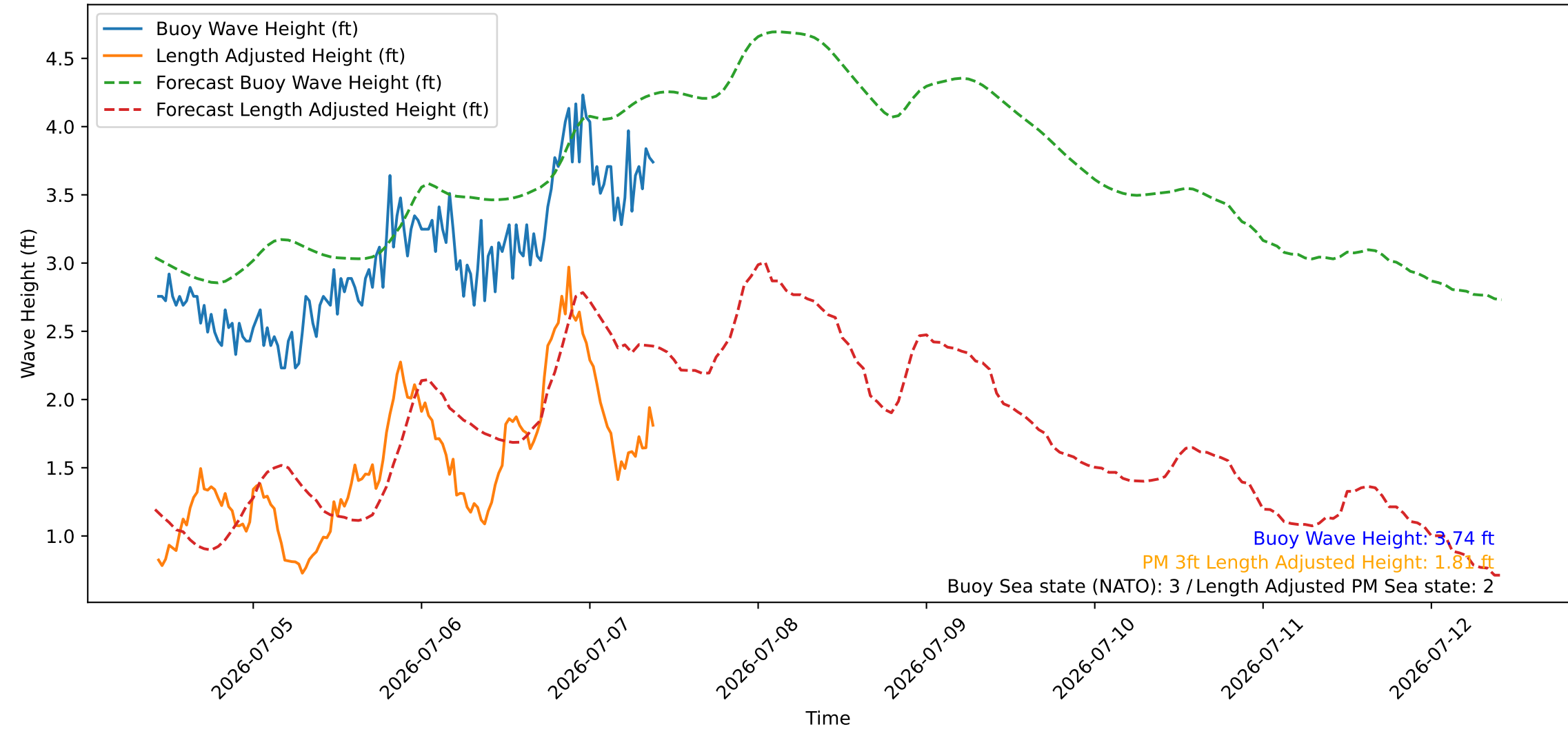
Wave Heights over Time for Red Beach at 2026-07-07 10:00:45
