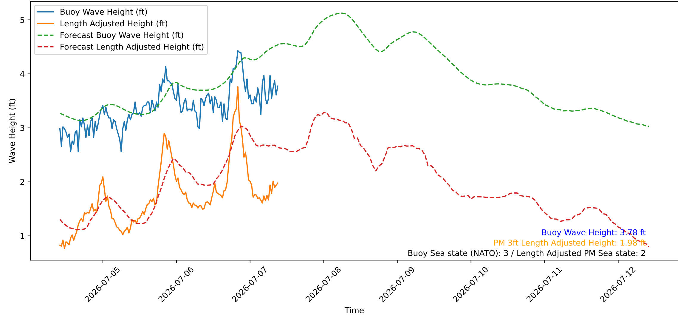
Wave Heights over Time for Green Beach at 2026-07-07 10:01:07
