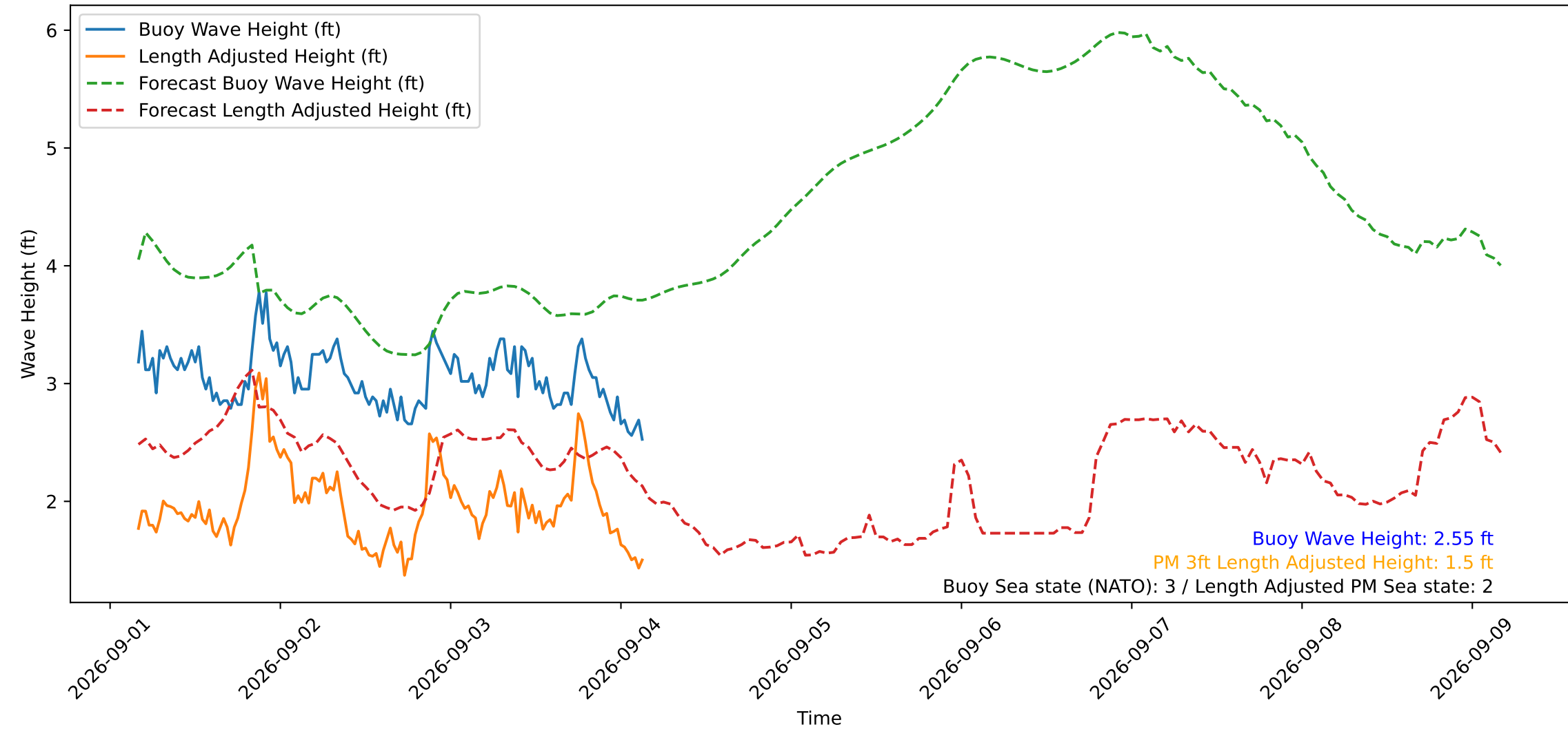
Wave Heights over Time for Green Beach at 2026-09-04 03:41:12
