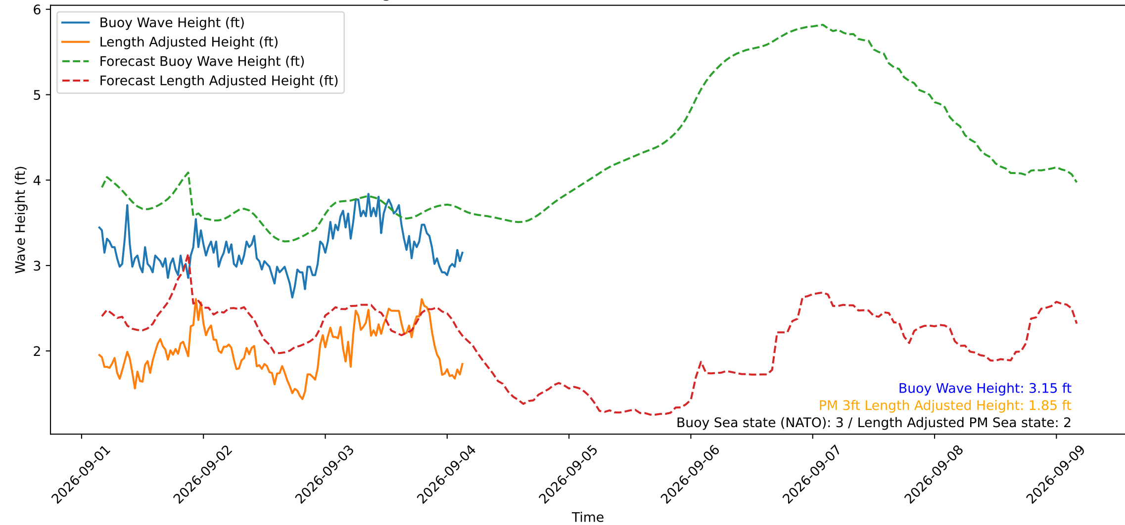
Wave Heights over Time for Oceanside Harbor at 2026-09-04 03:40:29
