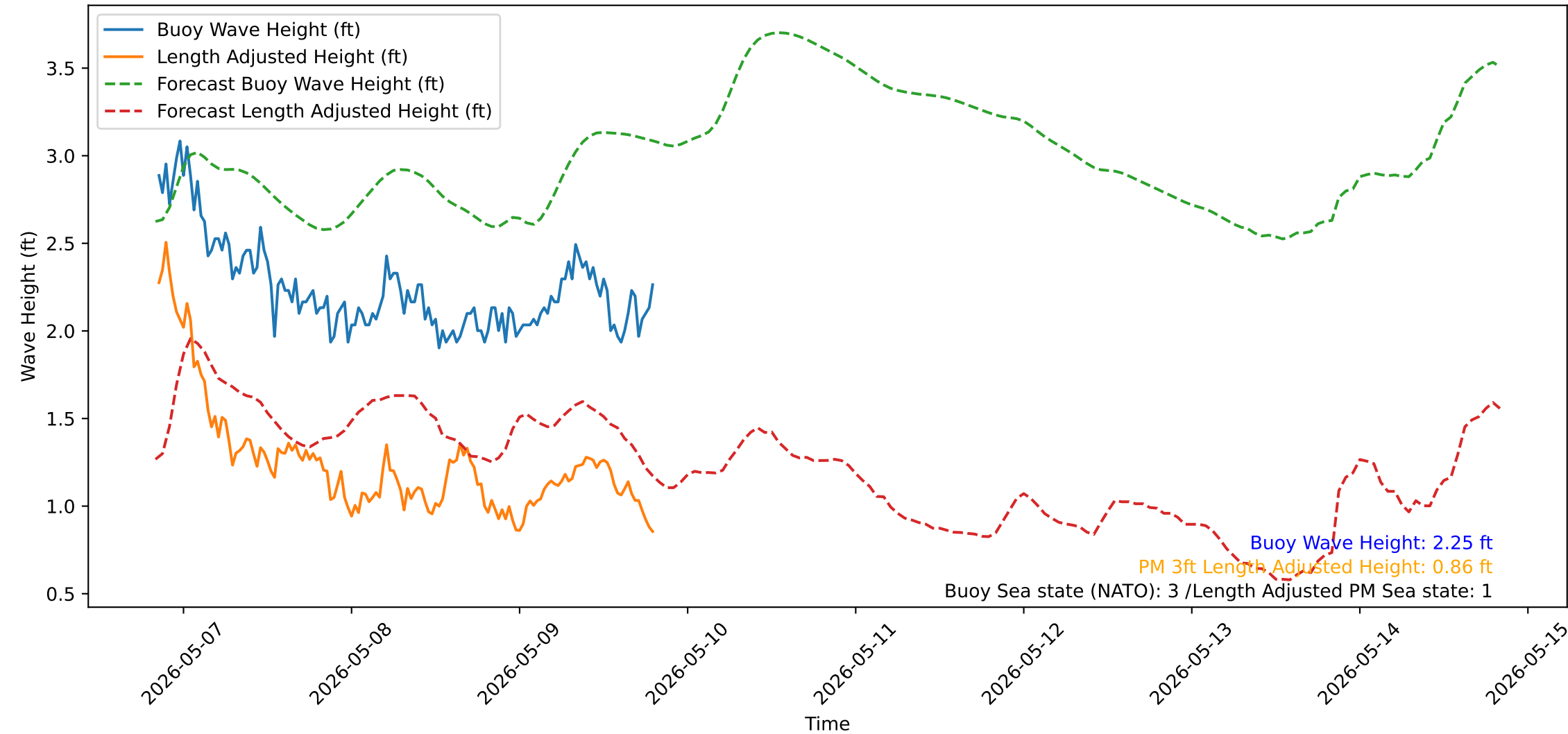
Wave Heights over Time for Red Beach at 2026-05-09 20:10:51
