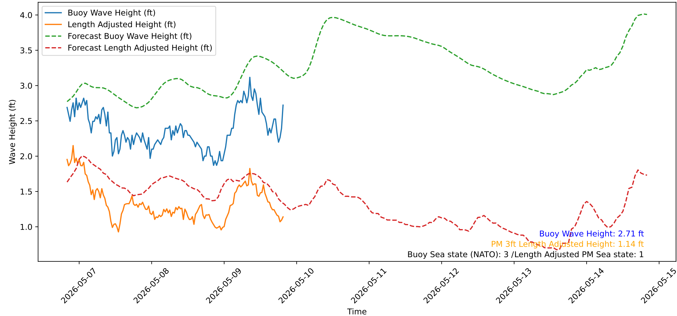
Wave Heights over Time for Oceanside Harbor at 2026-05-09 20:10:32
