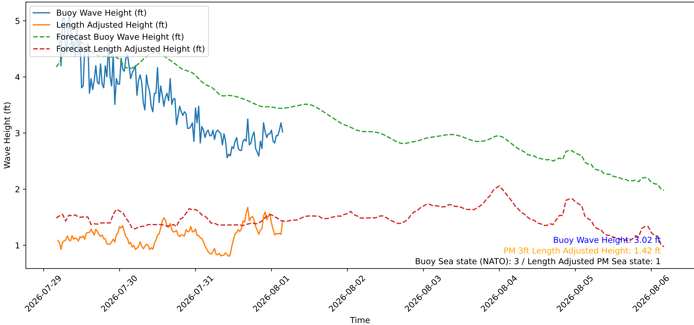
Wave Heights over Time for Red Beach at 2026-08-01 04:10:45
