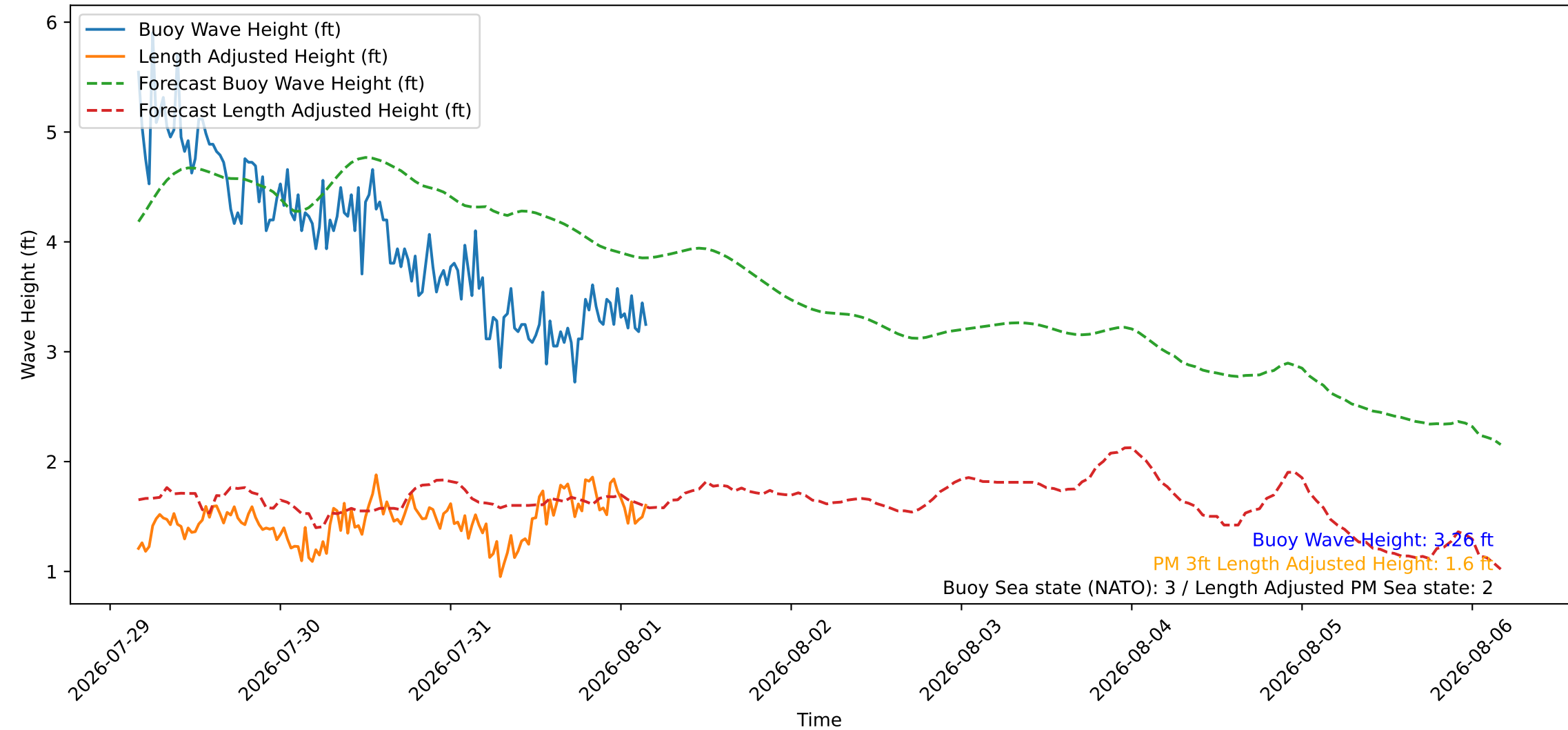
Wave Heights over Time for Oceanside Harbor at 2026-08-01 04:10:26
