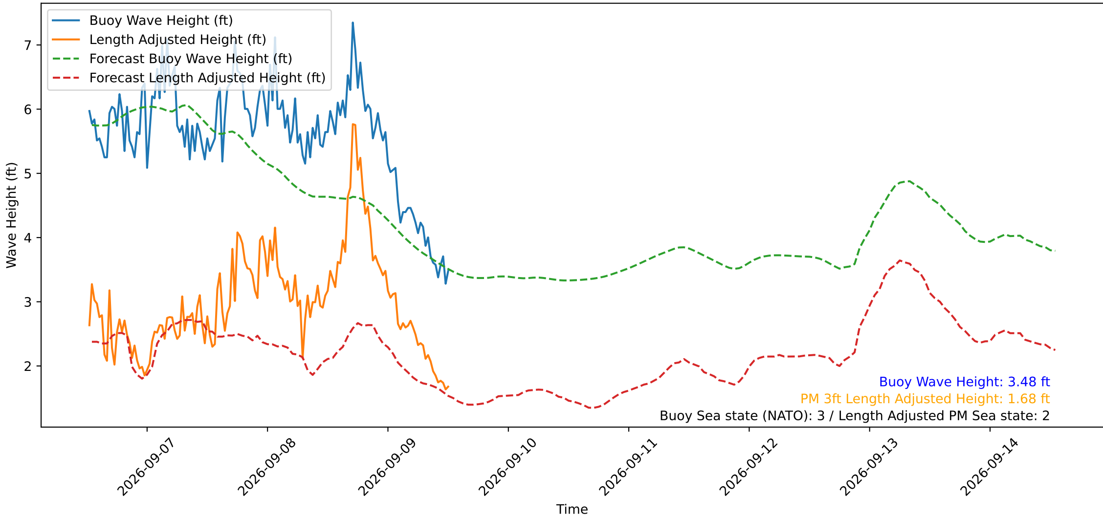
Wave Heights over Time for Oceanside Harbor at 2026-09-09 12:30:29
