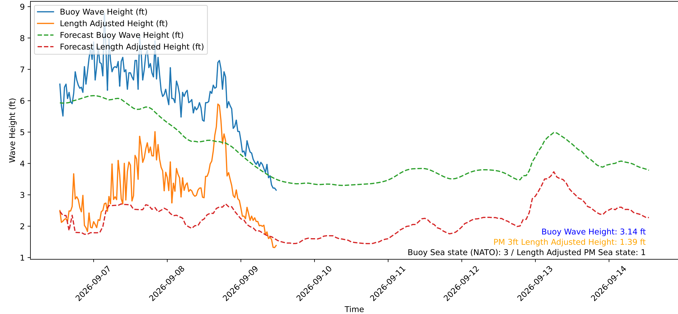
Wave Heights over Time for Green Beach at 2026-09-09 12:31:12
