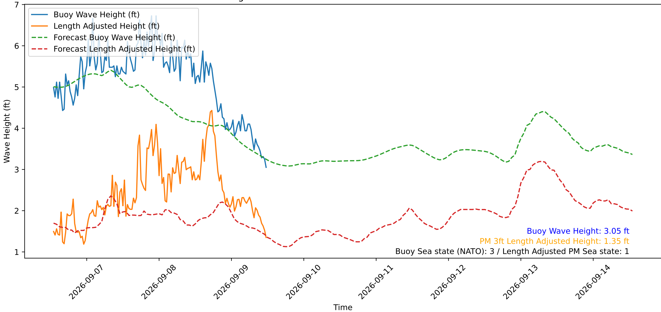
Wave Heights over Time for Red Beach at 2026-09-09 12:30:49
