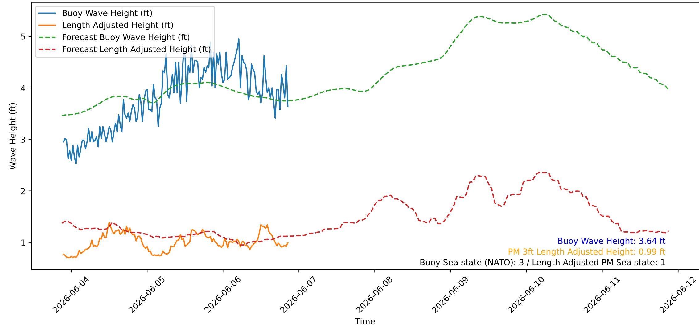
Wave Heights over Time for Red Beach at 2026-06-06 21:20:47
