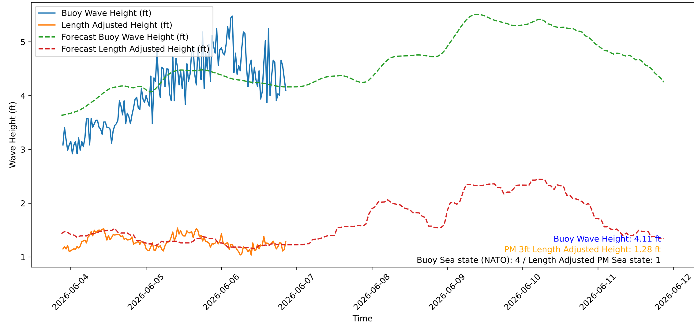
Wave Heights over Time for Oceanside Harbor at 2026-06-06 21:20:26
