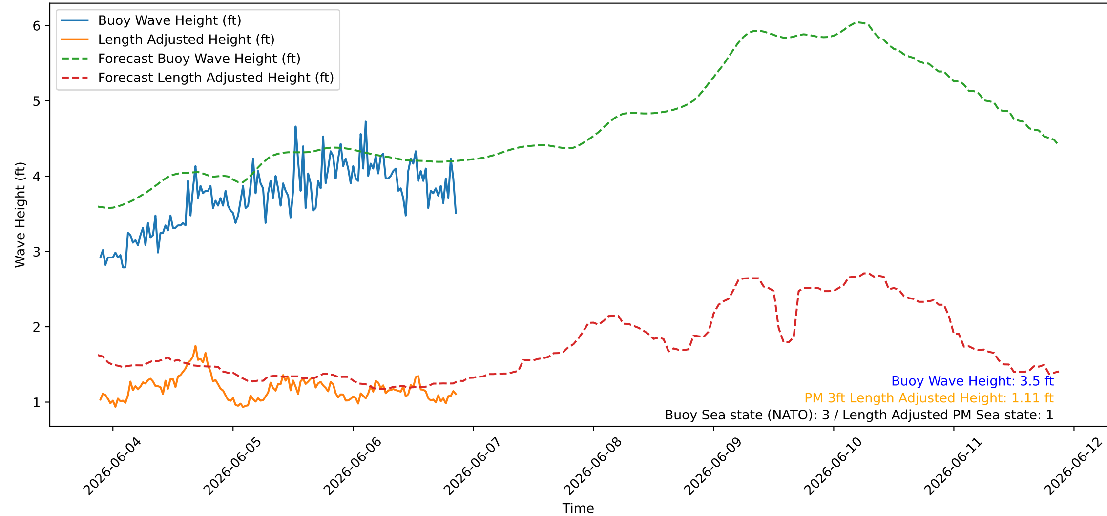
Wave Heights over Time for Green Beach at 2026-06-06 21:21:09
