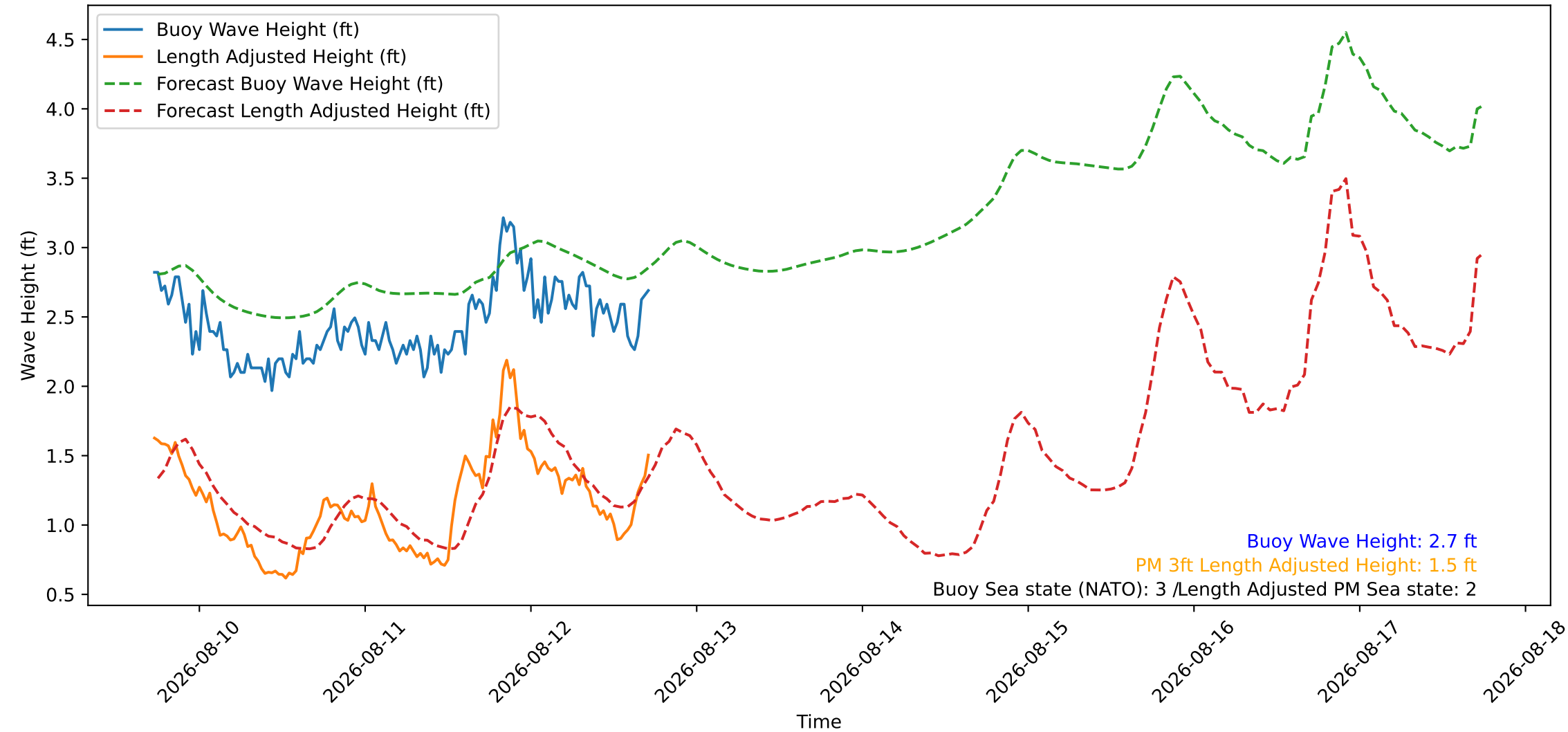
Wave Heights over Time for Green Beach at 2026-08-12 17:41:08
