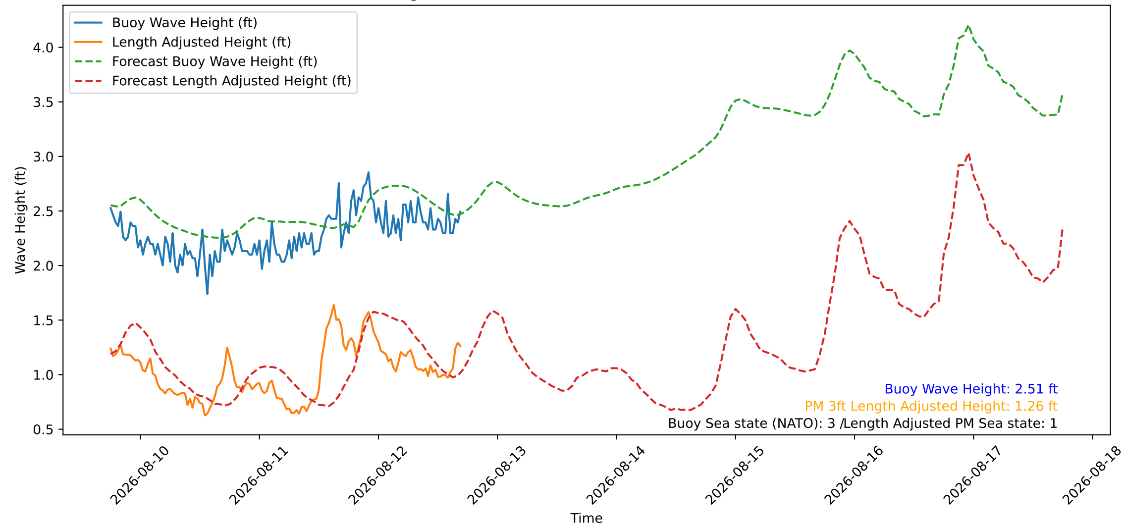
Wave Heights over Time for Red Beach at 2026-08-12 17:40:46
