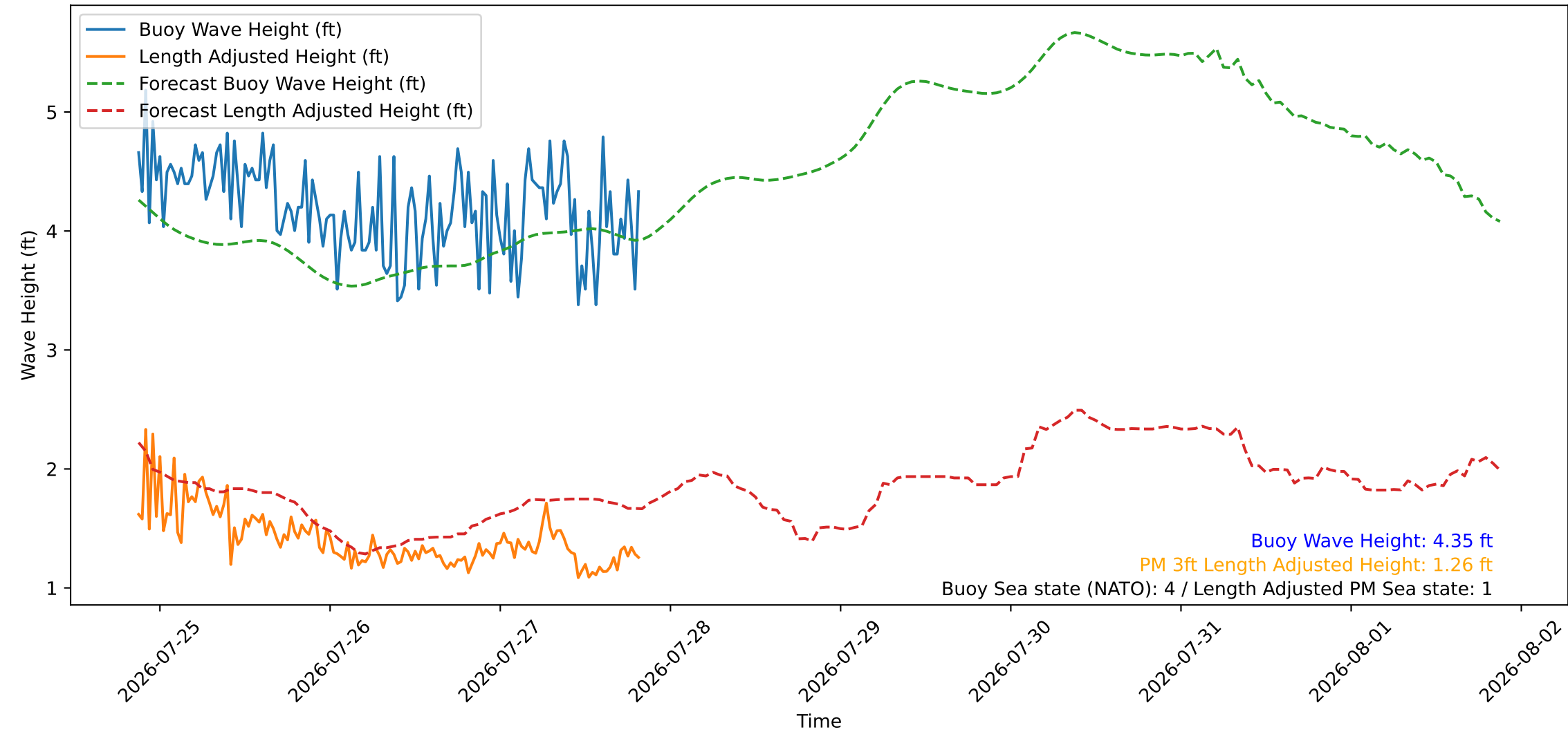
Wave Heights over Time for Green Beach at 2026-07-27 21:01:08
