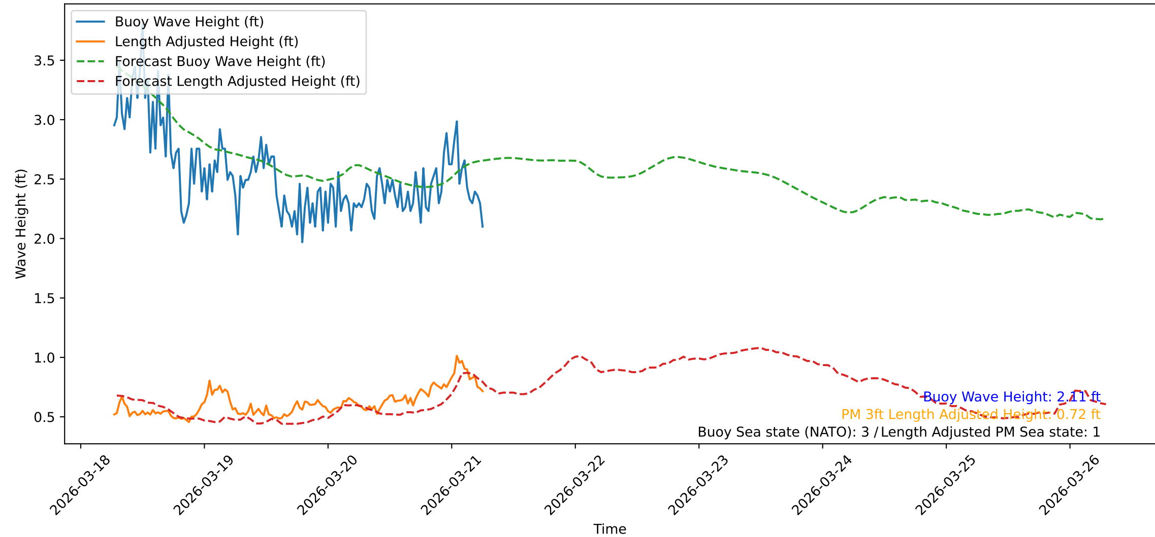
Wave Heights over Time for Oceanside Harbor at 2026-03-21 06:40:31
