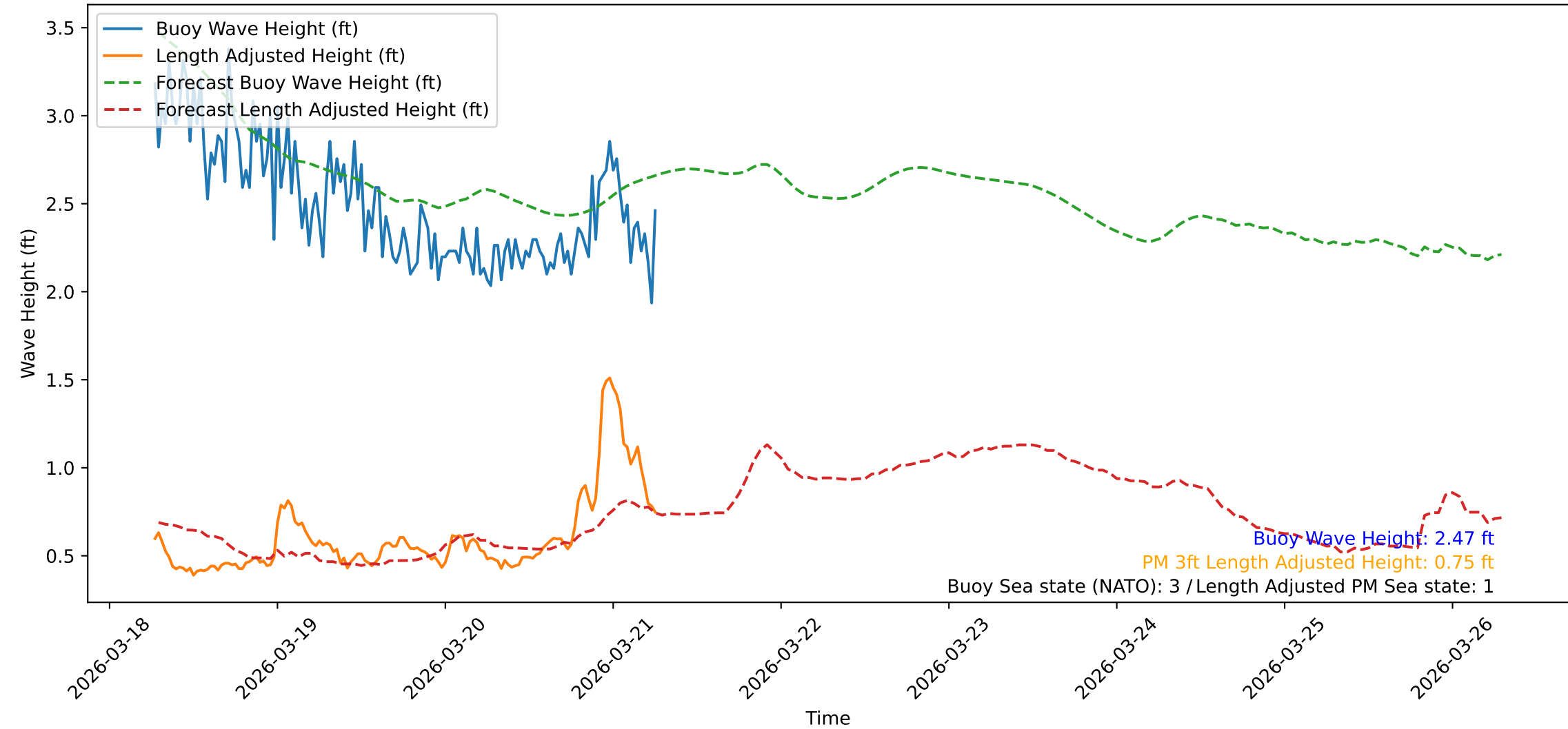
Wave Heights over Time for Green Beach at 2026-03-21 06:41:10
