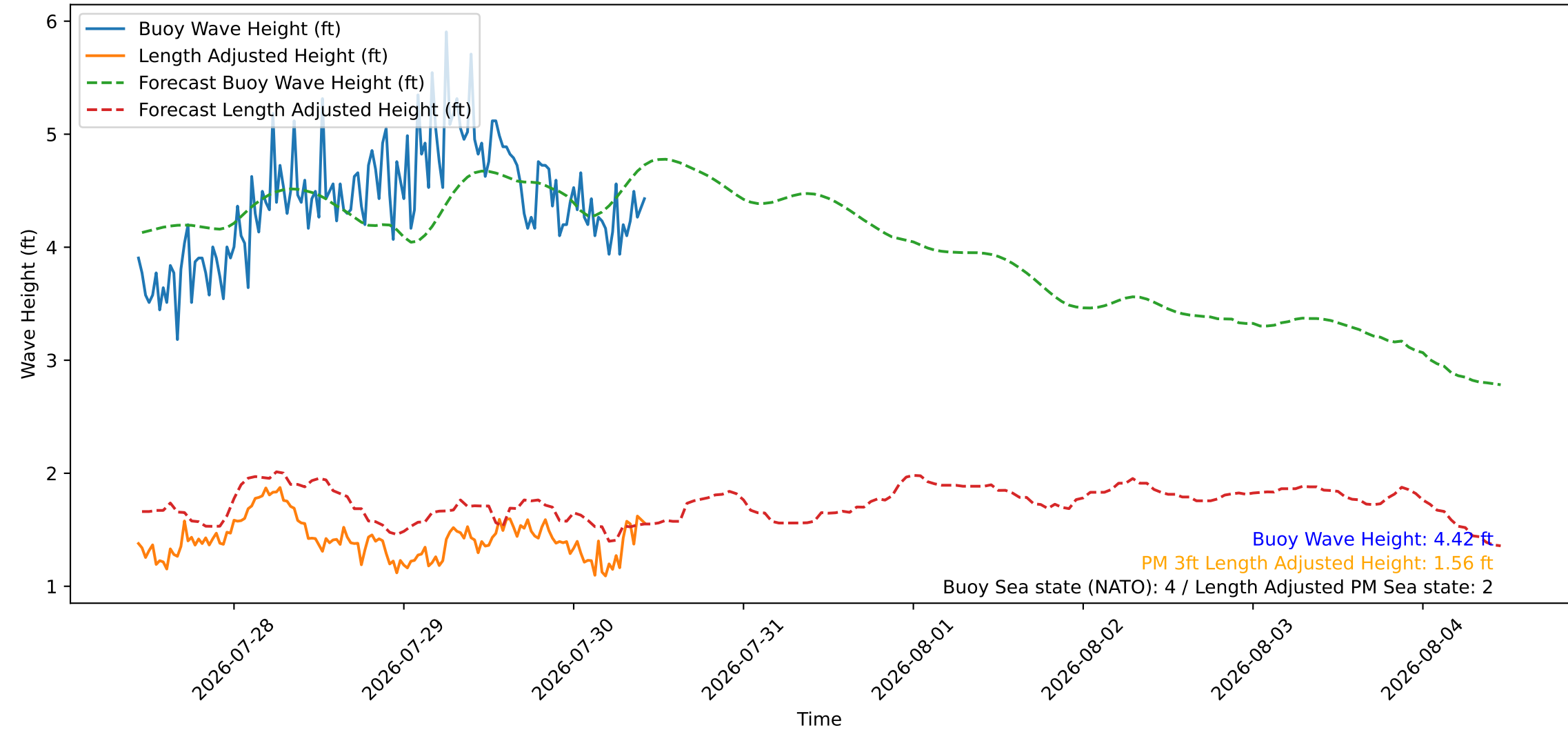
Wave Heights over Time for Oceanside Harbor at 2026-07-30 10:30:26
