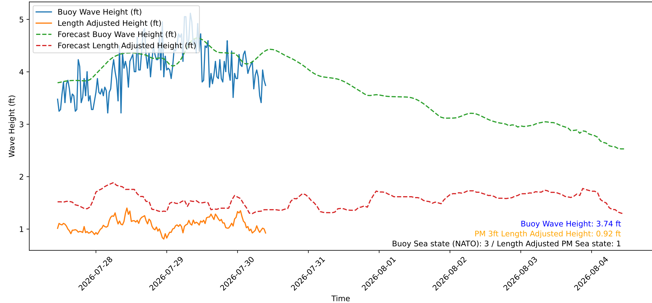
Wave Heights over Time for Red Beach at 2026-07-30 10:30:46
