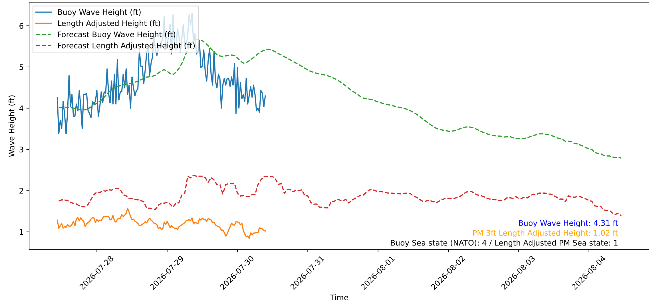
Wave Heights over Time for Green Beach at 2026-07-30 10:31:09
