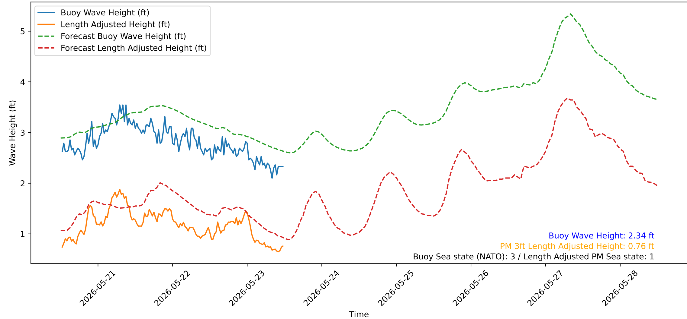
Wave Heights over Time for Green Beach at 2026-05-23 12:21:13
