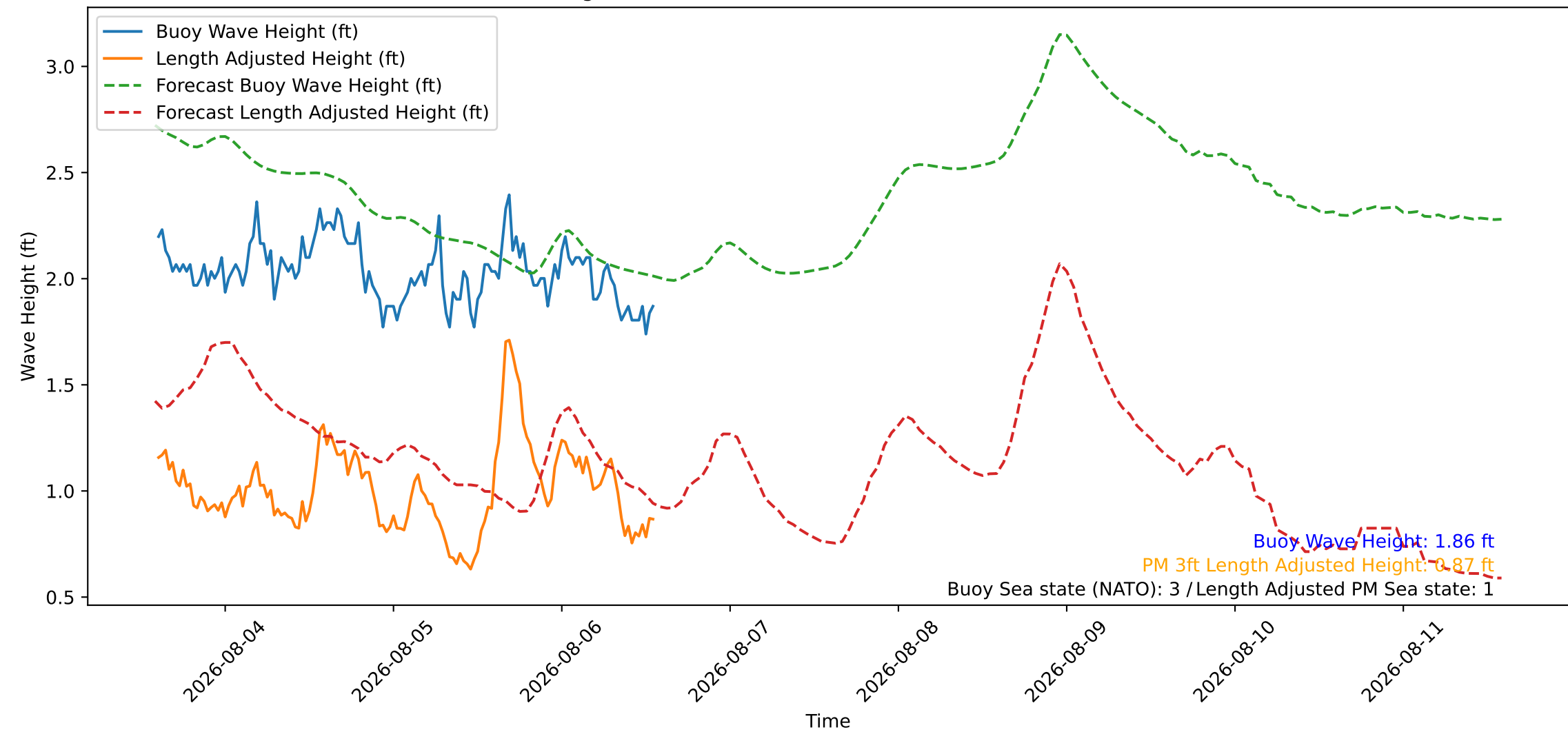
Wave Heights over Time for Red Beach at 2026-08-06 14:00:45
