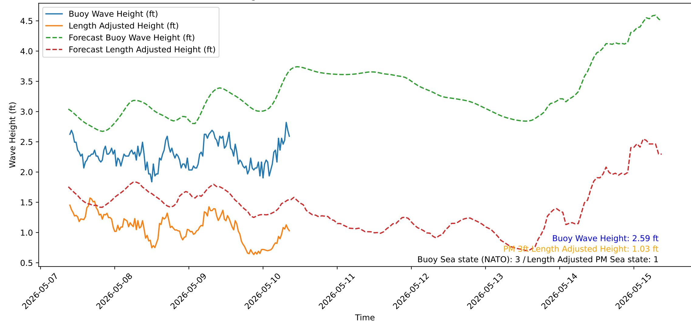
Wave Heights over Time for Green Beach at 2026-05-10 09:21:14
