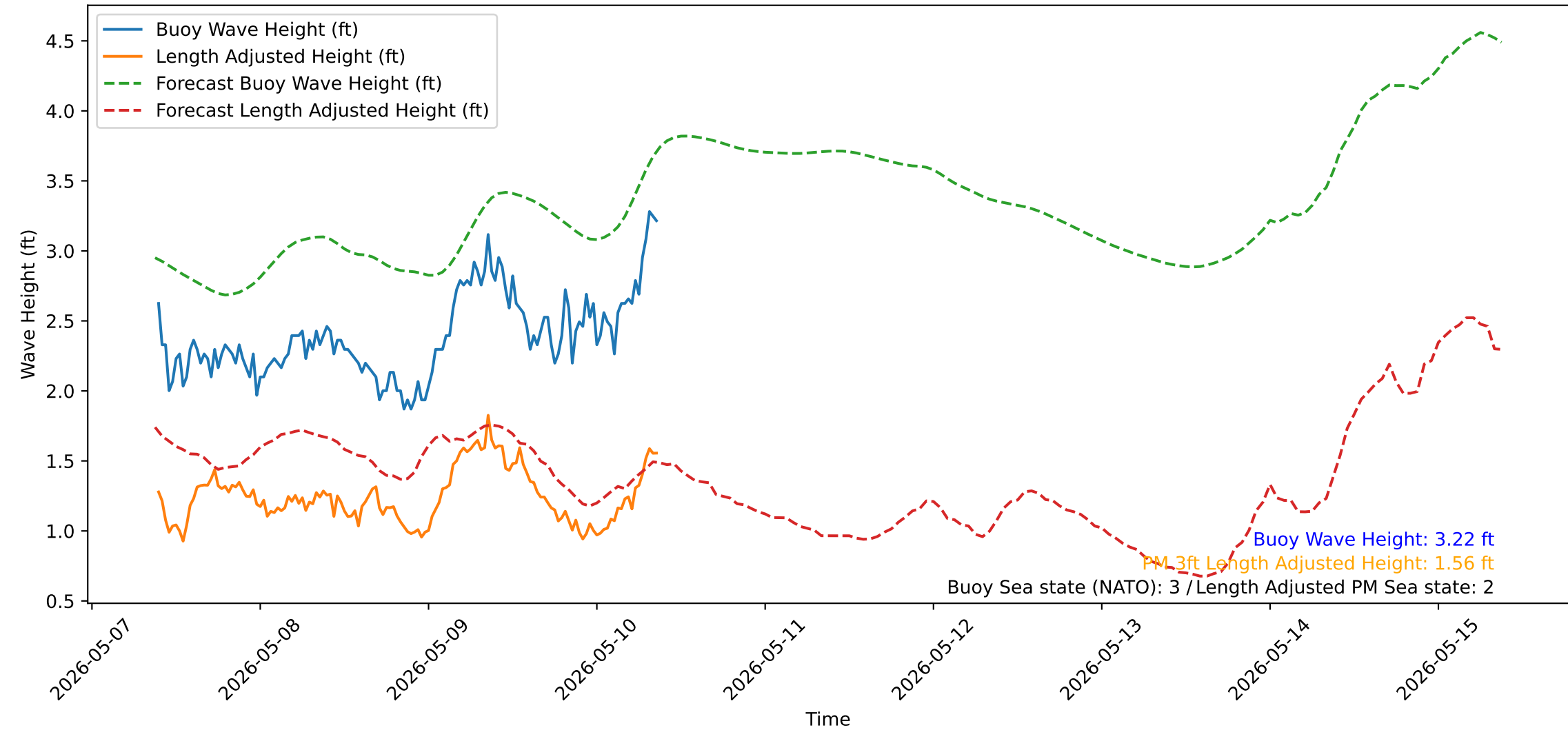
Wave Heights over Time for Oceanside Harbor at 2026-05-10 09:20:31
