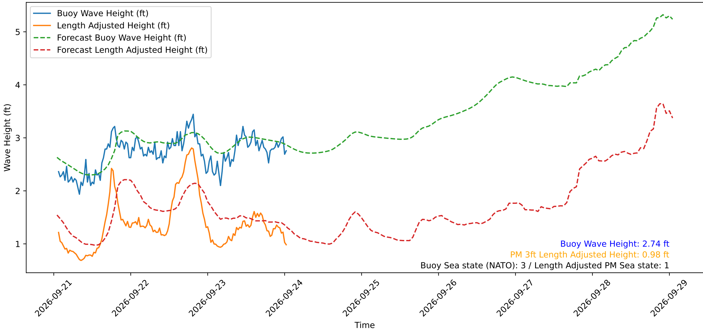
Wave Heights over Time for Green Beach at 2026-09-24 01:21:15
