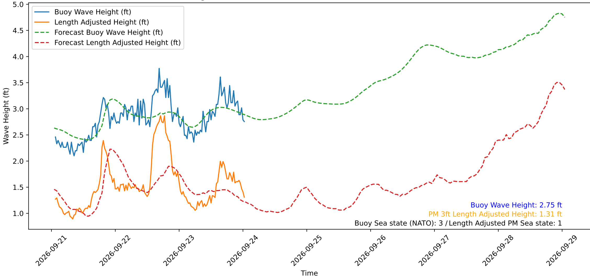
Wave Heights over Time for Oceanside Harbor at 2026-09-24 01:20:30
