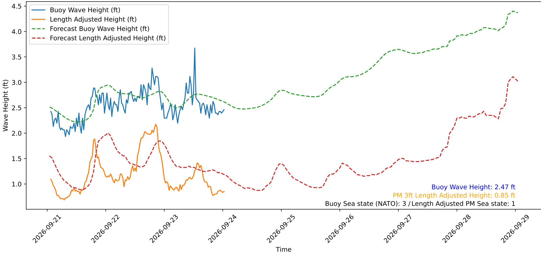
Wave Heights over Time for Red Beach at 2026-09-24 01:20:51
