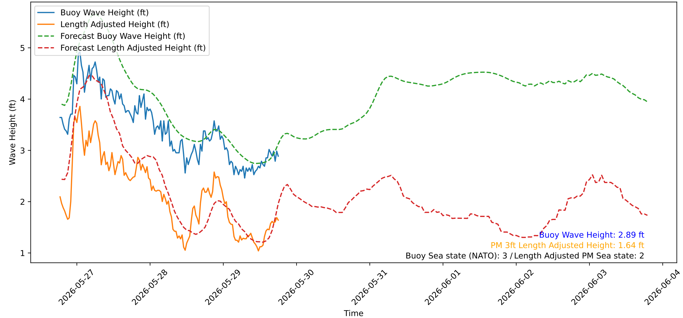
Wave Heights over Time for Green Beach at 2026-05-29 18:41:04
