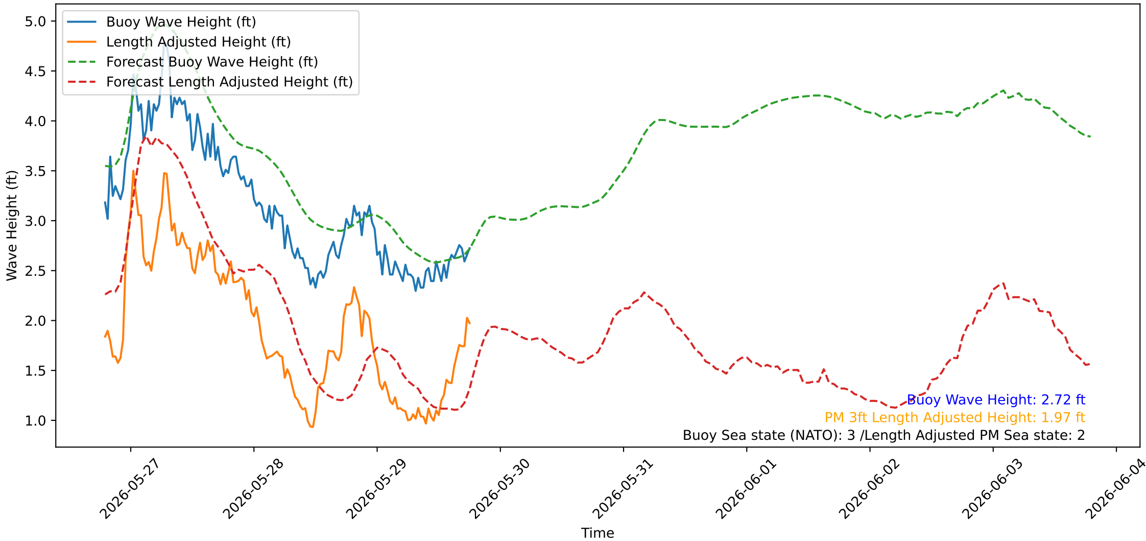
Wave Heights over Time for Red Beach at 2026-05-29 18:40:42
