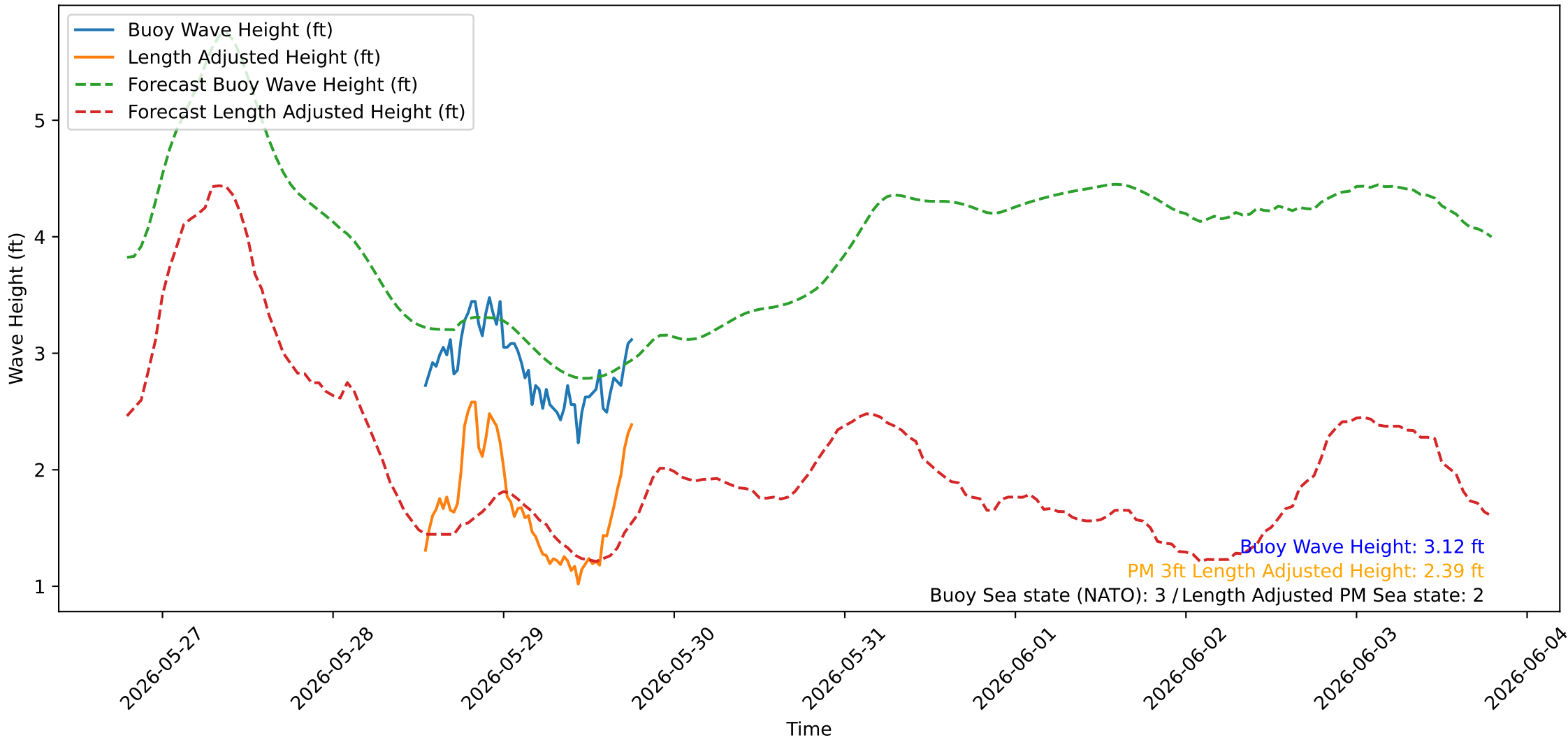
Wave Heights over Time for Oceanside Harbor at 2026-05-29 18:40:22
