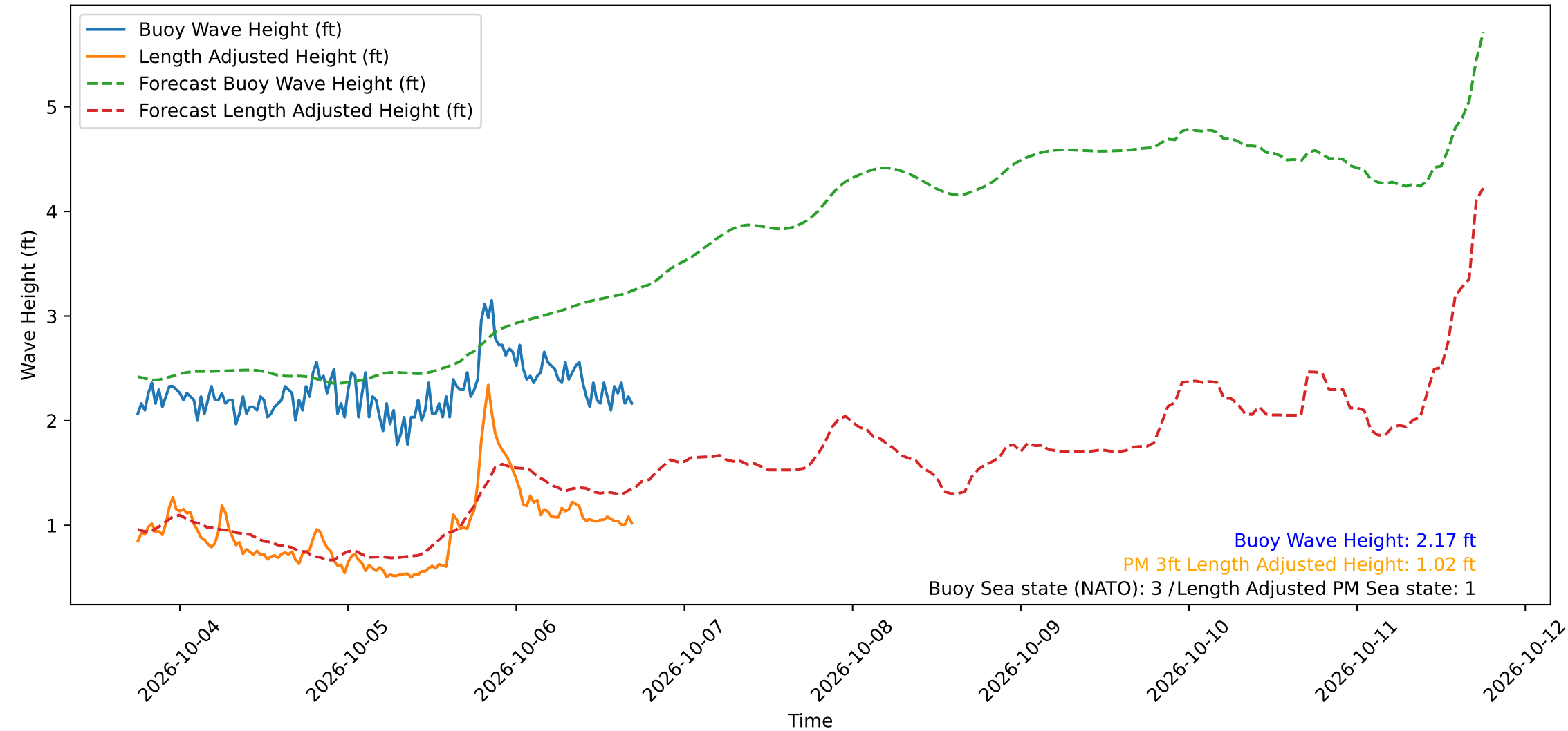
Wave Heights over Time for Green Beach at 2026-10-06 17:31:13
