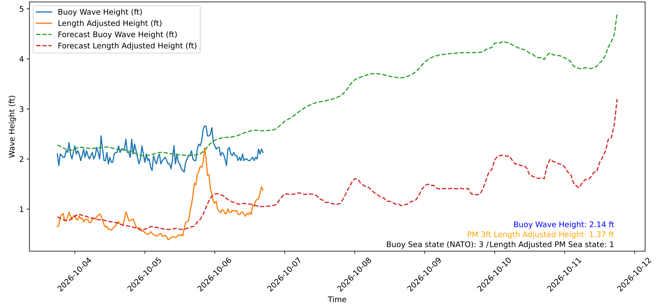
Wave Heights over Time for Red Beach at 2026-10-06 17:30:50
