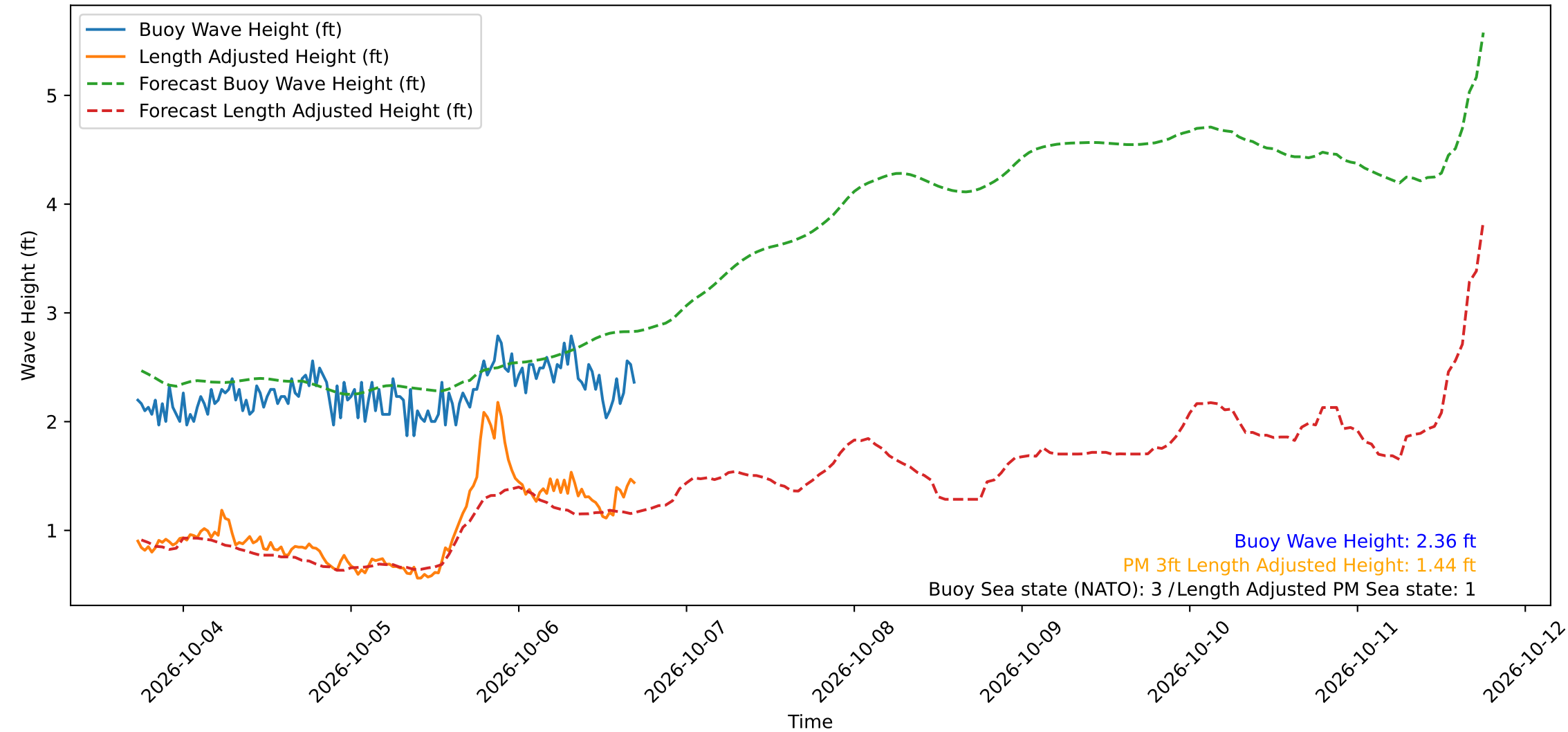
Wave Heights over Time for Oceanside Harbor at 2026-10-06 17:30:30
