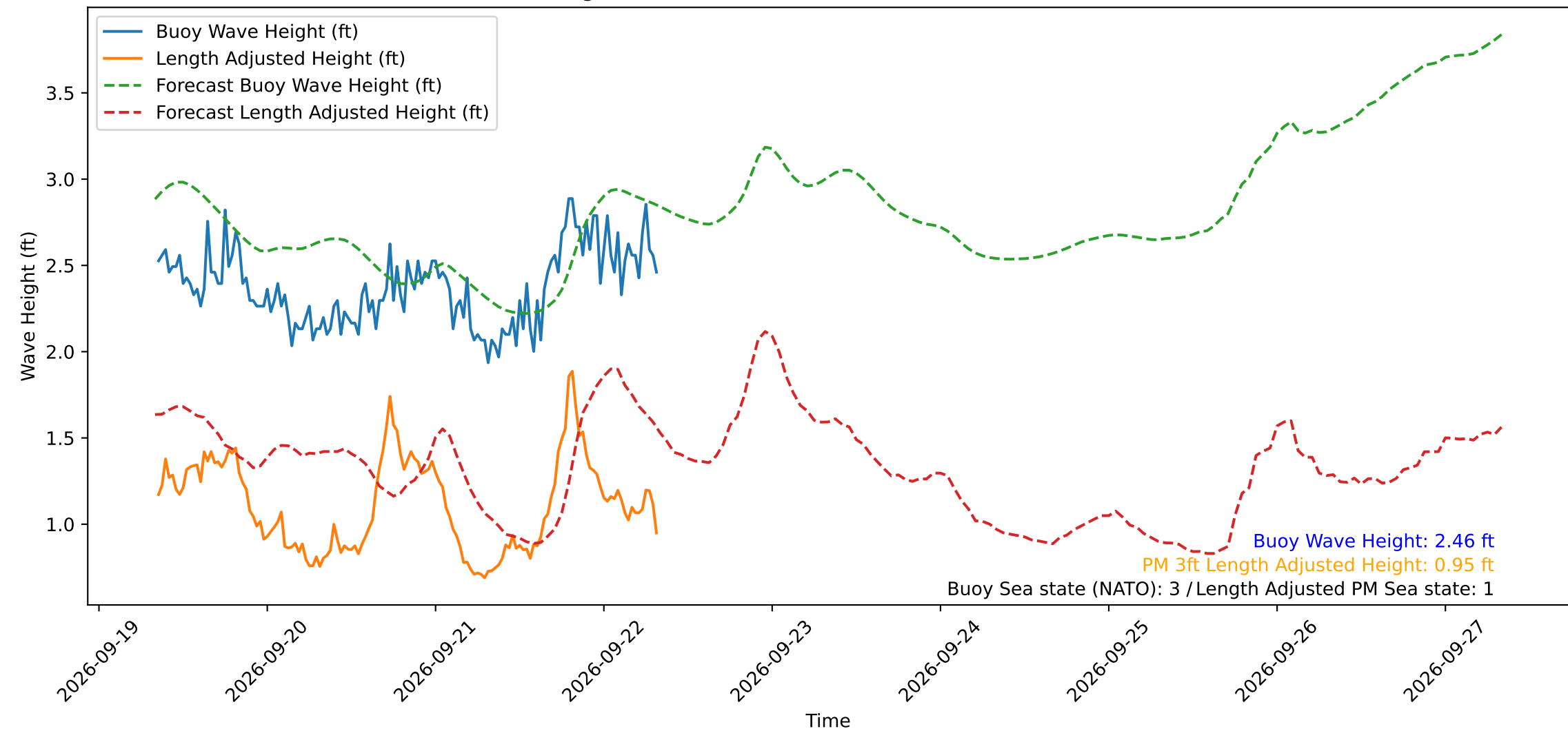
Wave Heights over Time for Red Beach at 2026-09-22 08:20:51
