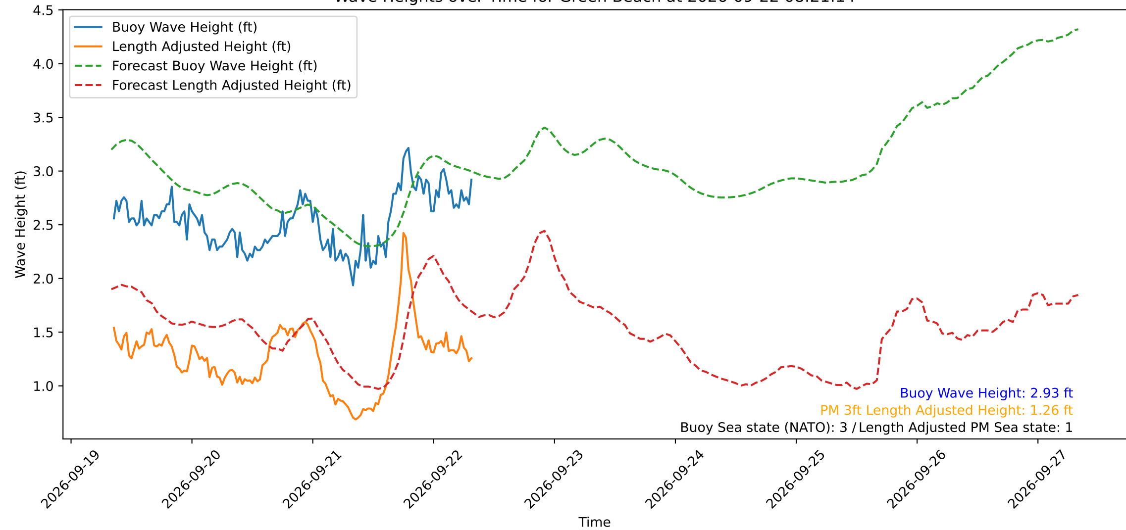
Wave Heights over Time for Green Beach at 2026-09-22 08:21:14
