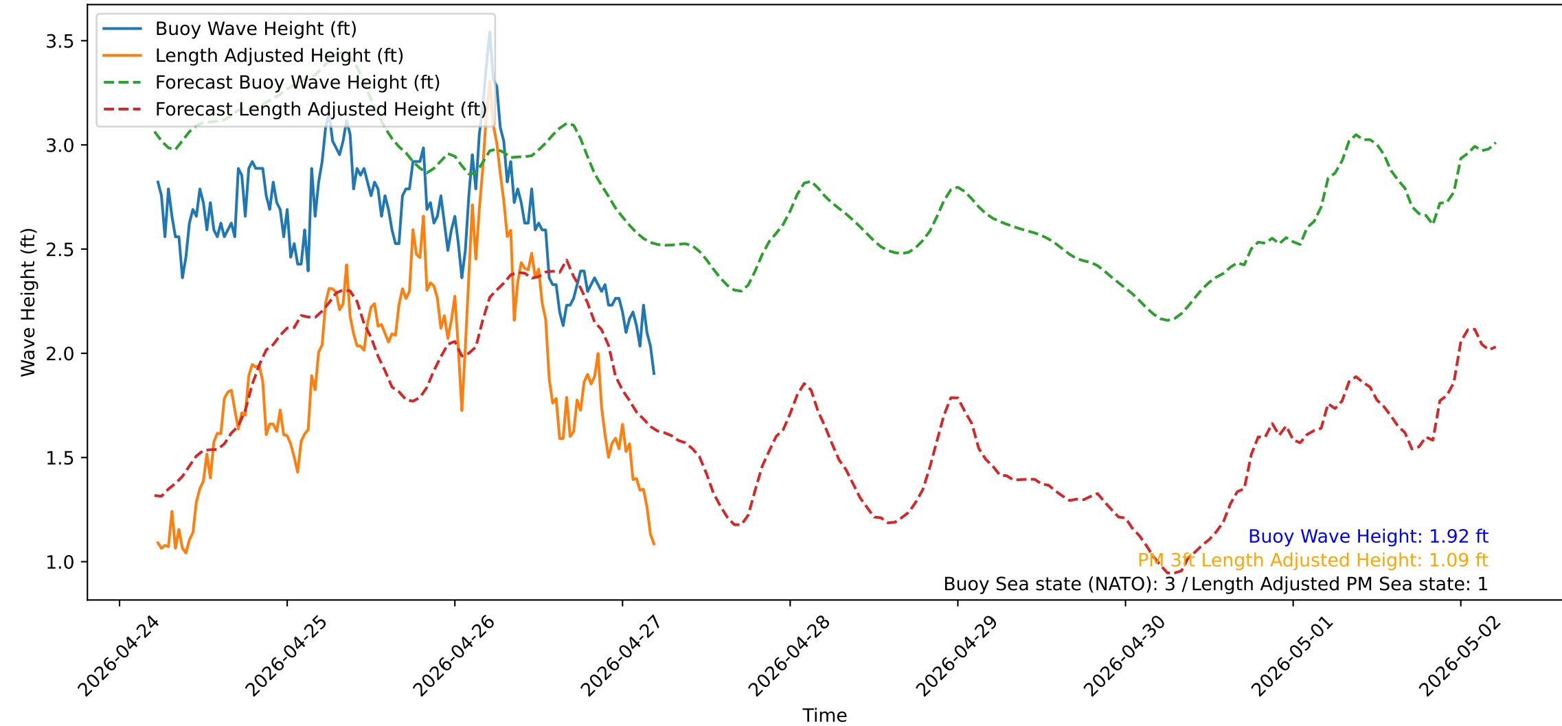
Wave Heights over Time for Red Beach at 2026-04-27 05:10:50
