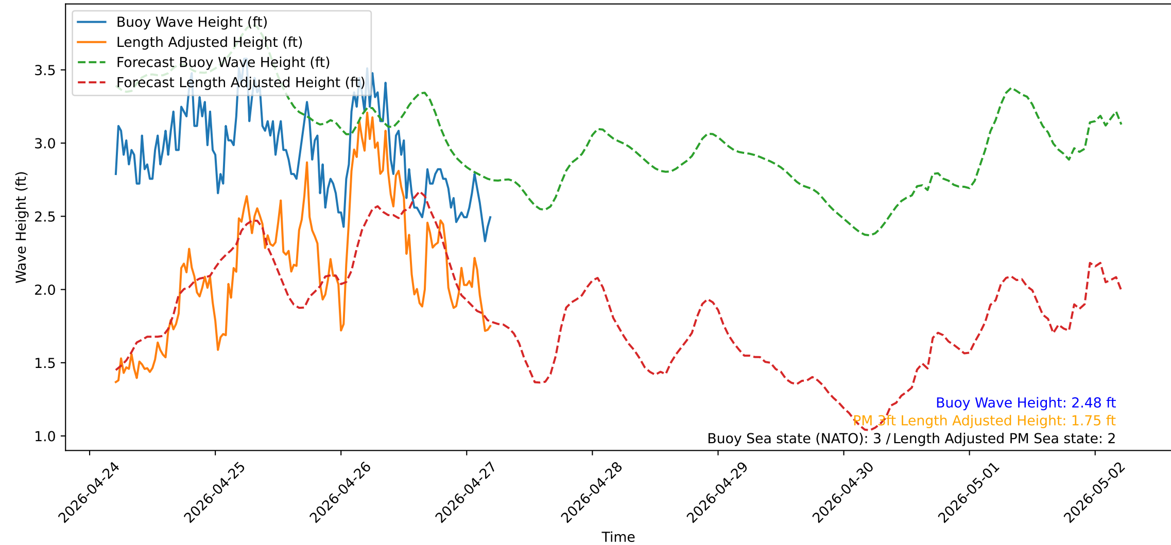
Wave Heights over Time for Green Beach at 2026-04-27 05:11:12
