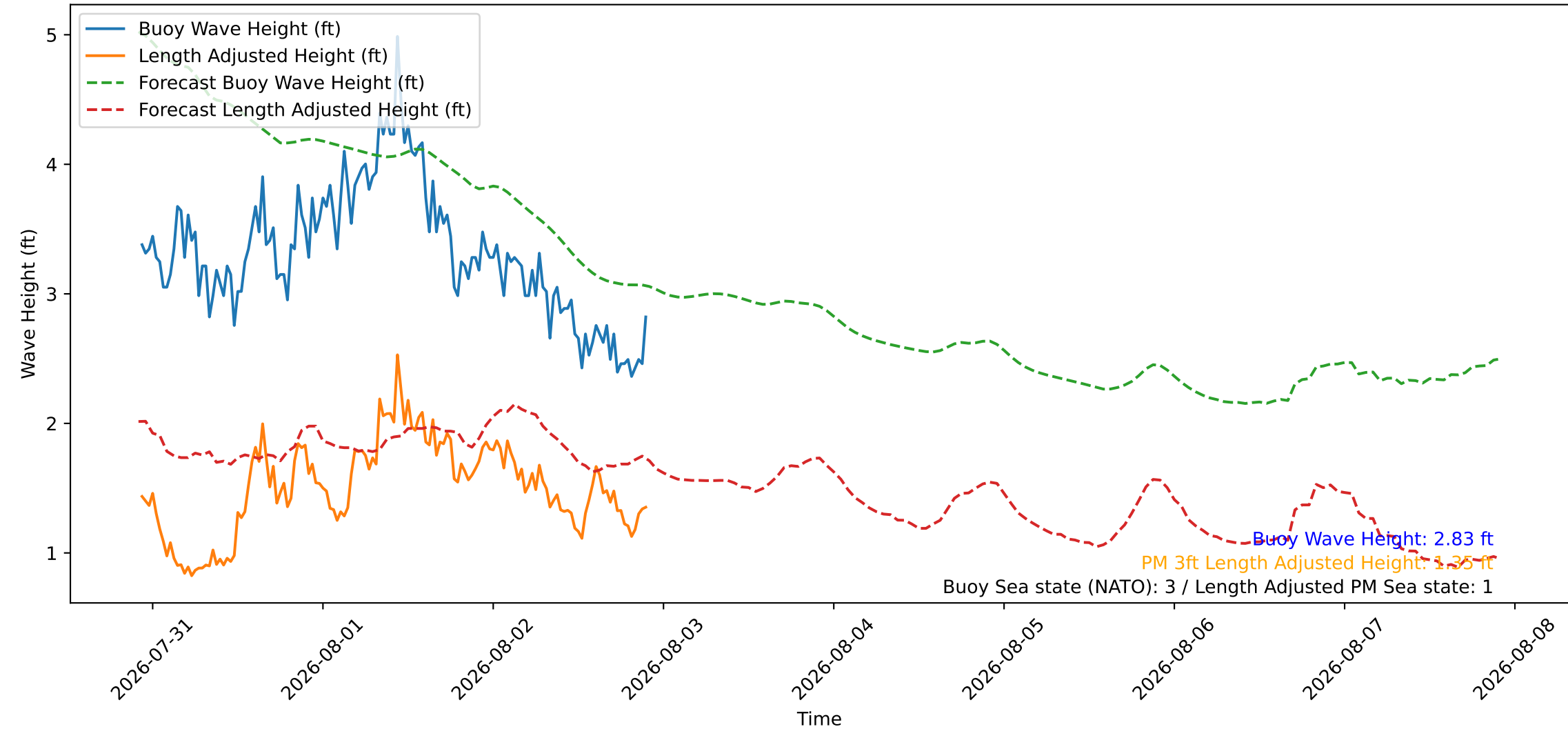
Wave Heights over Time for Green Beach at 2026-08-02 22:21:09
