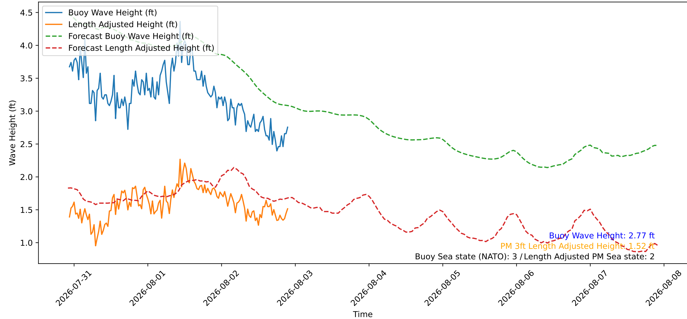
Wave Heights over Time for Oceanside Harbor at 2026-08-02 22:20:26
