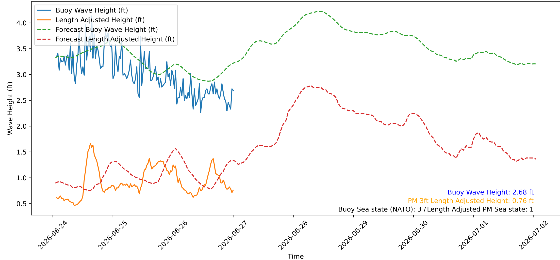
Wave Heights over Time for Red Beach at 2026-06-27 01:00:45
