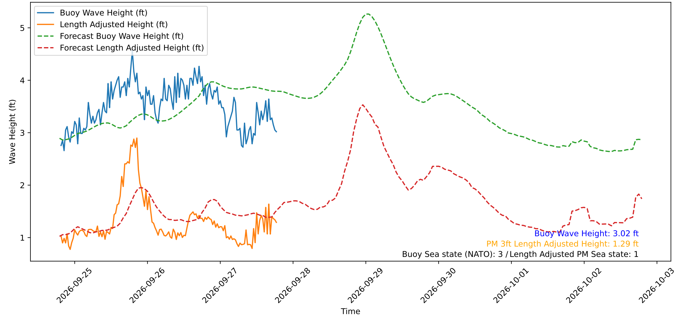
Wave Heights over Time for Green Beach at 2026-09-27 19:11:16
