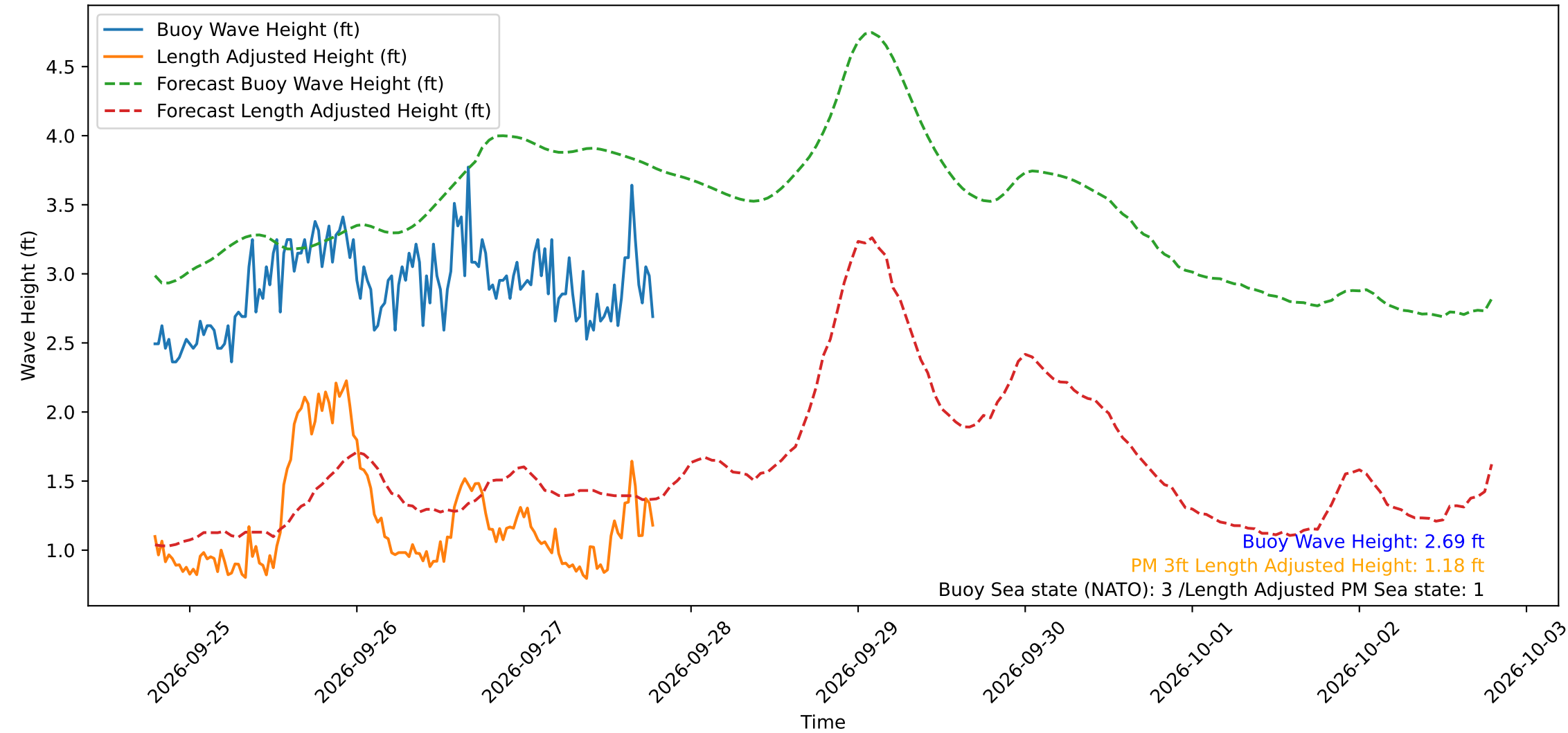
Wave Heights over Time for Oceanside Harbor at 2026-09-27 19:10:31
