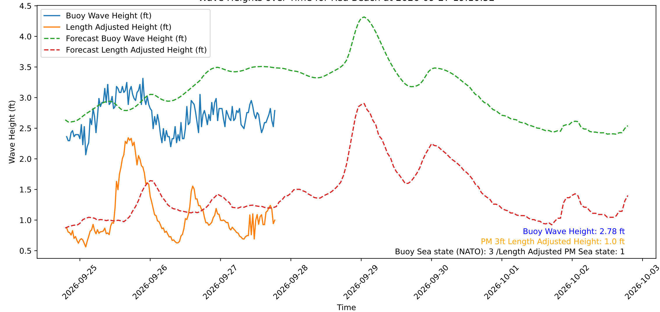
Wave Heights over Time for Red Beach at 2026-09-27 19:10:52
