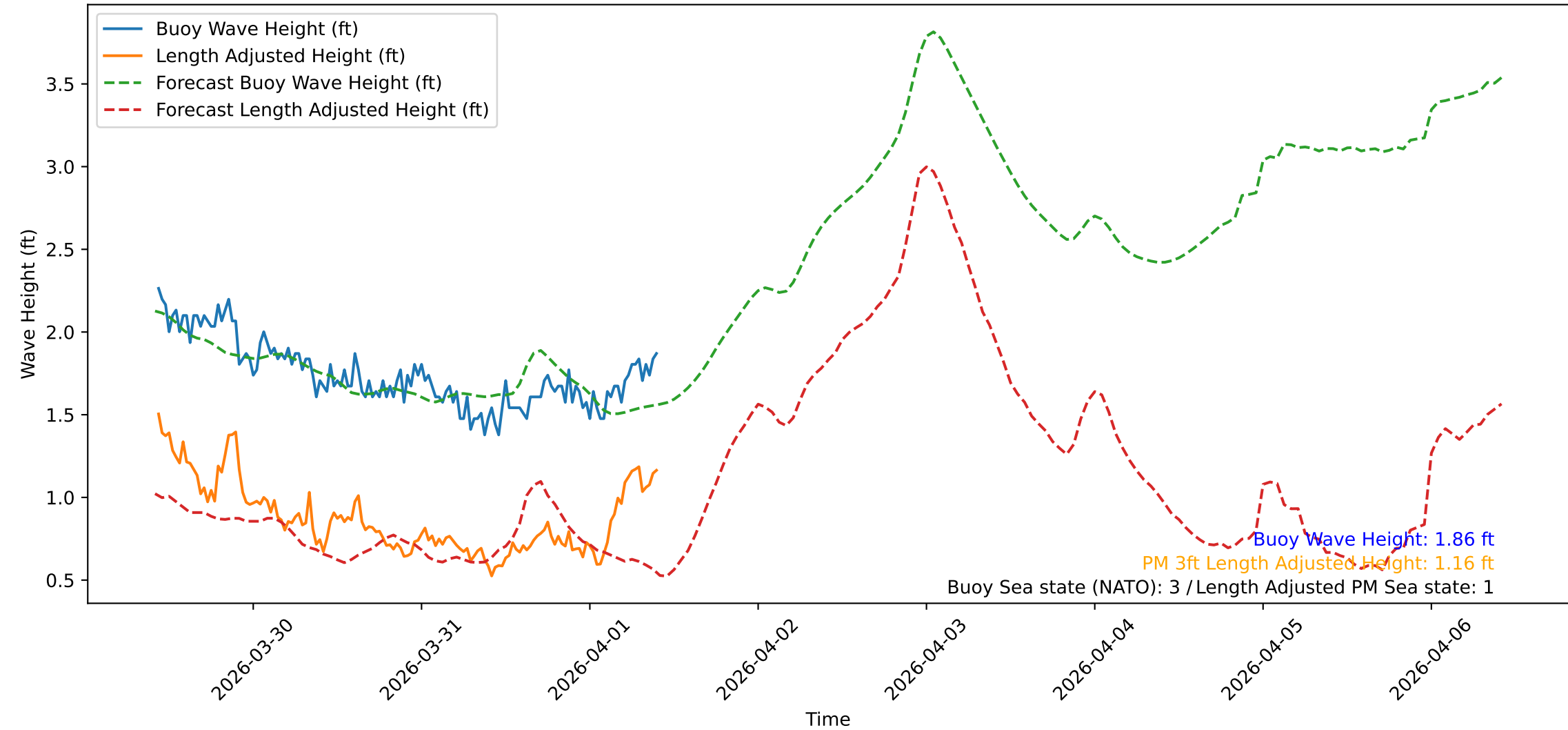
Wave Heights over Time for Red Beach at 2026-04-01 10:10:47
