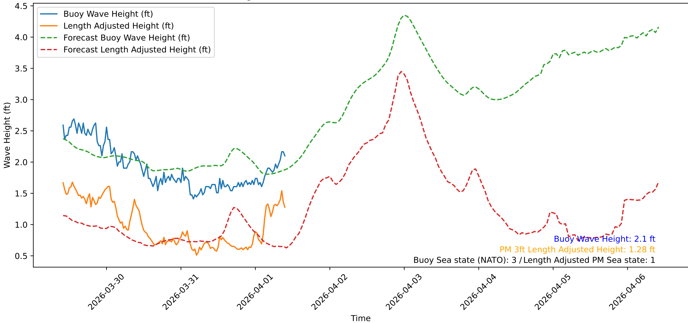
Wave Heights over Time for Green Beach at 2026-04-01 10:11:09
