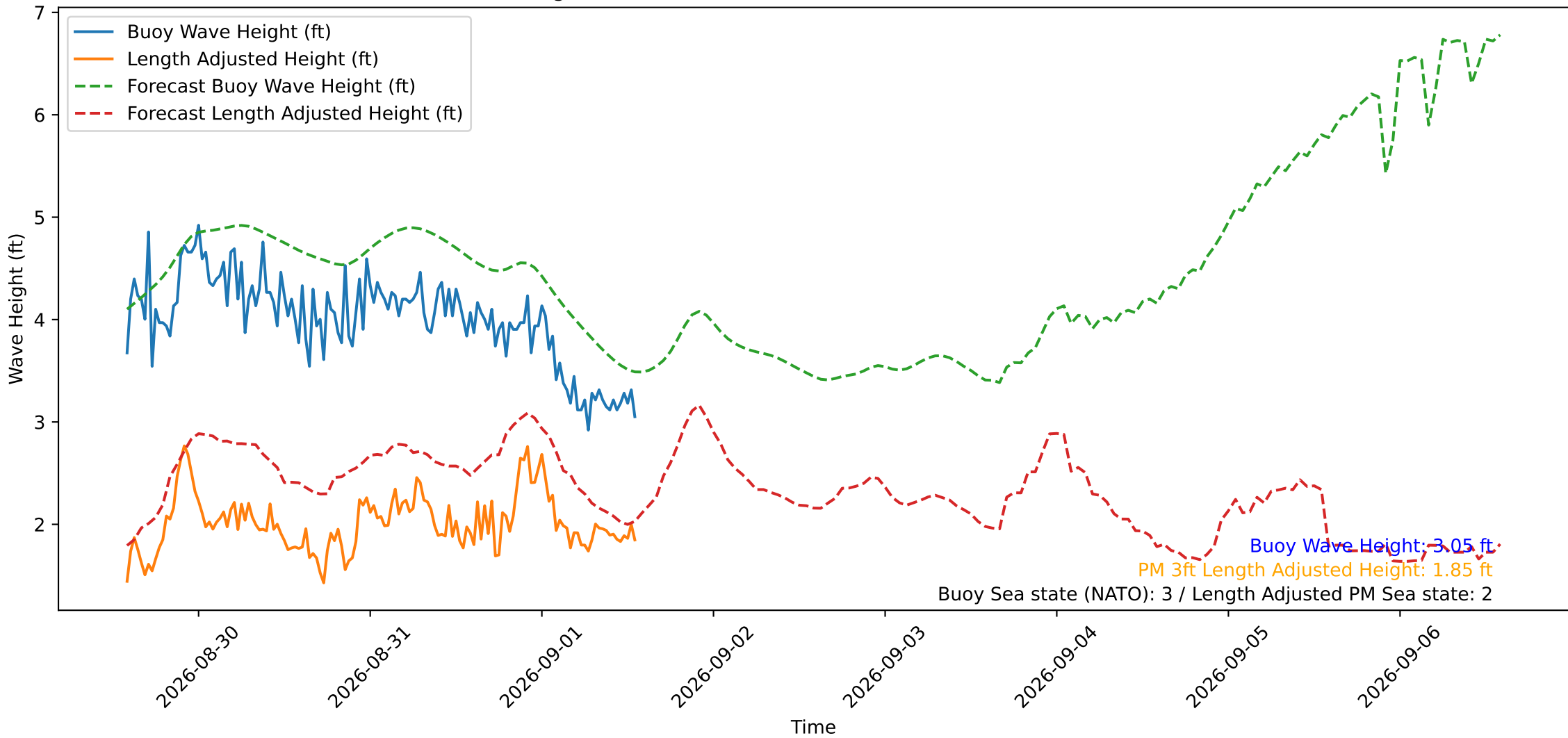
Wave Heights over Time for Green Beach at 2026-09-01 13:41:12
