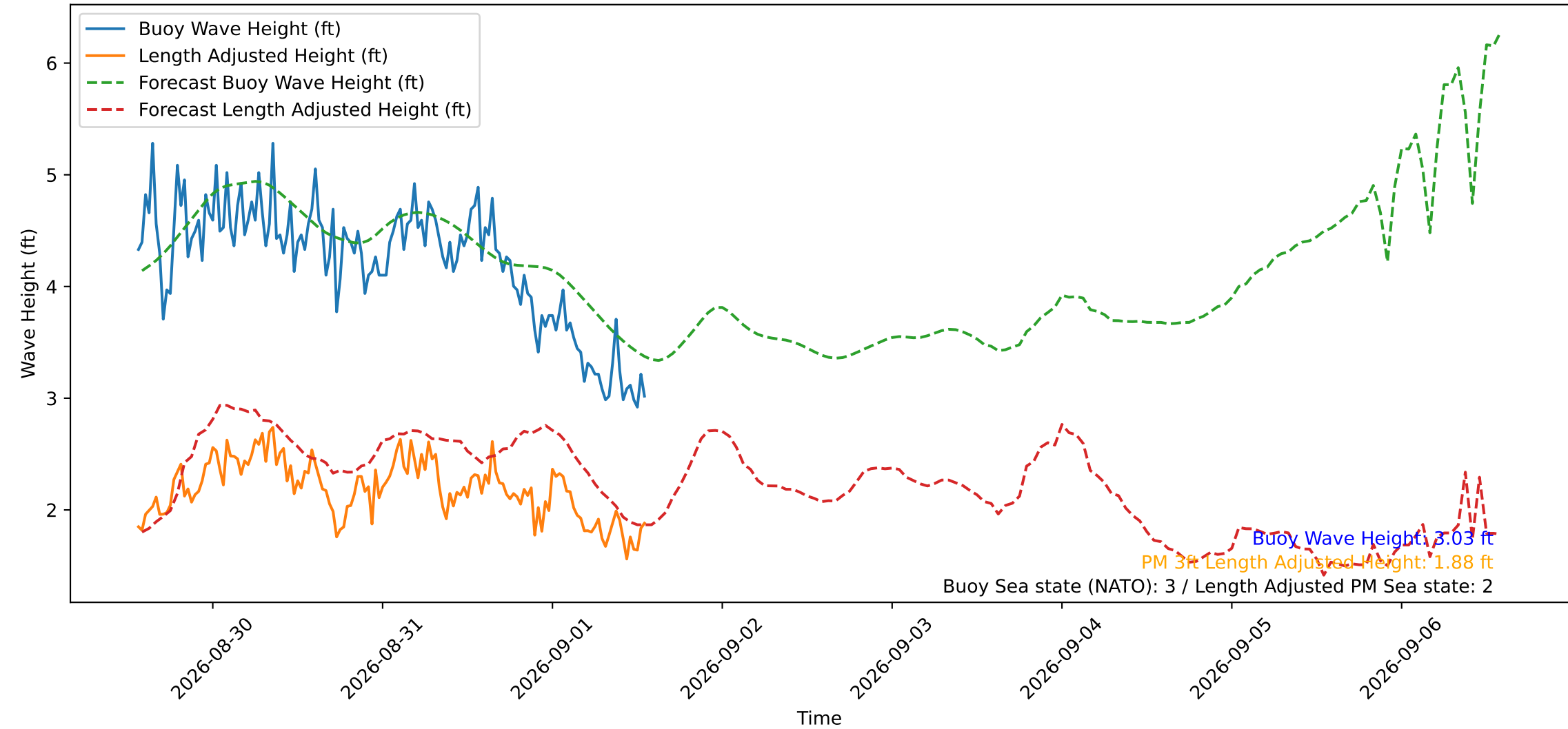
Wave Heights over Time for Oceanside Harbor at 2026-09-01 13:40:29
