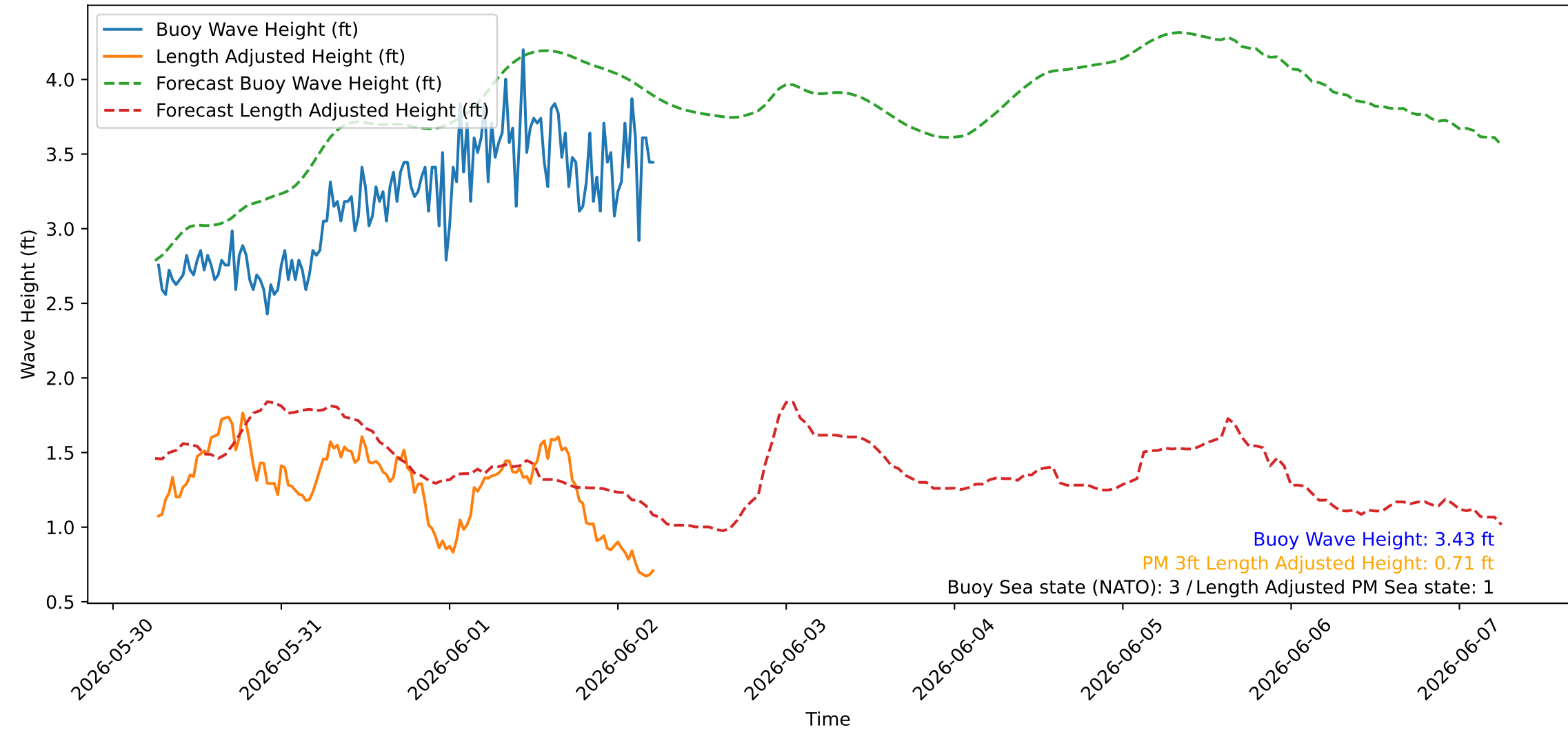
Wave Heights over Time for Red Beach at 2026-06-02 06:00:45
