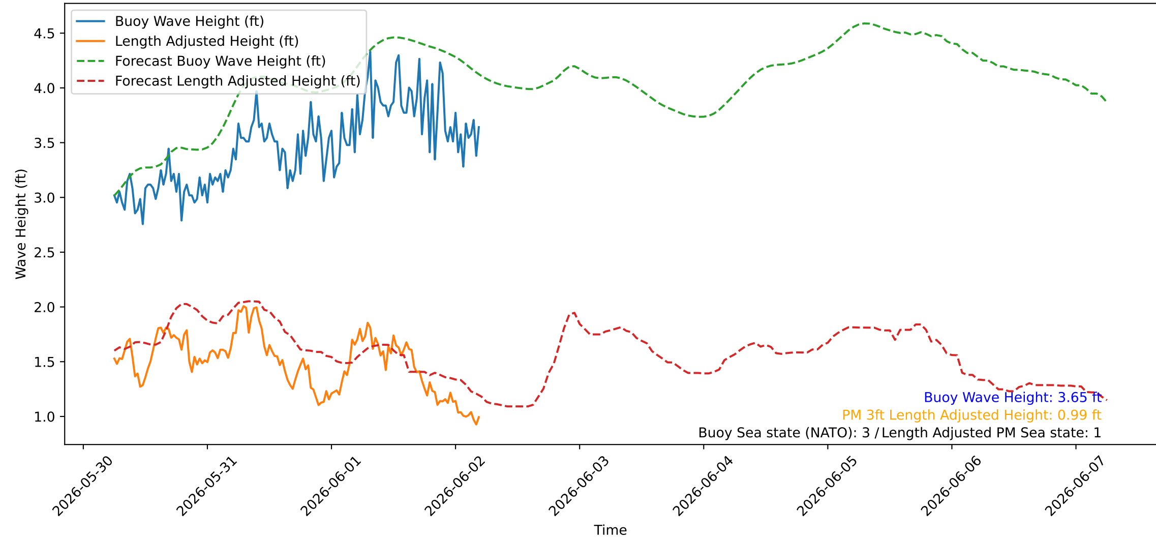
Wave Heights over Time for Green Beach at 2026-06-02 06:01:07
