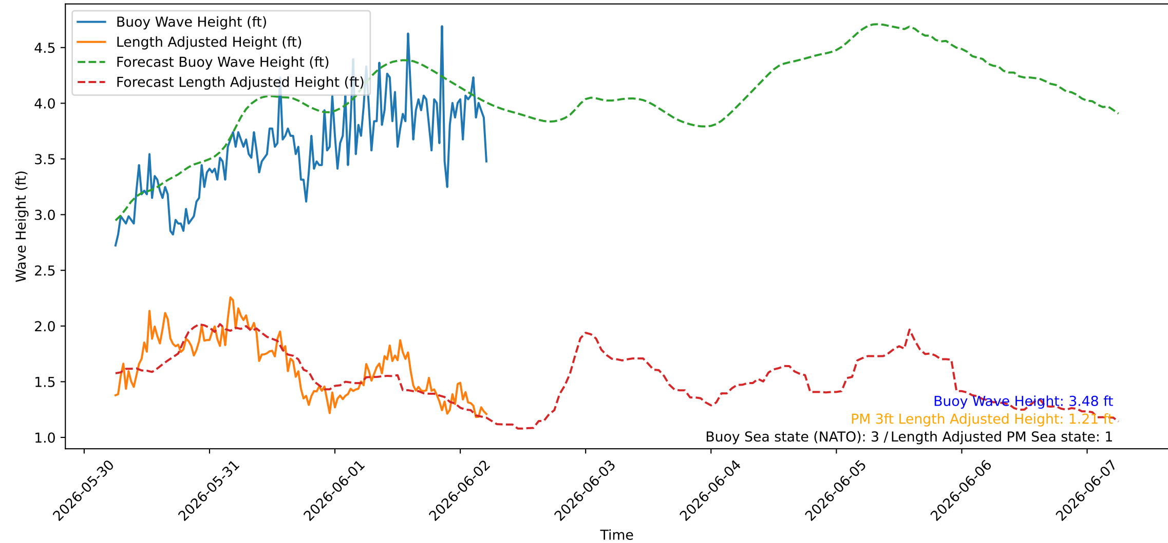
Wave Heights over Time for Oceanside Harbor at 2026-06-02 06:00:26
