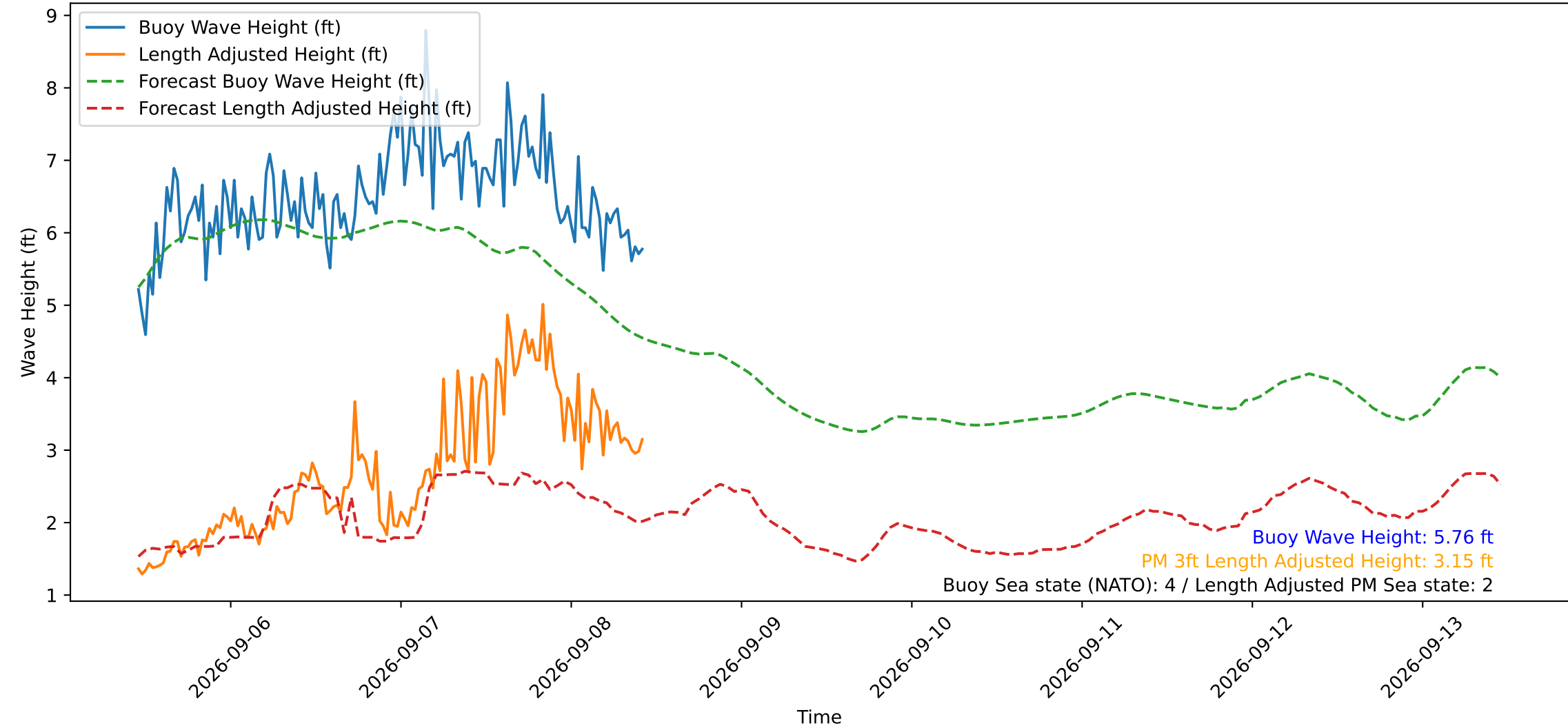
Wave Heights over Time for Green Beach at 2026-09-08 10:41:13
