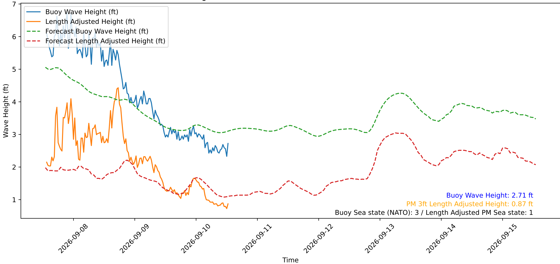
Wave Heights over Time for Red Beach at 2026-09-10 13:20:50
