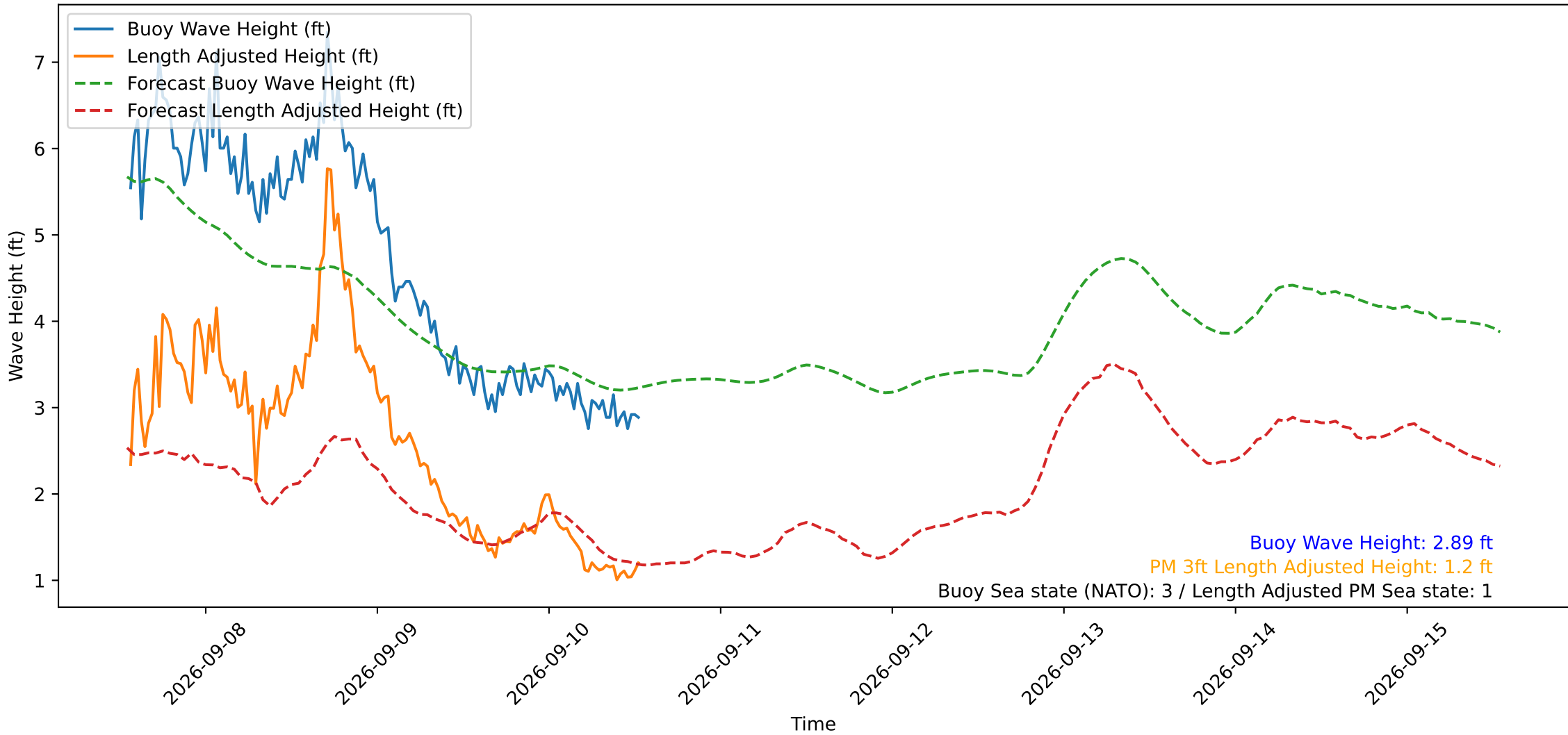
Wave Heights over Time for Oceanside Harbor at 2026-09-10 13:20:29
