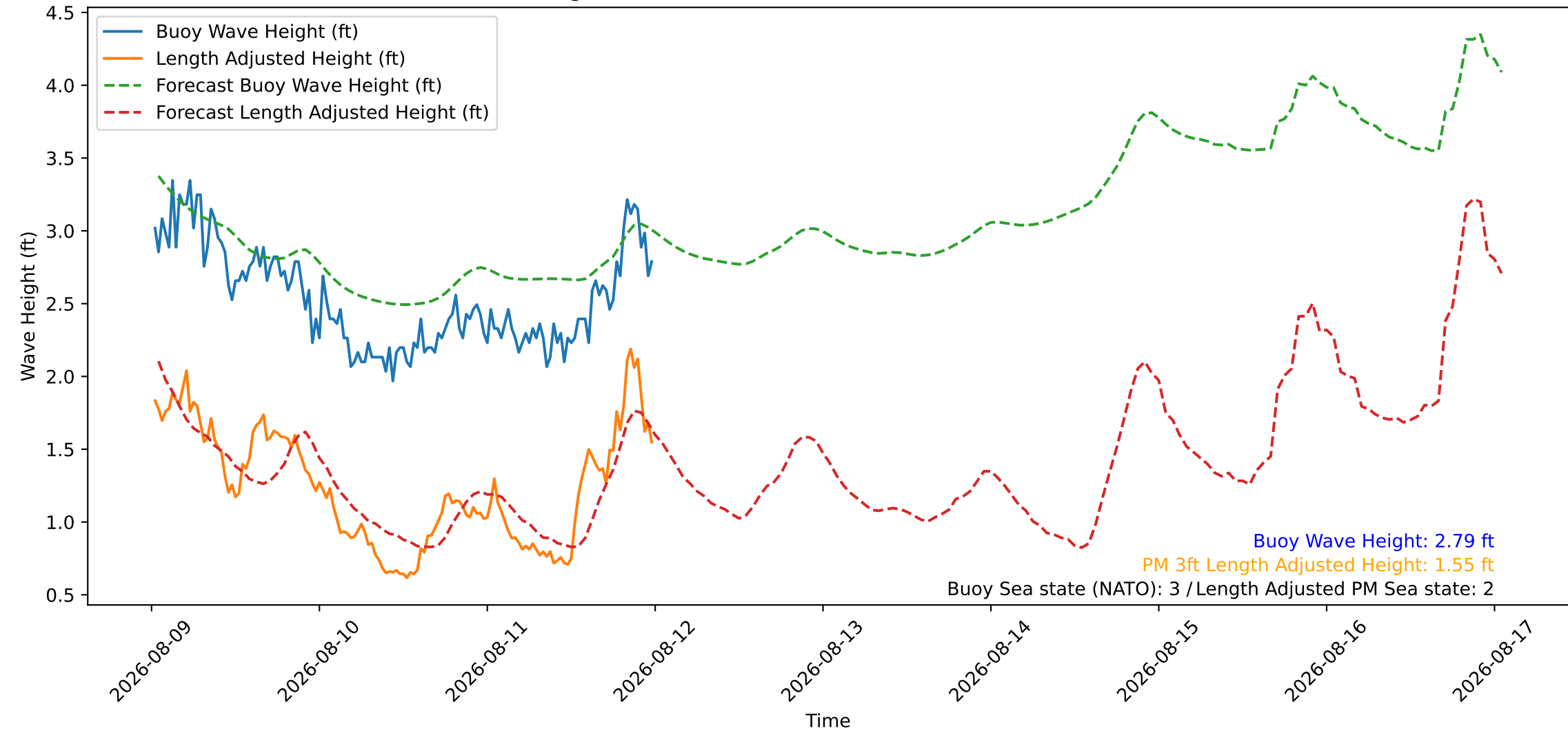
Wave Heights over Time for Green Beach at 2026-08-12 00:31:08
